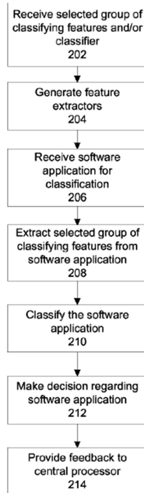
Fig. 2 (Classification)
