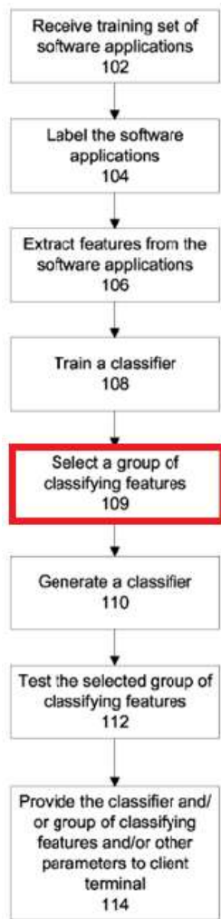
Fig. 1 (Training)
