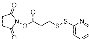
N-succinimidyl-3-(2-pyridyldithio)propionate (SPDP),
