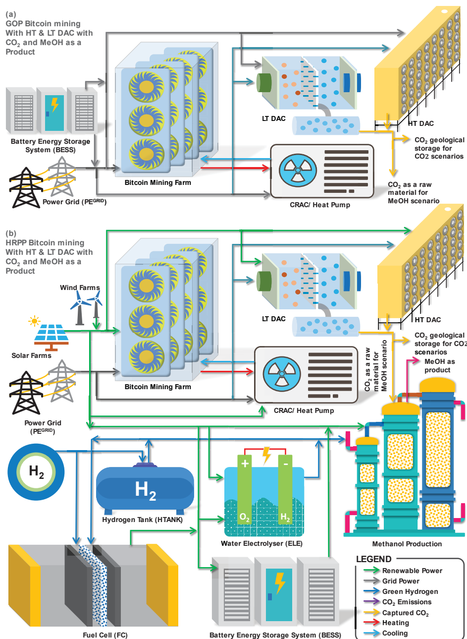
Figure 2. (a) GOP bitcoin mining with high-temperature (HT) and low-temperature (LT) direct air capture (DAC) with CO 2 capture and storage and MeOH as products, (b) HRPP mining with HT- and LT-DAC and CO 2 capture and storage and MeOH as products.
