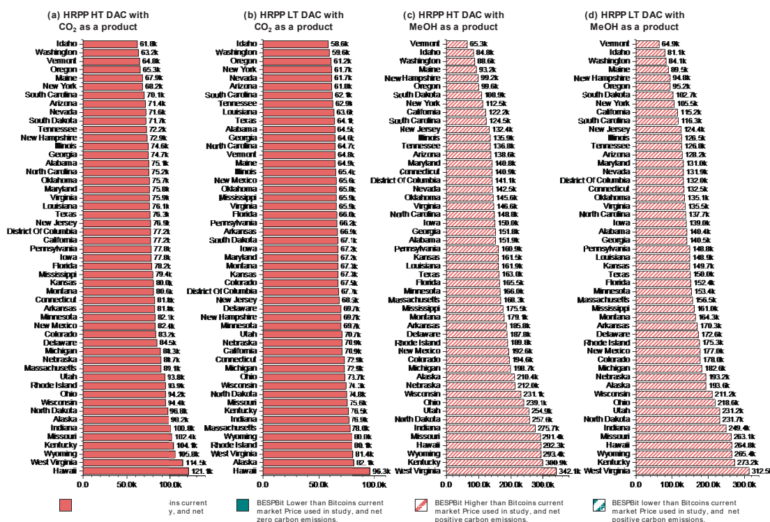
Figure 10. Best and worst states from the BESPBt perspective for the HRPP case.
