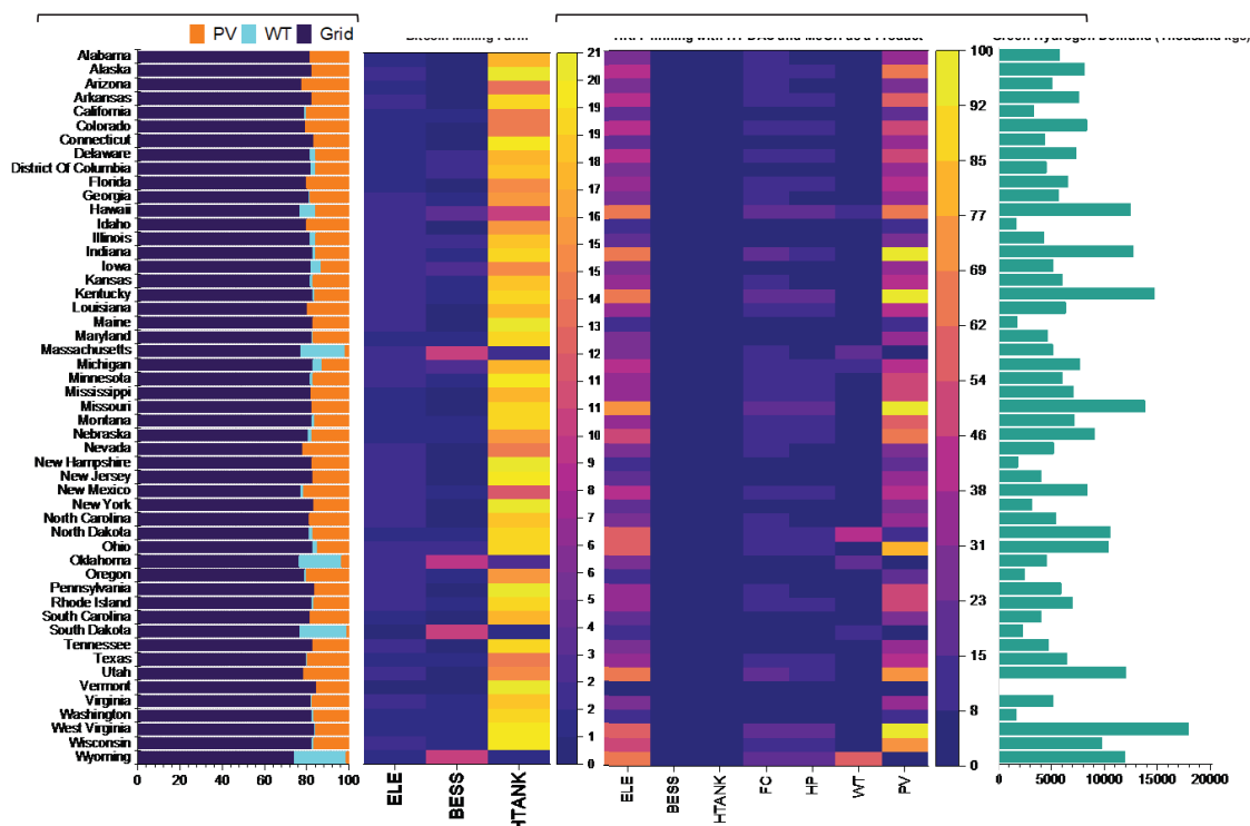
Figure 8. US state-wise PV, WT, and grid resource mix, the optimal numbers of BESS, WTs, and PVs required to power the bitcoin mining farm, and the optimal numbers of ELE, BESS, HTANKs, FCs, HPs, WTs, PVs, and hydrogen required to power the HT-DAC plant for the HRPP case with MeOH as a product. The BESS, PVs, ELE, FCs, and HPs all have a 1.0 MW rating, whereas the WTs and HTANKs have a 1.5 MW and 10 kg rating.
