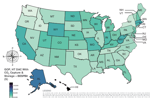
Figure 4. Break-even selling price of bitcoin (BESPBit) for HT-DAC with CO 2 capture and storage using GOP mining.
