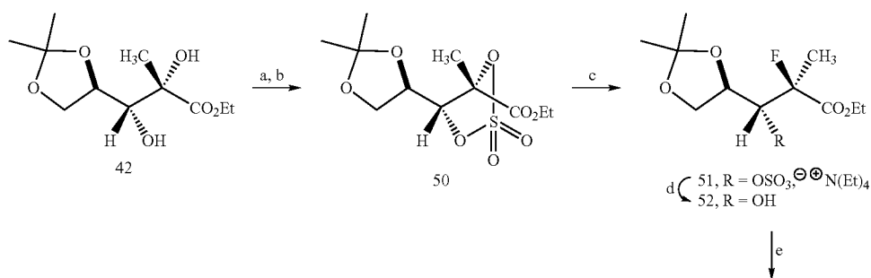
Scheme 6
