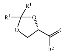
(S)-glyceraldehyde
