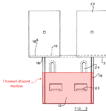
EX1040, FIG. 3 (annotated).
