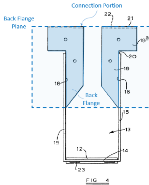
EX1040, FIG. 4 (annotated).
