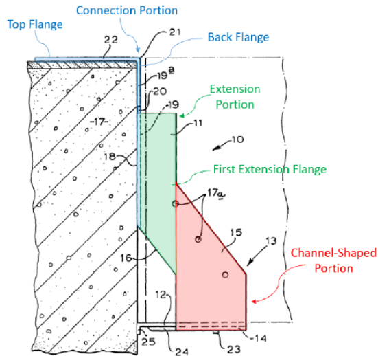
EX1040, FIG. 2 (annotated).
