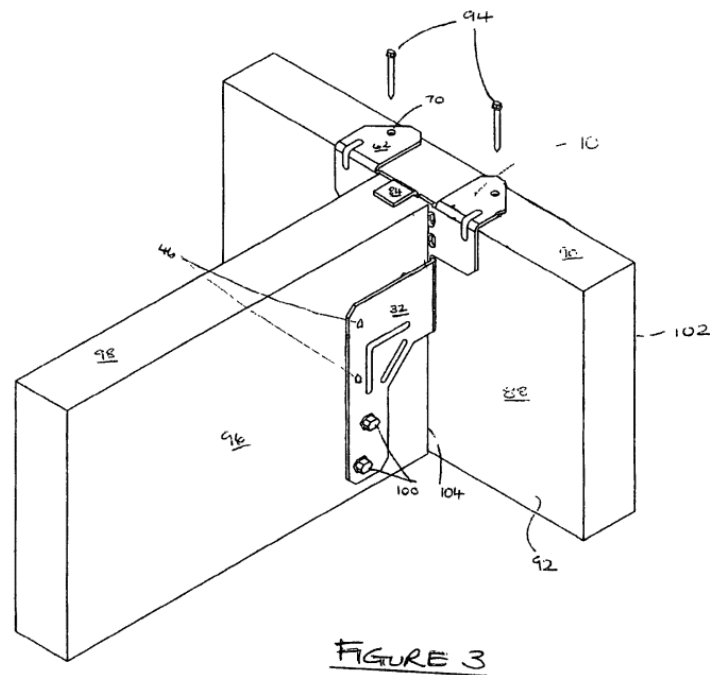
Figure 3 of Cullen is a schematic view of a portion of a decking platform including a bracket. Ex. 1039, 10:4–5.
