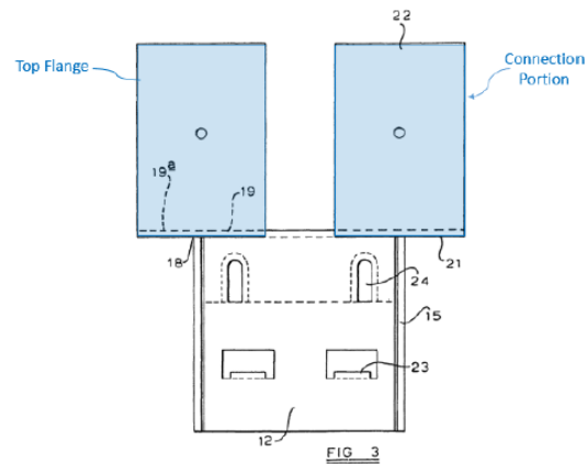
EX1040, FIG. 3 (annotated).
