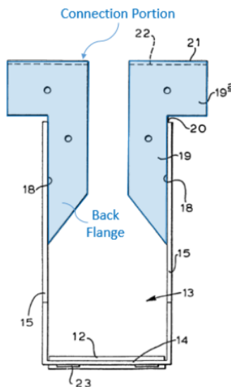
EX1040, FIG. 4 (annotated).
