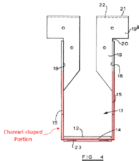
EX1040, FIG. 4 (annotated).
