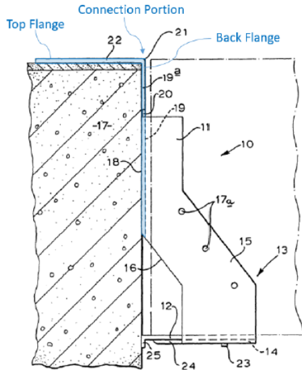
EX1040, FIG. 2 (annotated).
