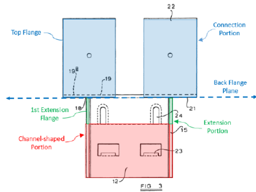
EX1040, FIG. 3 (annotated).
