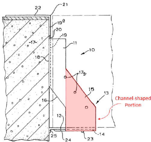
EX1040, FIG. 2 (annotated).
