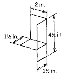
FIGURE 7.28 Typical framing anchor dimensions.
