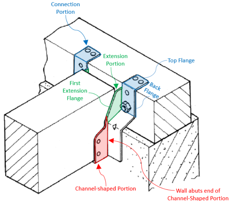
EX1041, 5, Usage View (annotations from Pet. 27 and additional annotations)
