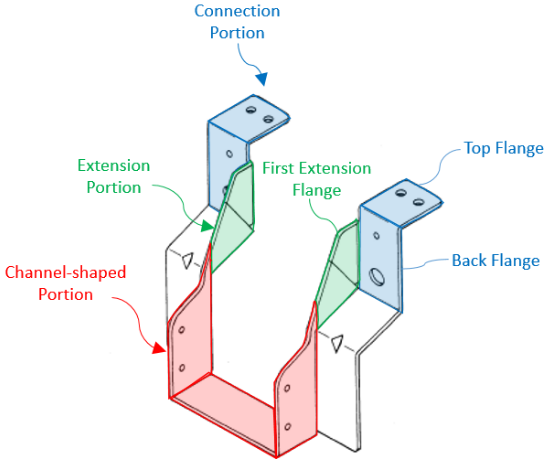
EX1041, 2, Perspective View (annotations from Pet., 27).
