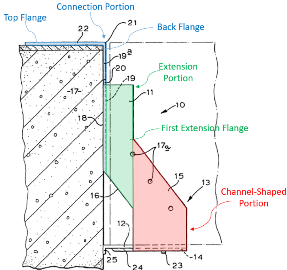
EX1040, FIG. 2 (annotations from Pet., 132).
