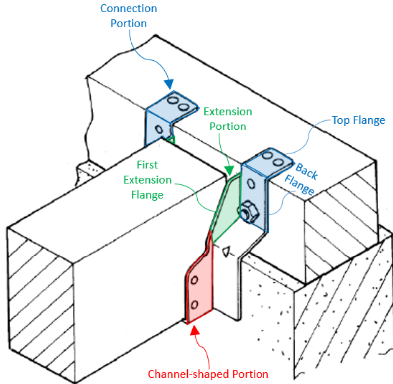
EX1041, 5, Usage View (annotations from Pet. 27).
