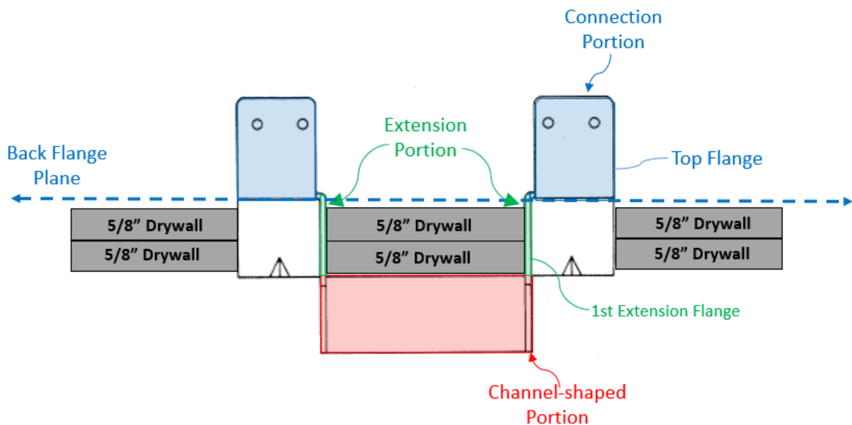
EX1041, 3, Plan View (annotations from Pet., 24).
