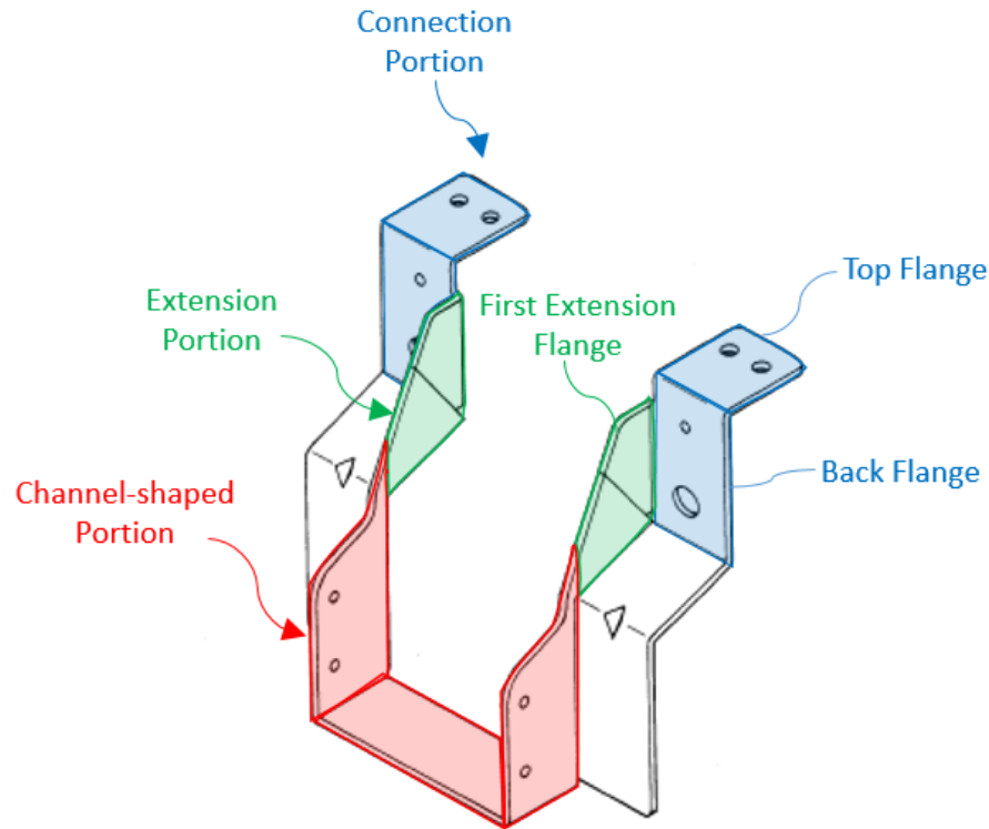
EX1041, 2, Perspective View (annotations from Pet., 32).
