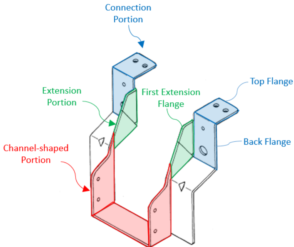
EX1041, 2, Perspective View (annotations from EX1003, ¶95).
