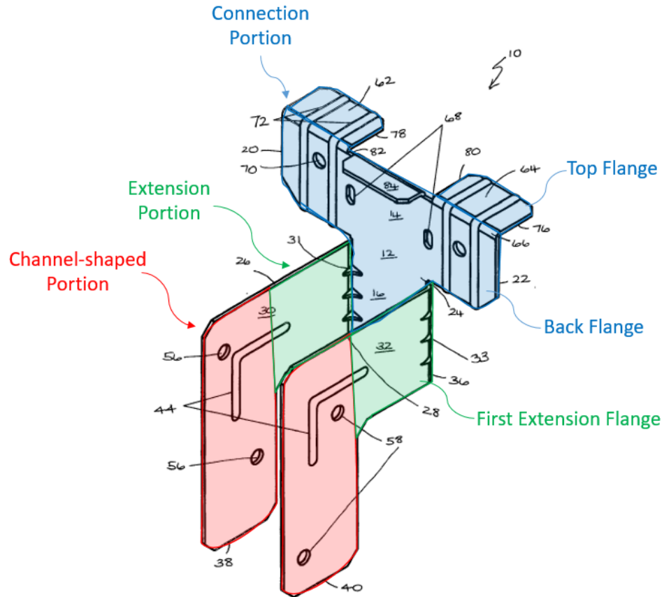
EX1039, FIG. 1 (annotations from EX1003, ¶175).
