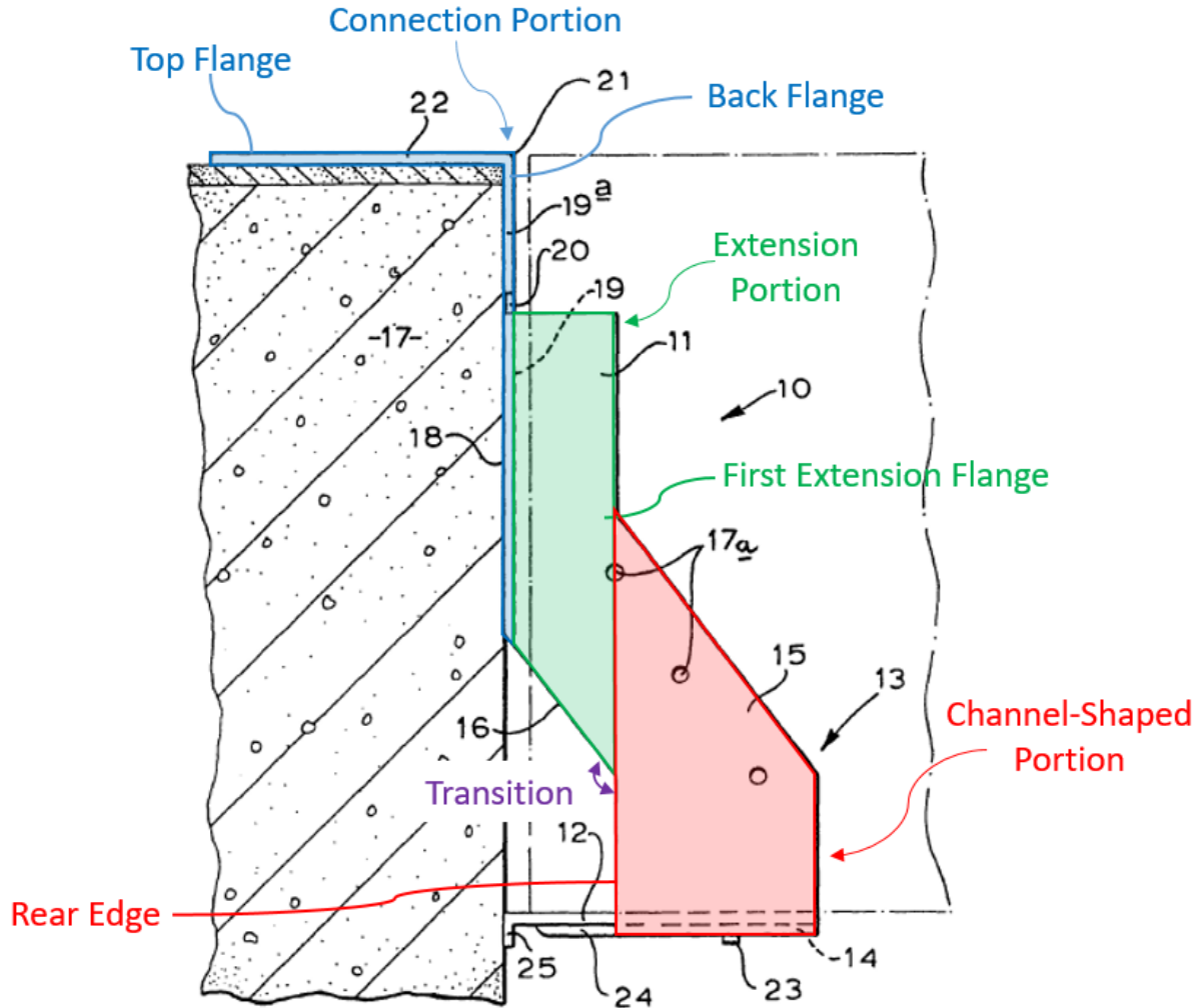
EX1040, FIG. 2 (annotated).
