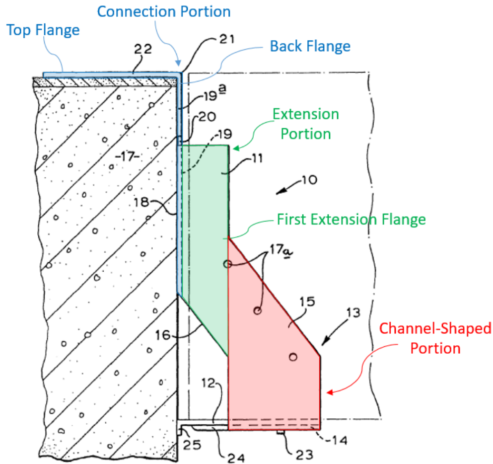
EX1040, FIG. 2 (annotations from EX1003, ¶249).
