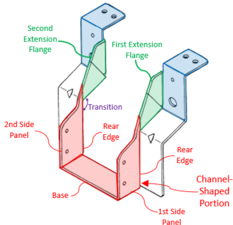
EX1041, 2, Perspective View (annotated).
