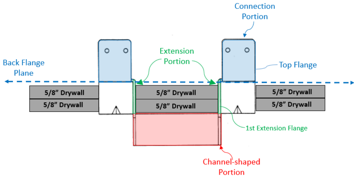
EX1041, 3, Plan View (annotations from EX1003, ¶98).
