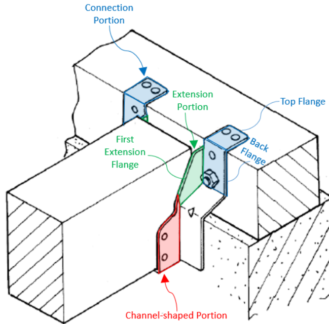
EX1041, 5, Usage View (annotations from EX1003, ¶95).
