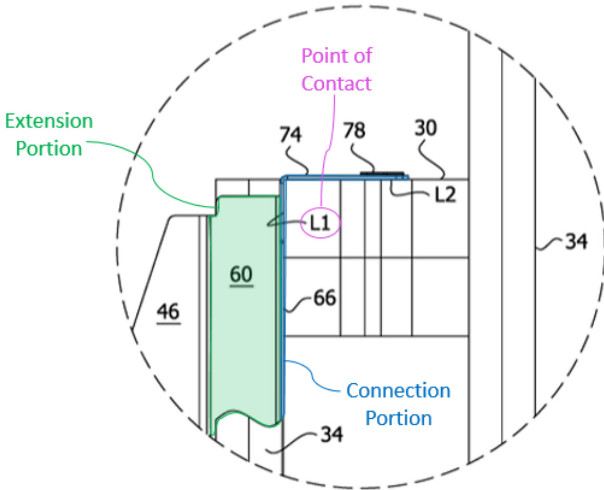
EX1001, FIG. 13A (annotated).
