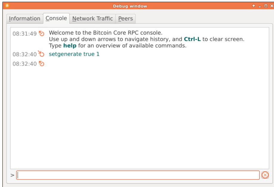
Fig. 2.1: Starting mining in Bitcoin Core
