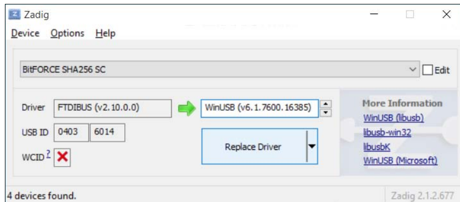
Fig. 5.3: Using Zadig to change a device driver
