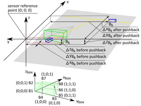
Figure 12. Definition of reference axes and coordinates of the bounding box corners B_k
