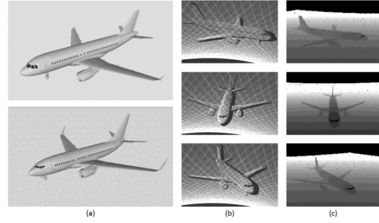
Figure 4. Training data generation. (a): 3D models of two aircraft. Top: Airbus 319-100. Bottom: Boeing 737-700. (b): Point clouds showing different poses of the Airbus 319-100 which were generated through sensor simulation by ray casting. (c): Depth image representation of the point clouds.
