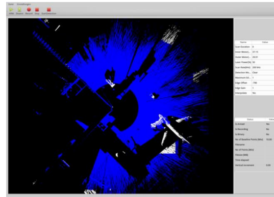
Figure 2. Experimental GUI displaying real-time detection results at Dresden airport, with detected objects coloured in white
