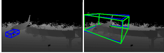
Figure 10. Before pushback: Manually annotated pose of tow truck (blue bounding box) in front of the nose of the Airbus A319 (left), estimated pose of Airbus A319 represented by green bounding box (right)
