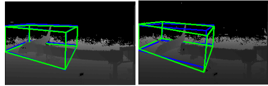
Figure 8. Depth image representation of Airbus A319 (left) and B737-700 (right) in 3D scans
