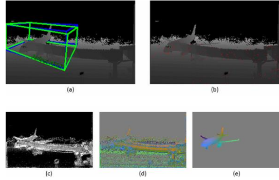
Figure 5. Overview of the classification process. (a): Depth image representation of a 3D scan showing an Airbus 319-100 in parking position. The ground truth 16 6D pose is depicted by the blue bounding volume. The estimated pose is shown in green. (b): Hypothesis generation process. Sampled hypotheses are projected into the image. Color coding: Hypotheses in red color were rejected by a geometric check. Hypotheses in green were refined. (c): Probability map for the query object. (d): Object coordinate prediction for the query object. (e): Ground truth object coordinates.
