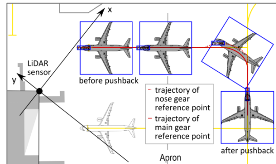
Figure 9. Pushback trajectory for an Airbus A319, consisting of both trajectories described by the nose and the main gear reference point during the pushback manoeuvre
