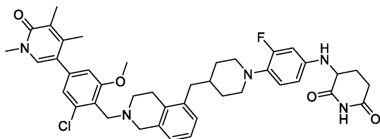
Isomer 2
