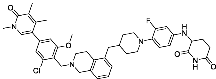
Isomer 1
