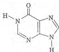
Hypoxanthine
