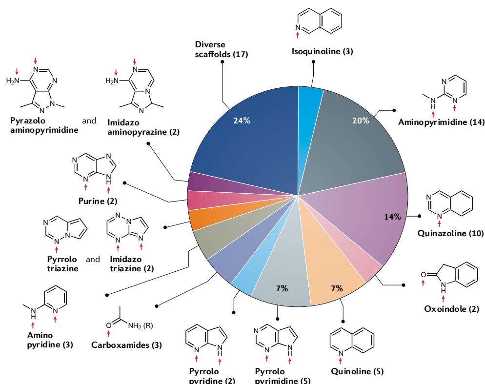
Fig. 4 | Chemical scaffolds used in approved kinase inhibitors. Chemical structures of the major hinge-binding scaffolds used in approved kinase inhibitors. Shown is the distribution of hinge-binding scaffolds for all ATP mimetic inhibitors (centre) as well as the structures of the most frequently used moieties. The number of approved drugs using each major scaffold is provided in brackets and each chemotype has been linked to the central pie chart by colour and numbering. Hydrogen bond donors and acceptors are indicated by red arrows.
