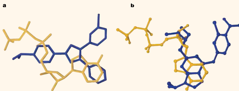
Figure 3 | Basis for the specificity of two ATP-competitive protein-kinase inhibitors. a | Comparison of the binding of SB203580 (blue) and ATP (yellow) to p38 MAPK 54 . b | Comparison of the binding of purvalanol (blue) and ATP (yellow) to CDK2 59 . Drug specificity is largely determined by the part of the molecule that does not interact with residues that bind ATP, but which occupies a hydrophobic binding pocket near the ATP-binding site. CDK2, cyclin-dependent kinase 2; p38 MAPK, p38 mitogen-activated protein kinase.
