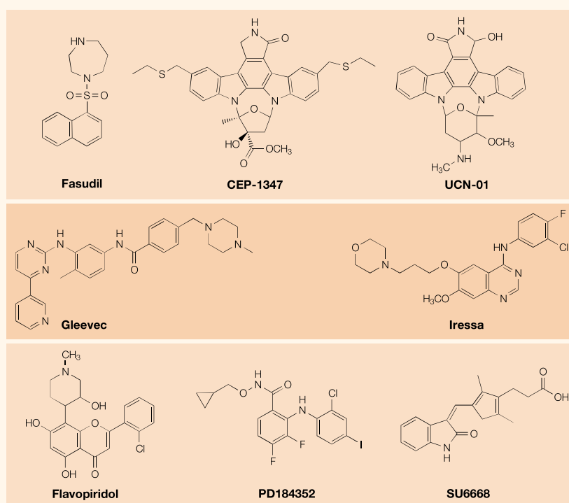
Figure 2 | Chemical structures of some small-molecule inhibitors of protein kinases that have been approved or are undergoing human clinical trials. Further information is given in the TIMELINE.
