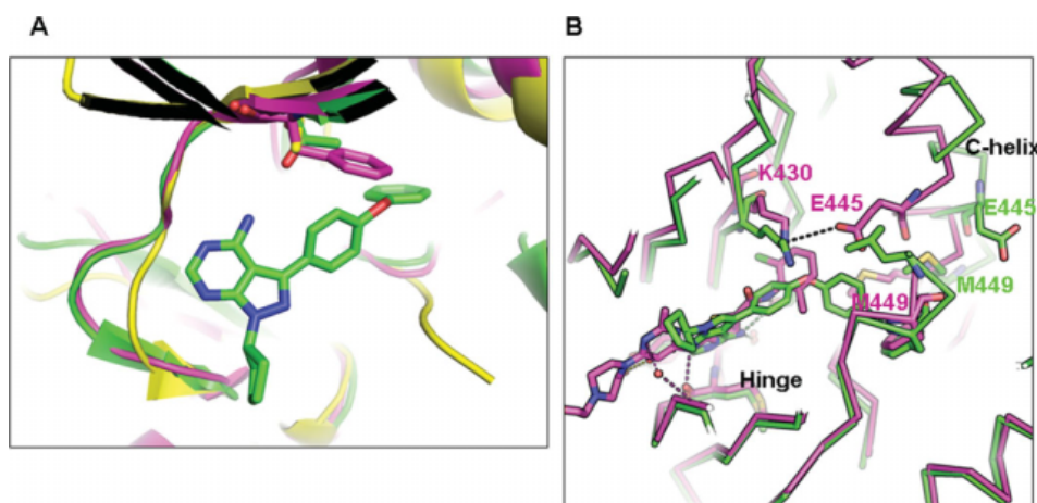
Figure 3. Differences between the “inactive” B43 and “active” Dasatinib-bound conformation of BTK. A: Overlay of BTK-KD bound to B43 (green), ITK bound to staurosporin (magenta, PDB ID: 1SNU) and P38 \alpha (yellow, PDB ID: 1P38). This indicates that the larger phenylalanine gatekeeper of ITK compared to the Thr474 gatekeeper of BTK prevents B43 from binding. It also indicates that the shorter hinge of P38 \alpha blocks the B43 binding site. B: Overlay of B43 structure (green) and Dasatinib structure (magenta) indicates that they superimpose well near the hinge but differ near the C-helix, resulting in a shift of >10 Å in the conformation of the Glu445 side chain and the residues that surround the hydrophobic back pocket.
