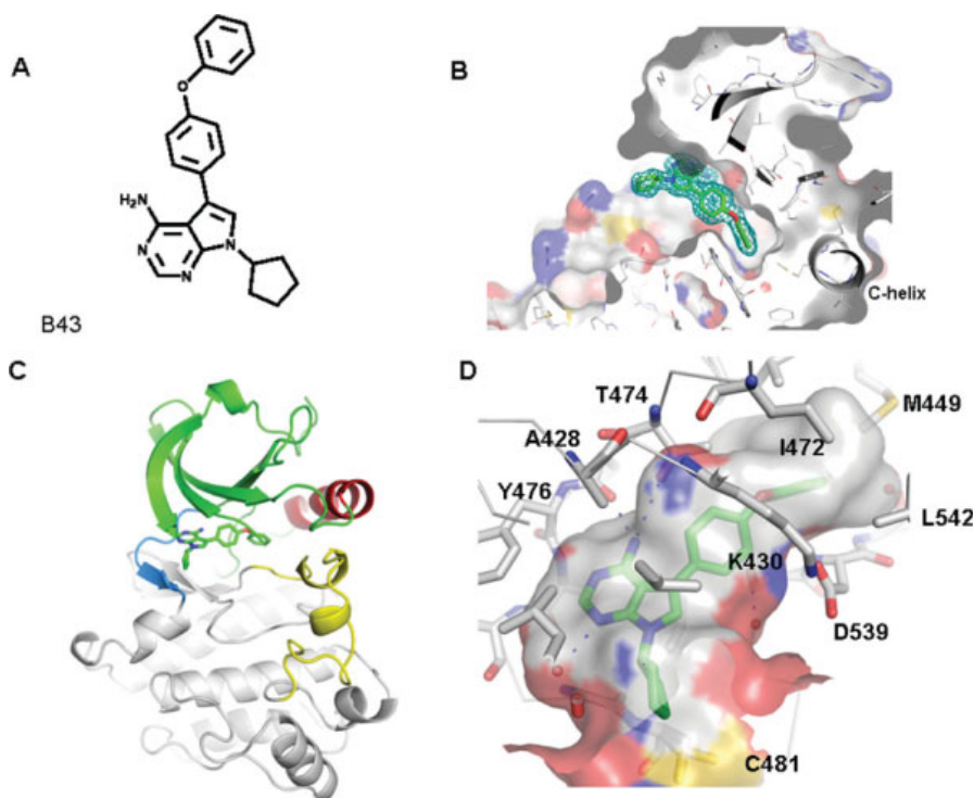
Figure 2. BTK-KD/B43 crystal structure. A: Chemical structure of B43. B: Electron density (2Fo-Fc map at 1 sigma) for B43 within a surface representation of the BTK protein in the human BTK-KD-B43 complex. C: Overall view of the BTK kinase domain bound to B43. Inhibitor (green), amino-terminal lobe (green), carboxy-terminal lobe (gray), C-helix (red), hinge (blue), and activation loop (yellow). D: Close-up of the active site and residues within 5 Å of the bound B43. The surface is colored according to the convention of base (blue) and acid (red). The active site cysteine is shown with a yellow surface.
