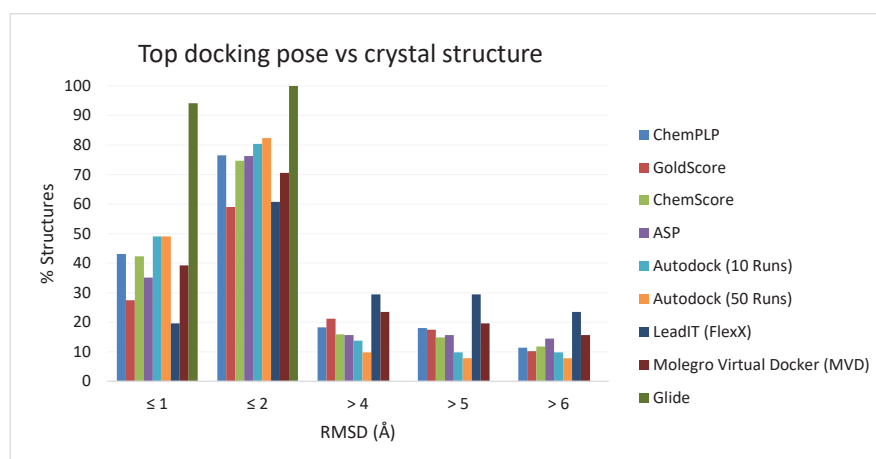
Fig. 1. Distribution of RMSD between the top-ranked docking pose and the corresponding experimentally determined pose in crystal structures. x axis: RMSD cutoffs y axis: percentage of top-ranked docking poses within a given RMSD cutoff values of the crystallographic pose.
