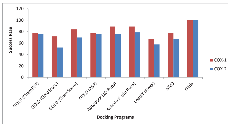
Fig. 3. Comparison of the performances of different docking methods on 18 COX1-inhibitor complexes and 32 COX2-inhibitor complexes presented in terms of percentages of docking solutions at RMSD cutoff level of \leq 2 Å.
