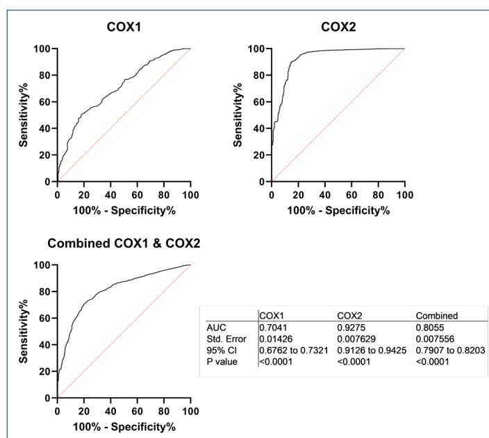
Fig. 4. The results of ROC analyses on docking scores for COX1 and COX2 active ligands and decoys obtained by Glide docking method. The plots show AUC curves for COX1, COX2, and combined COX1 and COX2 date sets. The statistics for ROC analyses are given in bottom right hand panel.
