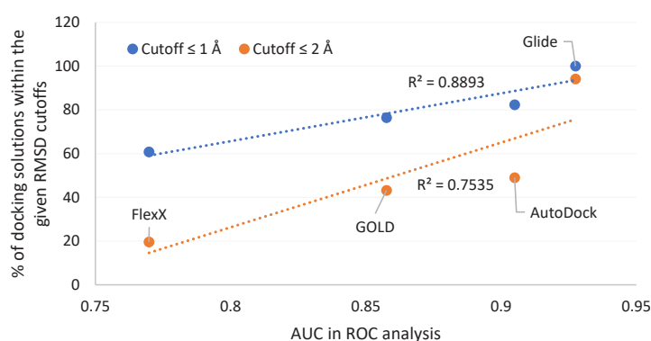
Fig. 5. Correlations between AUC values in ROC analyses on docking screening results and the percentages of docking solutions within the given RMSD cutoffs from the experimentally known positions of structurally known ligand-COX complexes using Glide, GOLD, AutoDock and FlexX software.
