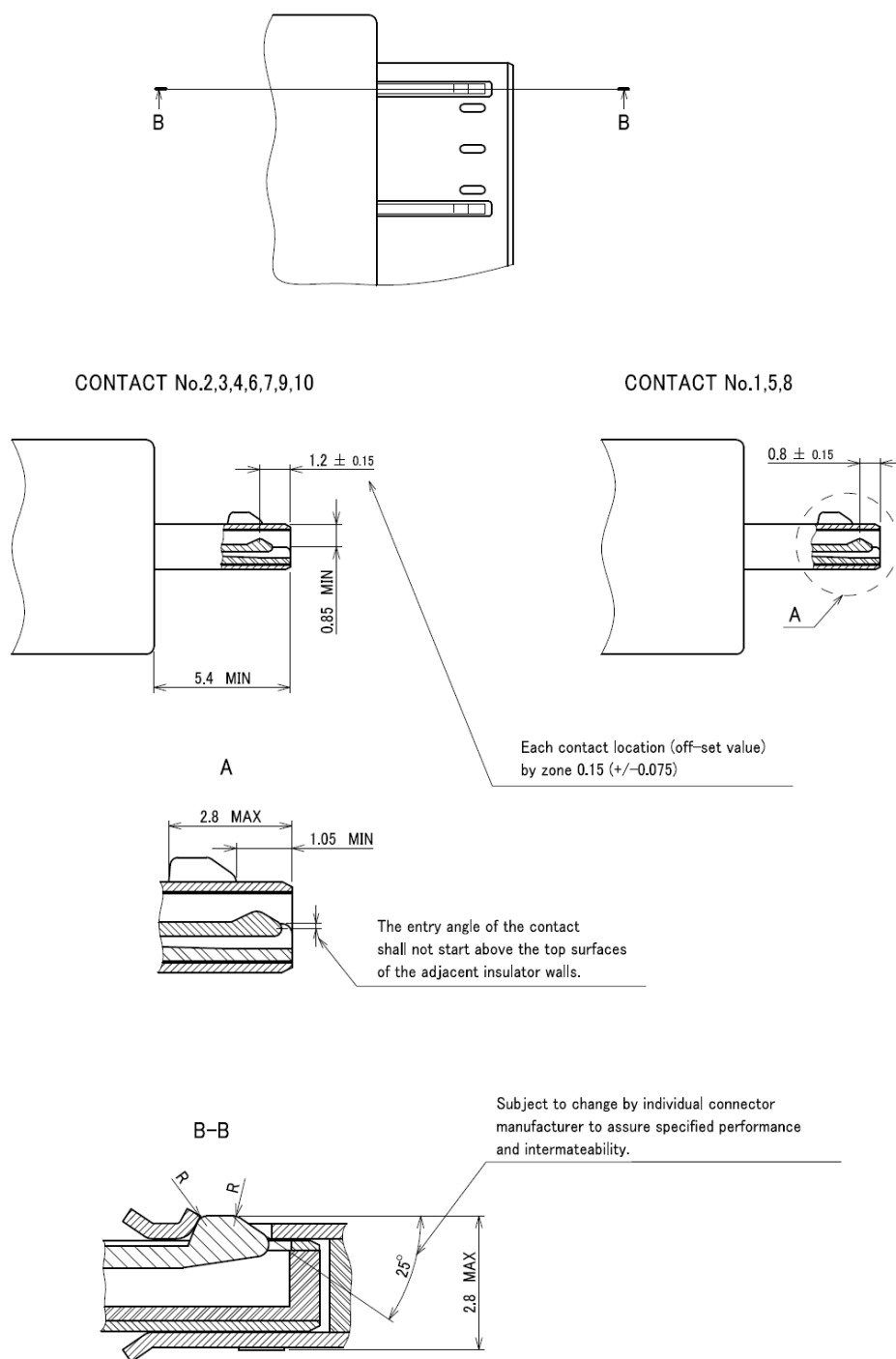
Figure 5-13. USB 3.0 Micro-B and Micro-A Plug Interface Dimensions
