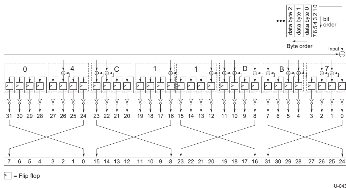
Figure 7-9. CRC-32 Remainder Generation
