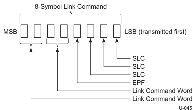
Figure 7-11. Link Command Structure
