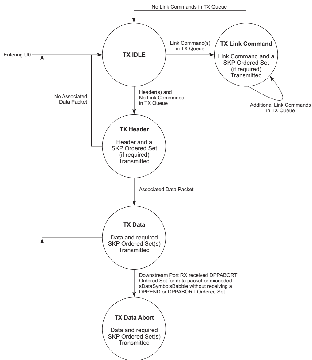
Figure 10-16. Upstream Facing Port Tx State Machine
