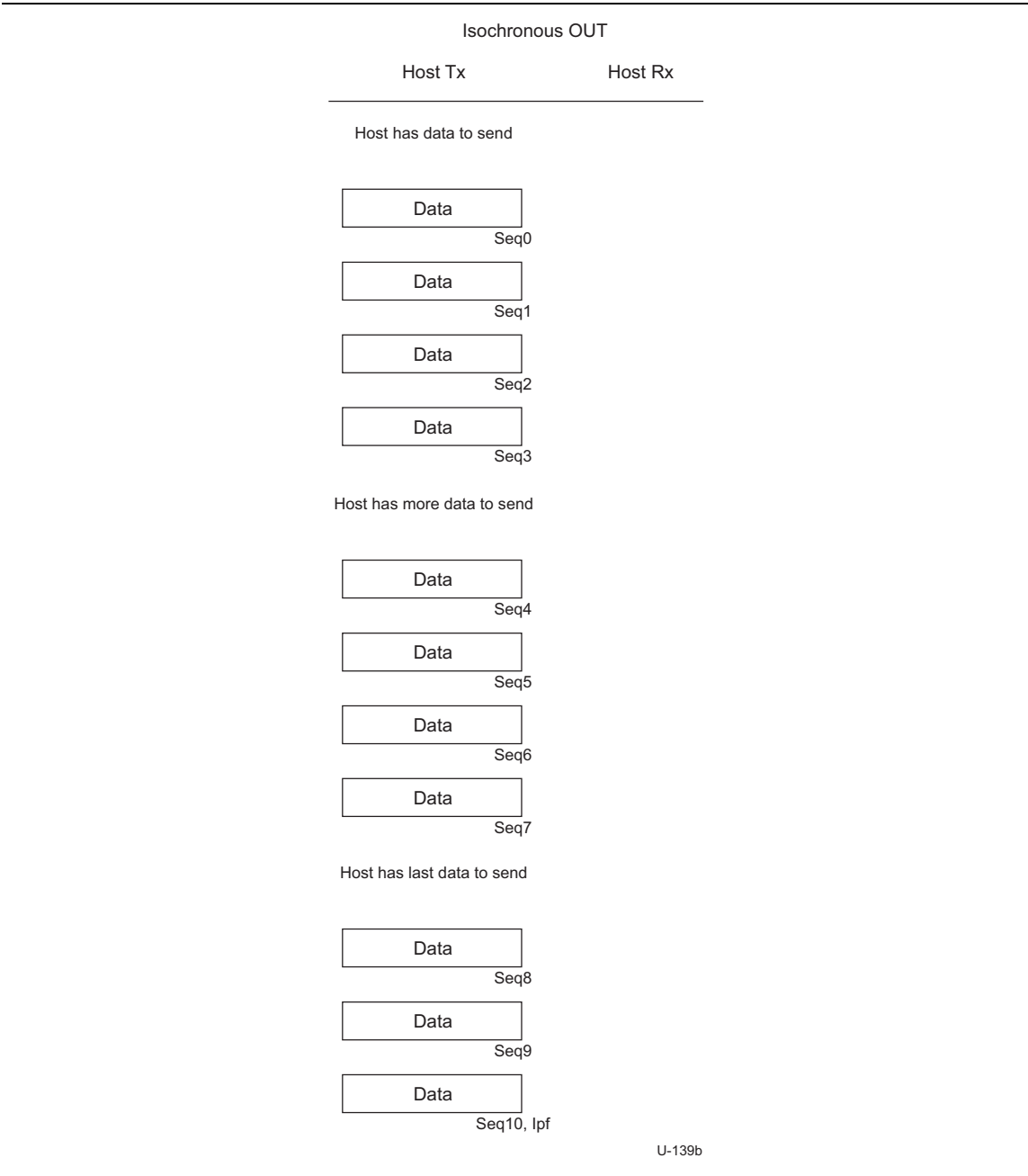
Figure 8-51. Isochronous OUT Transaction Example
