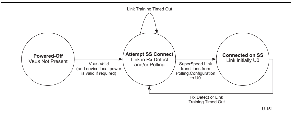
Figure 10-12. Hub Connect State Machine
