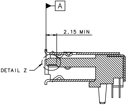
SECTION J-J
