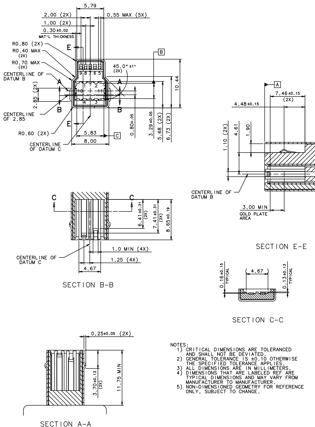
Figure 5-10. USB 3.0 Powered-B Plug Interface Dimensions
