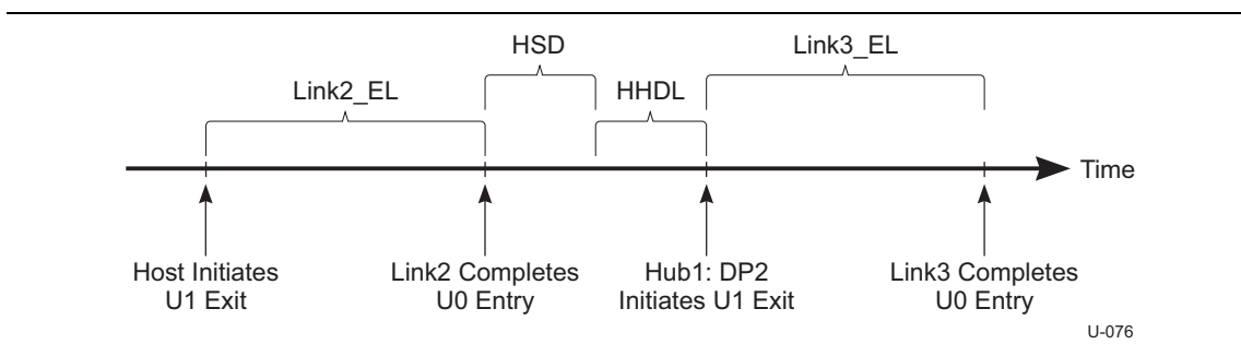
Figure C-6. Downstream Host to Device Path Exit Latency with Hub
