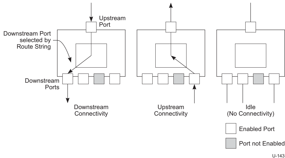
Figure 10-4. Hub Signaling Connectivity
