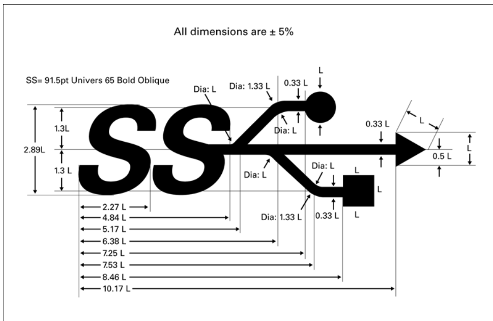
Figure 5-19. USB 3.0 Icon
