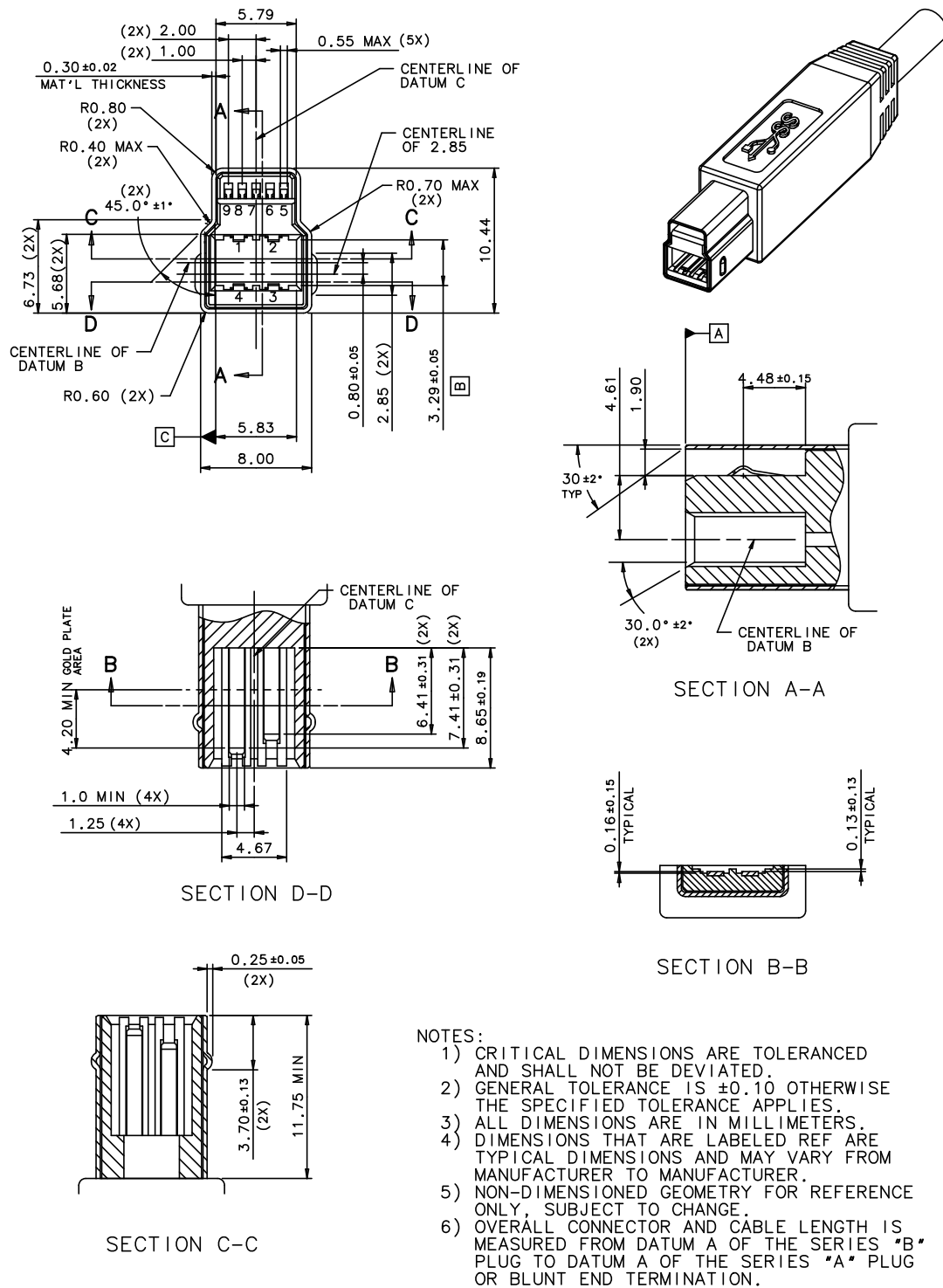
Figure 5-7. USB 3.0 Standard-B Plug Interface Dimensions
