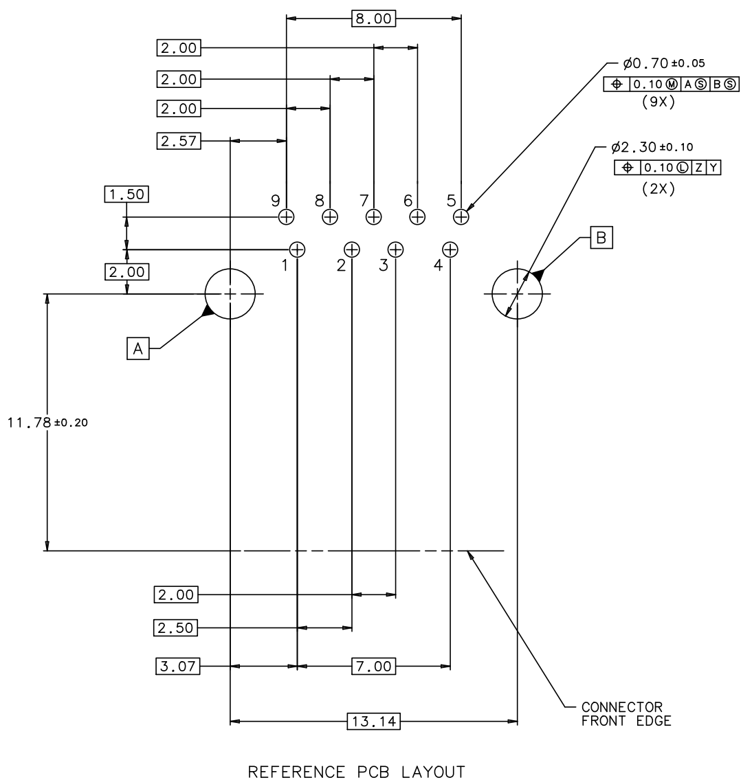
Figure 5-3. Reference Footprint for the USB 3.0 Standard-A Receptacle
