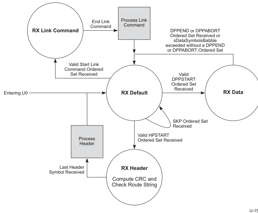
Figure 10-17. Upstream Facing Port Rx State Machine
