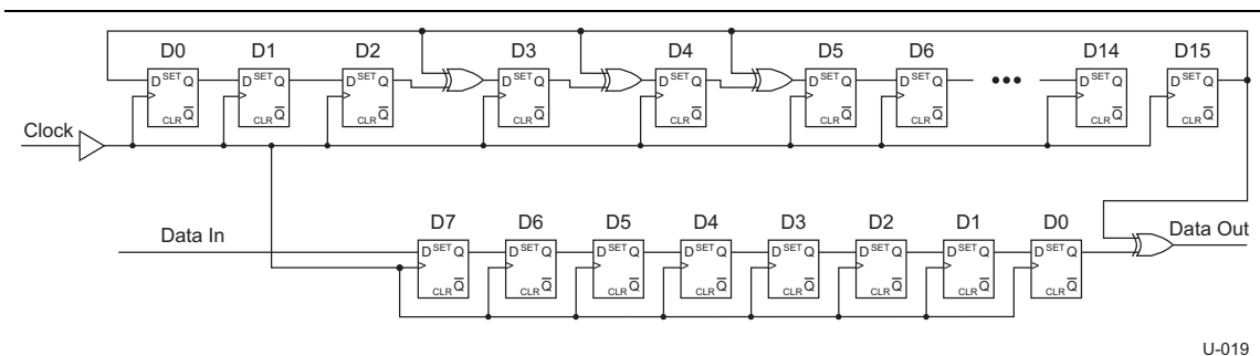
Figure 6-7. LFSR with Scrambling Polynomial
