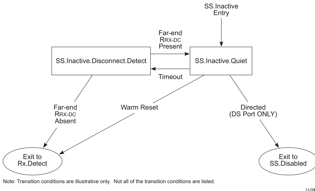
Figure 7-14. SS.Inactive Substate Machine
