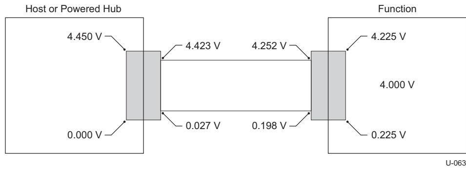
Figure 11-5. Worst-case Voltage Drop Topology (Steady State)
