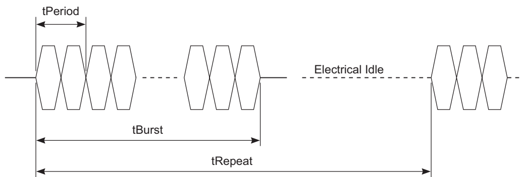
Figure 6-20. LFPS Signaling
