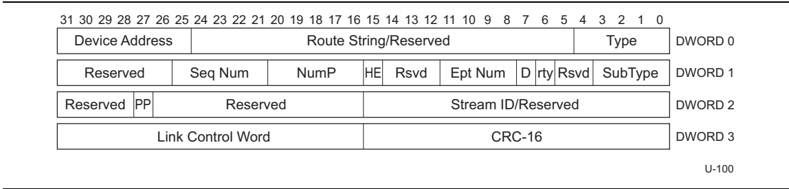
Figure 8-11. ACK Transaction Packet
