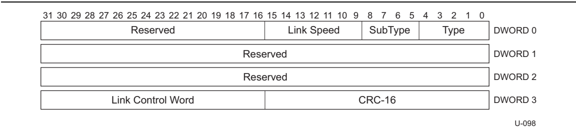
Figure 8-9. Port Configuration LMP
