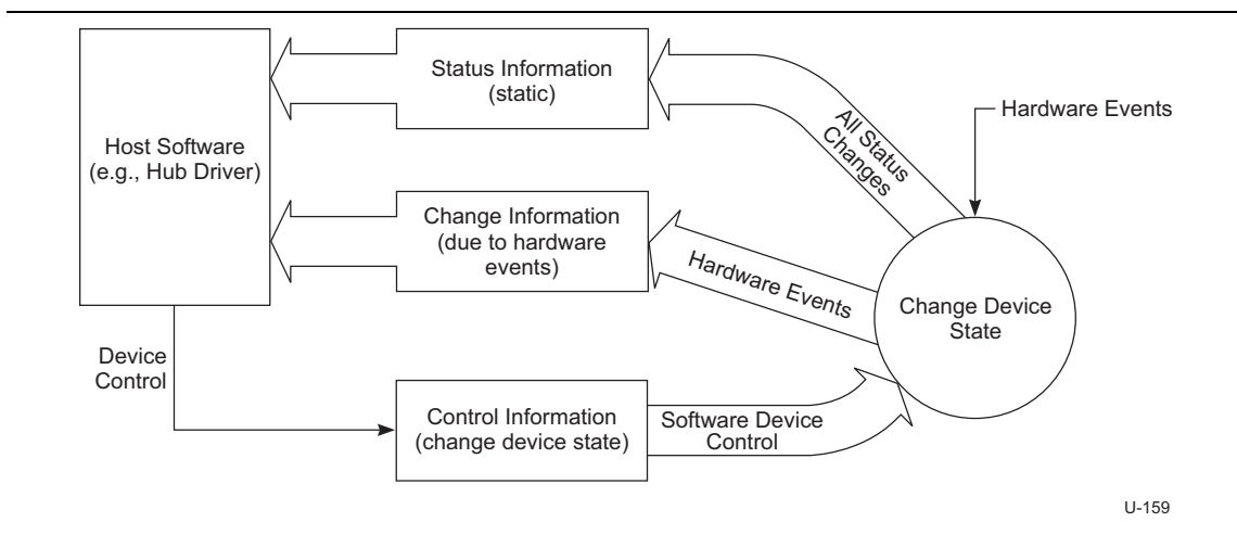
Figure 10-21. Relationship of Status, Status Change, and Control Information to Device States
