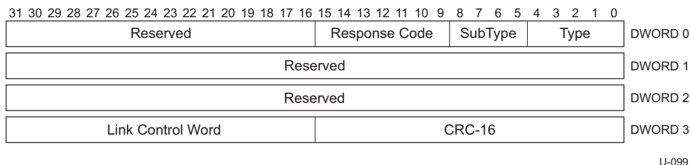
Figure 8-10. Port Configuration Response LMP
