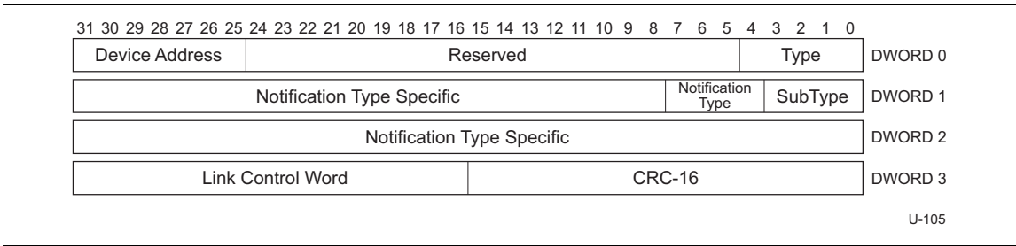
Figure 8-16. Device Notification Transaction Packet
