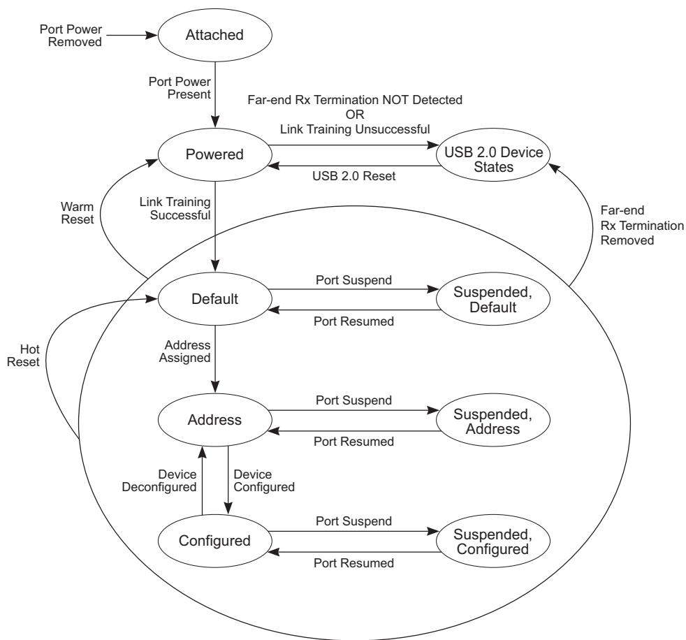
Figure 9-1. Peripheral Device State Diagram
