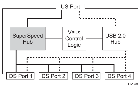
Figure 10-1. Hub Architecture
