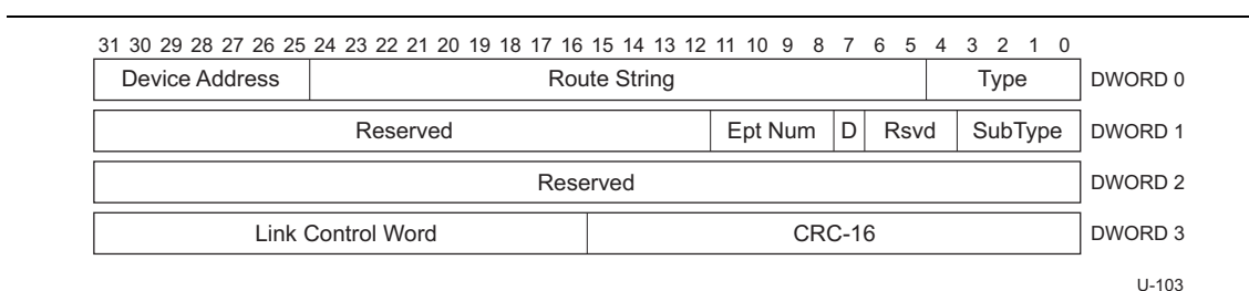
Figure 8-14. STATUS Transaction Packet
