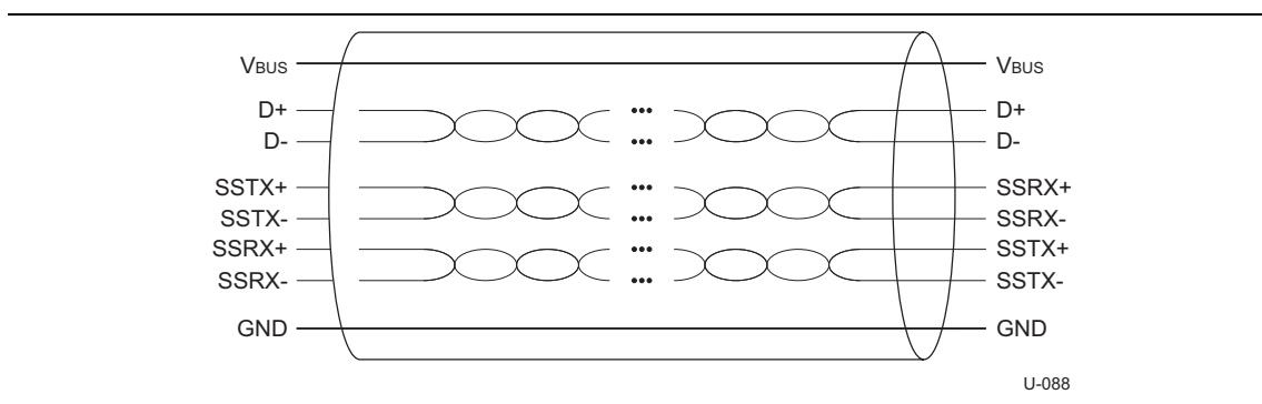
Figure 3-2. USB 3.0 Cable
