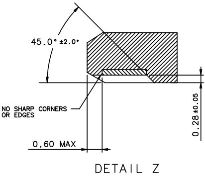
DETAIL Z
