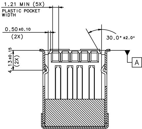
SECTION S-S
