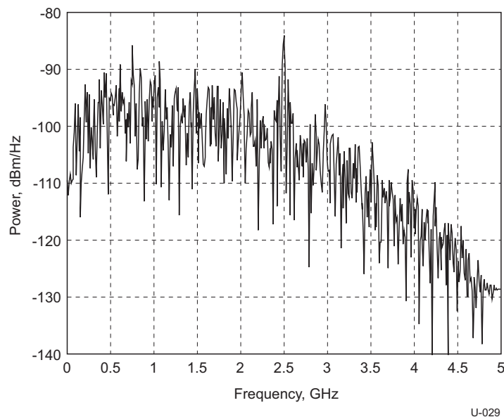
Figure 6-16. Frequency Spectrum of TSEQ
