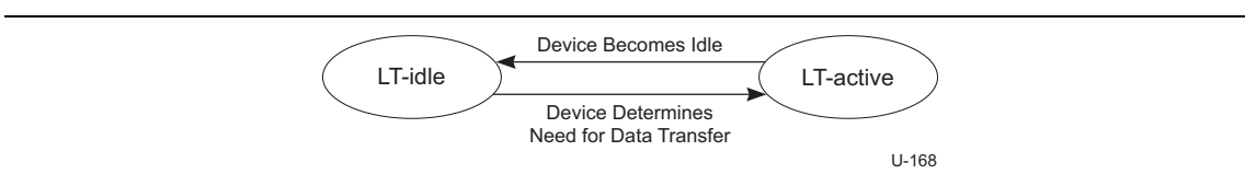
Figure C-8. LT State Diagram
