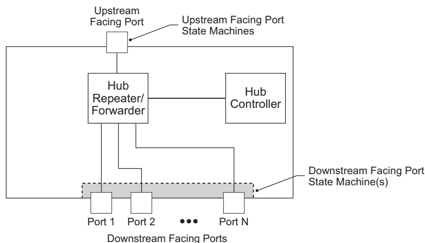
Figure 10-2. SuperSpeed Portion of the Hub Architecture
