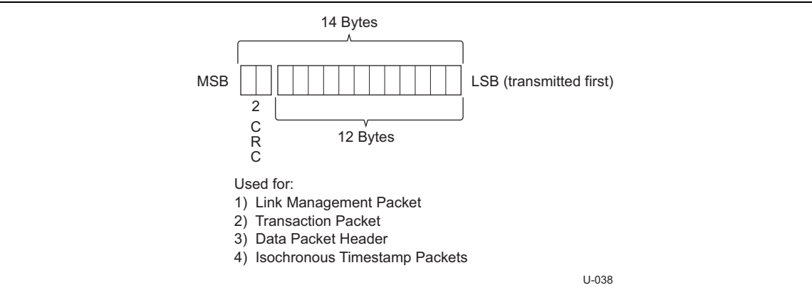
Figure 7-4. Packet Header
