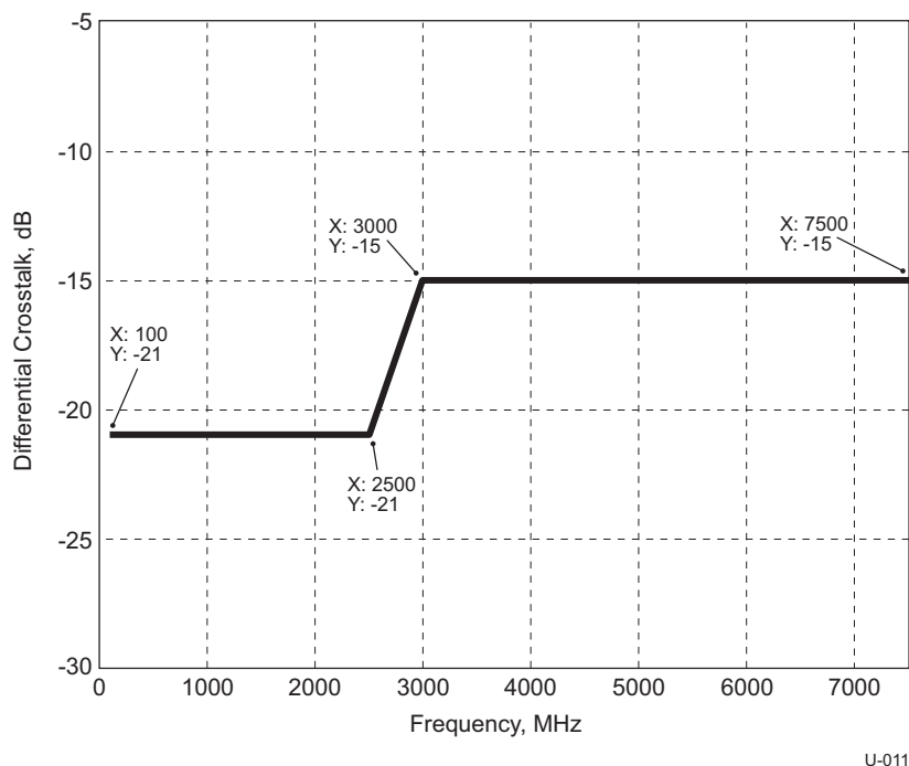
Figure 5-25. Differential Near-End and Far-End Crosstalk Requirement Between D+/D- Pair and SuperSpeed Pairs
