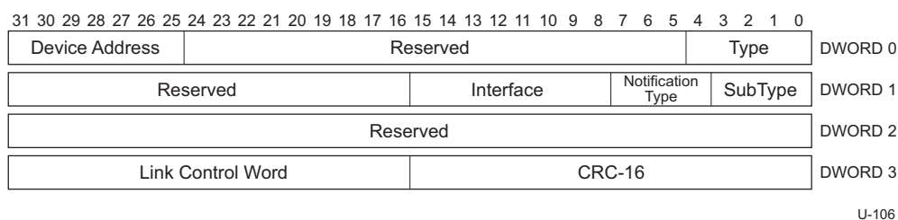
Figure 8-17. Function Wake Device Notification
