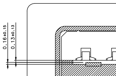
SECTION Q-Q
