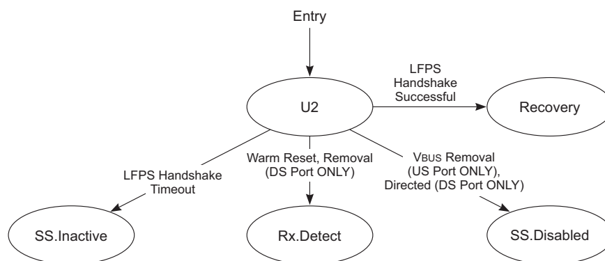
Figure 7-18. U2
