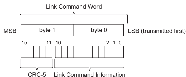
Figure 7-12. Link Command Word Structure
