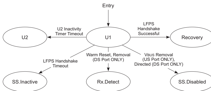
Figure 7-17. U1
