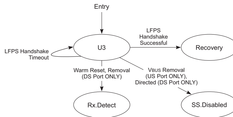
Figure 7-19. U3
