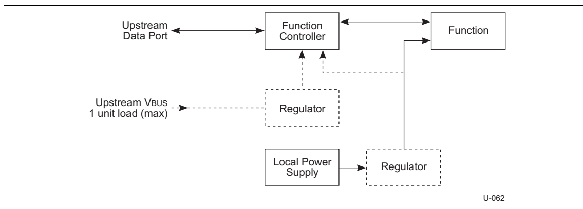
Figure 11-4. Self-powered Function
