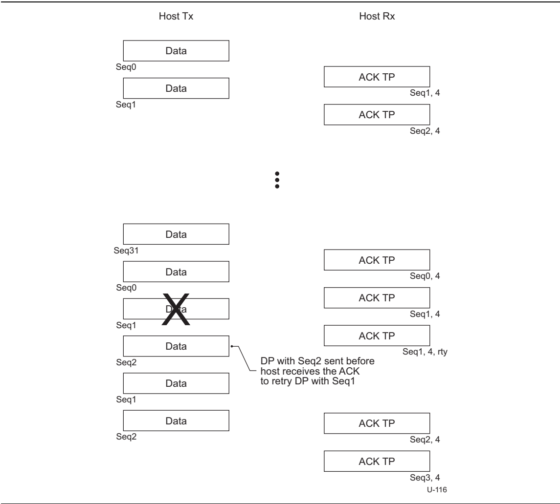
Figure 8-27. Sample BULK OUT Sequence
