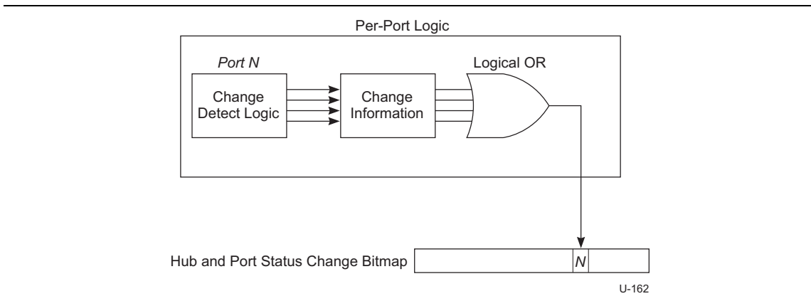
Figure 10-24. Example Hub and Port Change Bit Sampling
