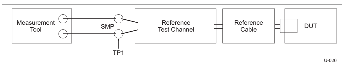
Figure 6-14. Tx Normative Setup with Reference Channel
