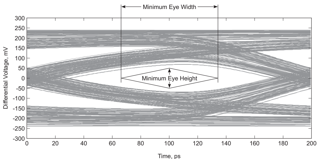
Figure 6-11. Generic Eye Mask
