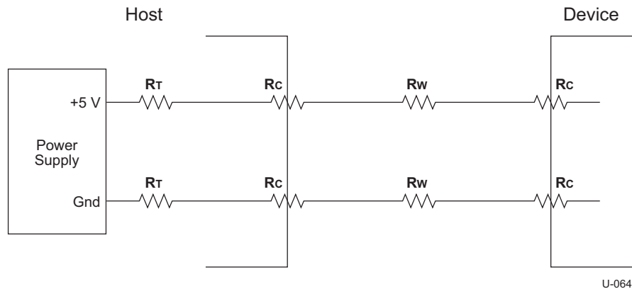
Figure 11-6. Worst-case Voltage Drop Analysis Using Equivalent Resistance
