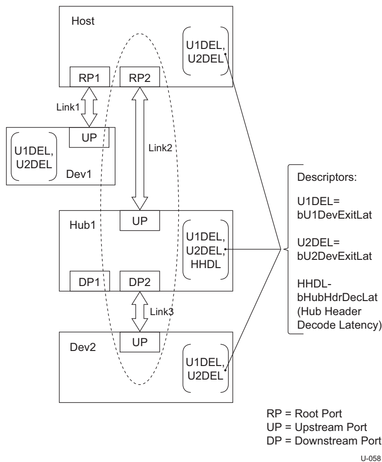
Figure C-5. Device Connected Through a Hub
