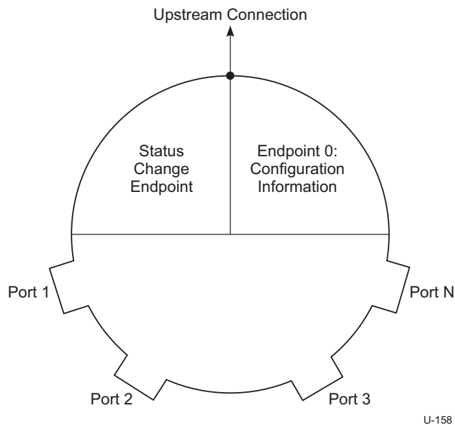
Figure 10-20. Example Hub Controller Organization
