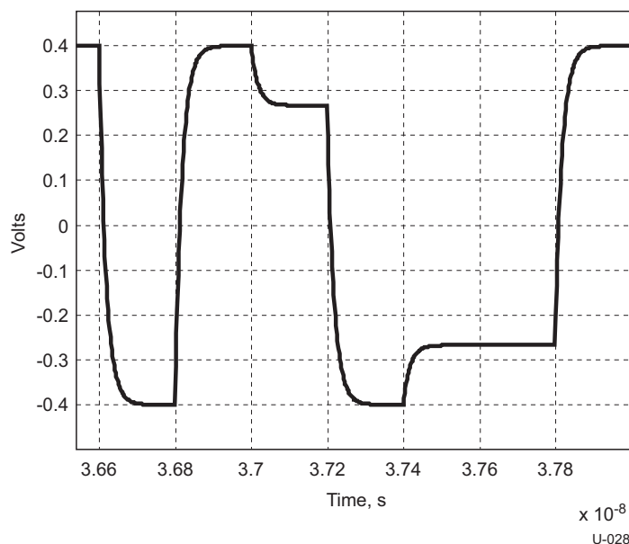
Figure 6-15. De-Emphasis Waveform
