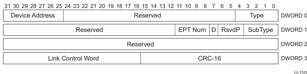
Figure 8-21. PING_RESPONSE Transaction Packet
