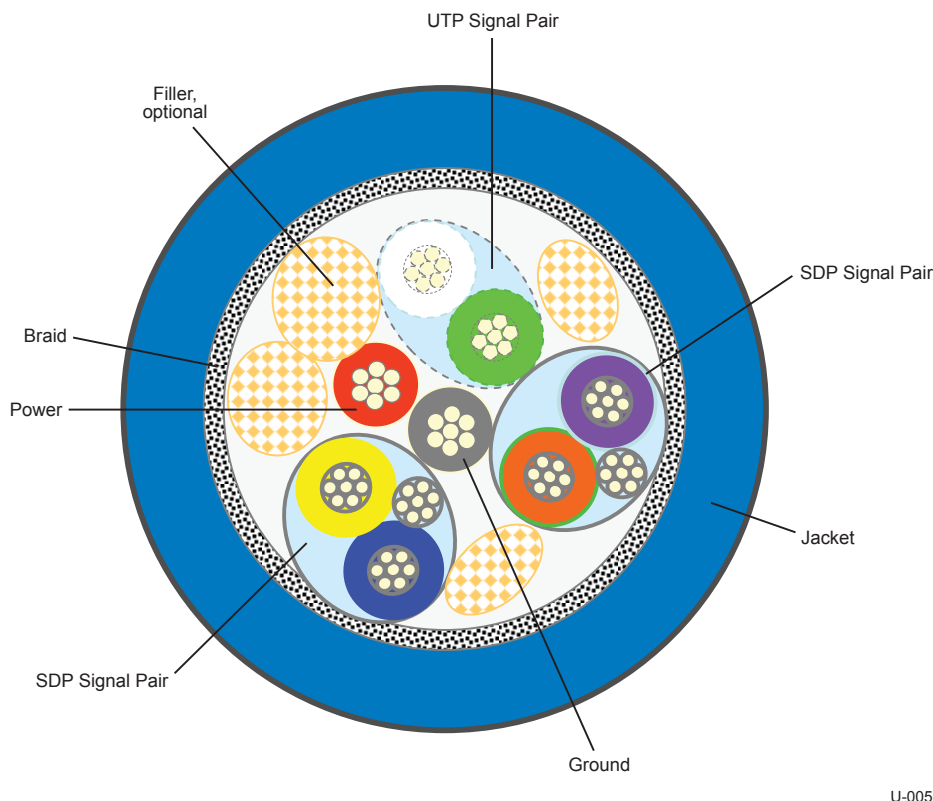
Figure 5-15. Illustration of a USB 3.0 Cable Cross-Section
