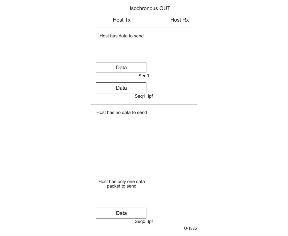
Figure 8-49. Sample Isochronous OUT Transaction
