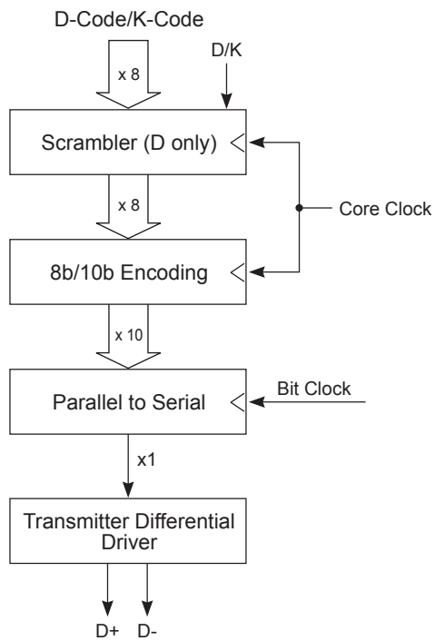
Figure 6-2. Transmitter Block Diagram
