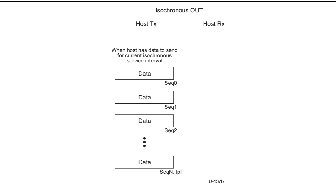
Figure 8-47. Isochronous OUT Transaction Format
