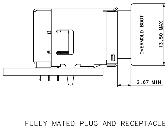
Figure 5-29. Mated USB 3.0 Standard-B Connector
