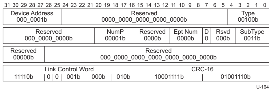
Figure D-1. Sample ERDY Transaction Packet
