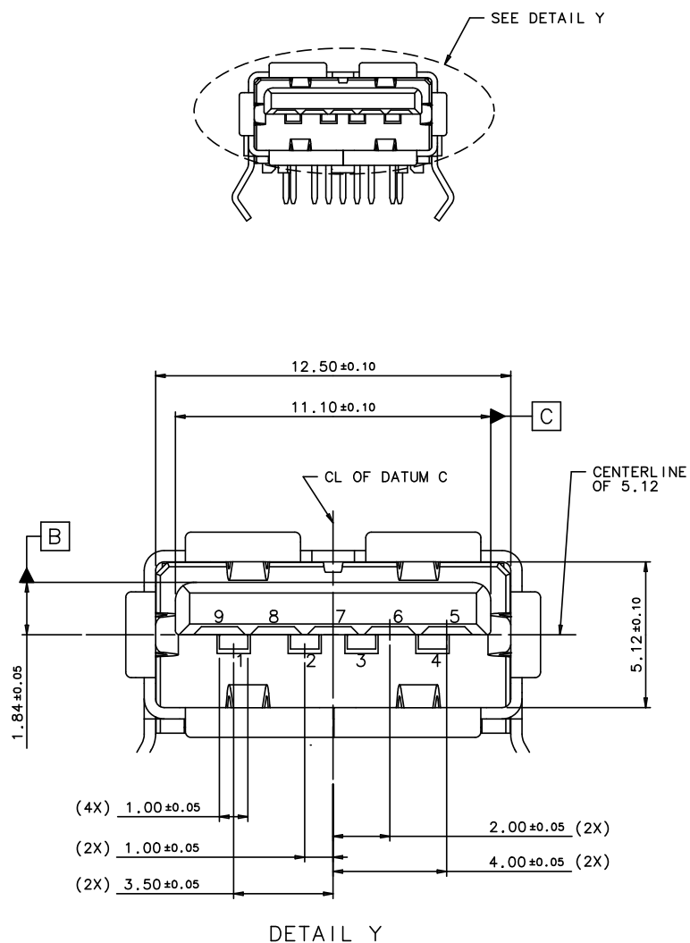
Figure 5-1. USB 3.0 Standard-A Receptacle Interface Dimensions
