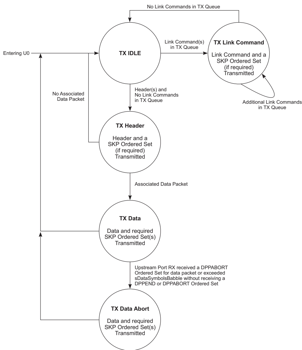
Figure 10-18. Downstream Facing Port Tx State Machine
