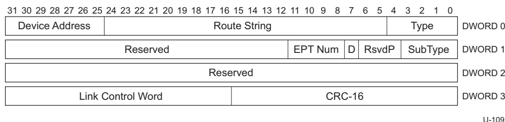
Figure 8-20. PING Transaction Packet
