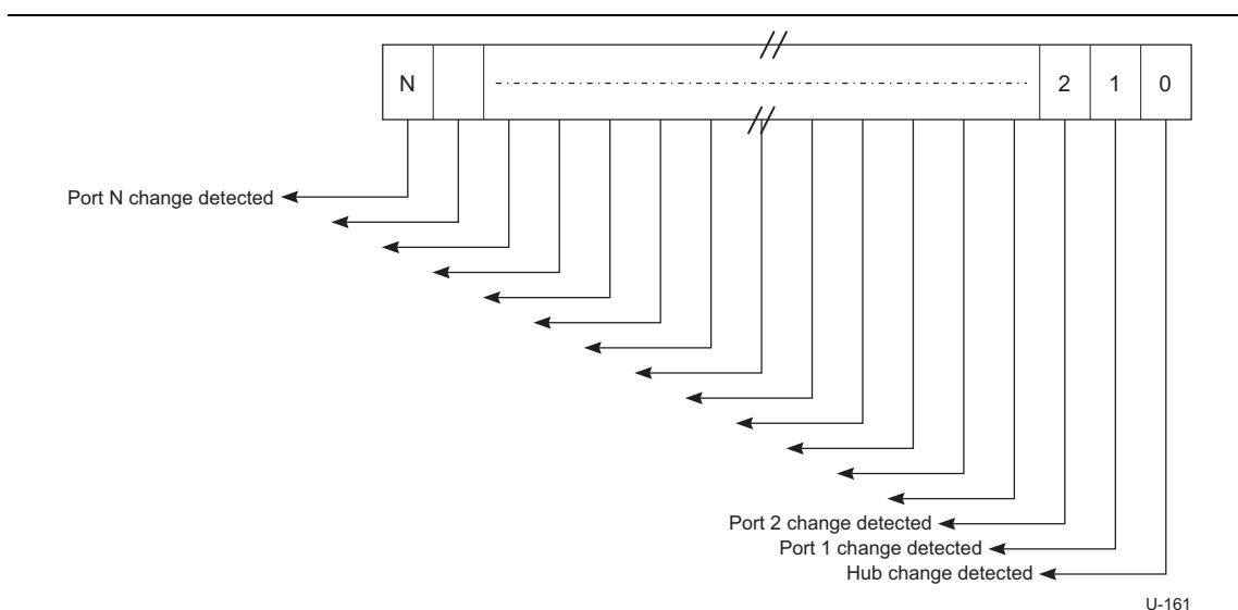
Figure 10-23. Hub and Port Status Change Bitmap
