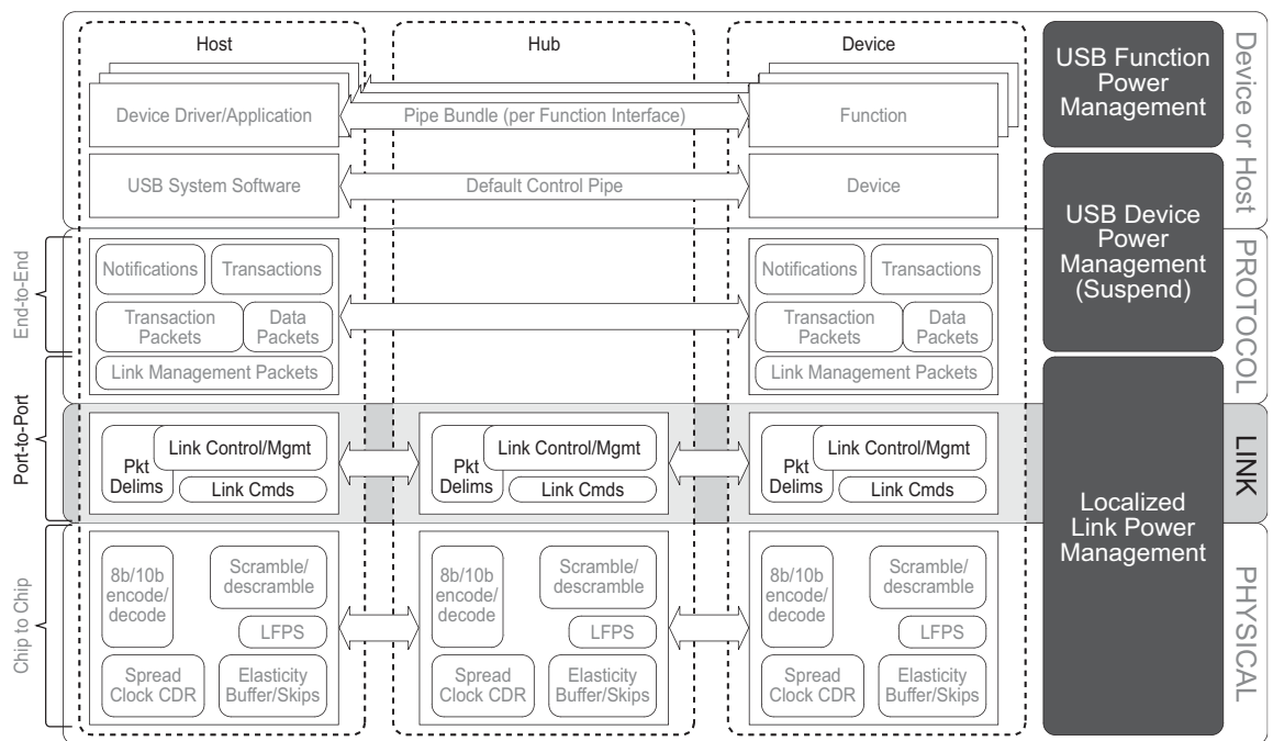
Figure 7-1. Link Layer
