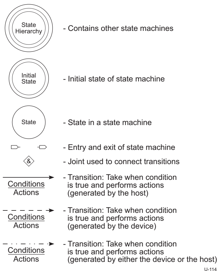
Figure 8-25. Legend for State Machines
