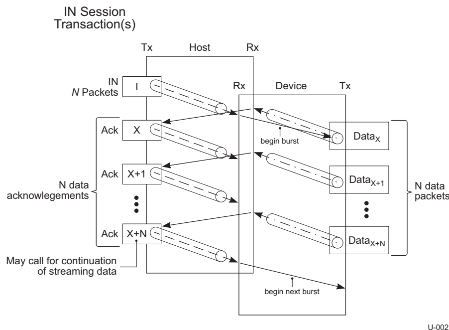
Figure 4-1. SuperSpeed IN Transaction Protocol
