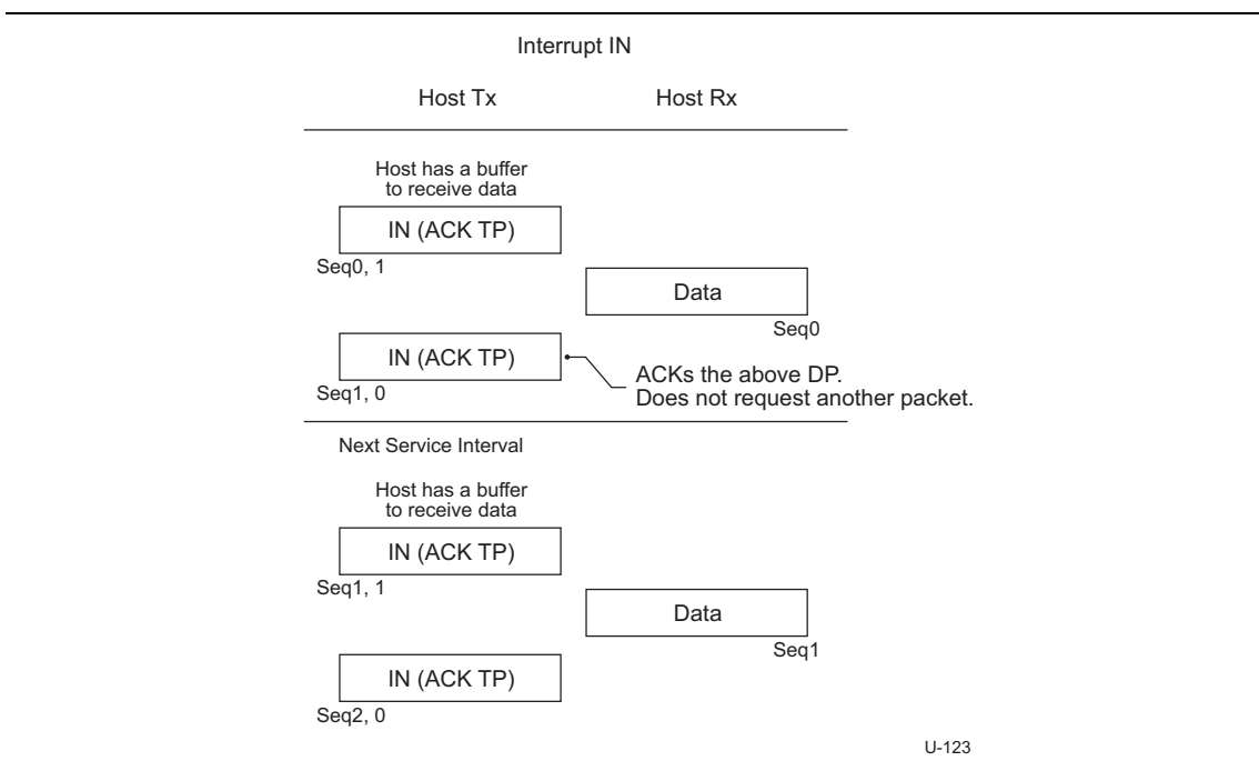
Figure 8-35. Host Sends Interrupt IN Transaction in Each Service Interval
