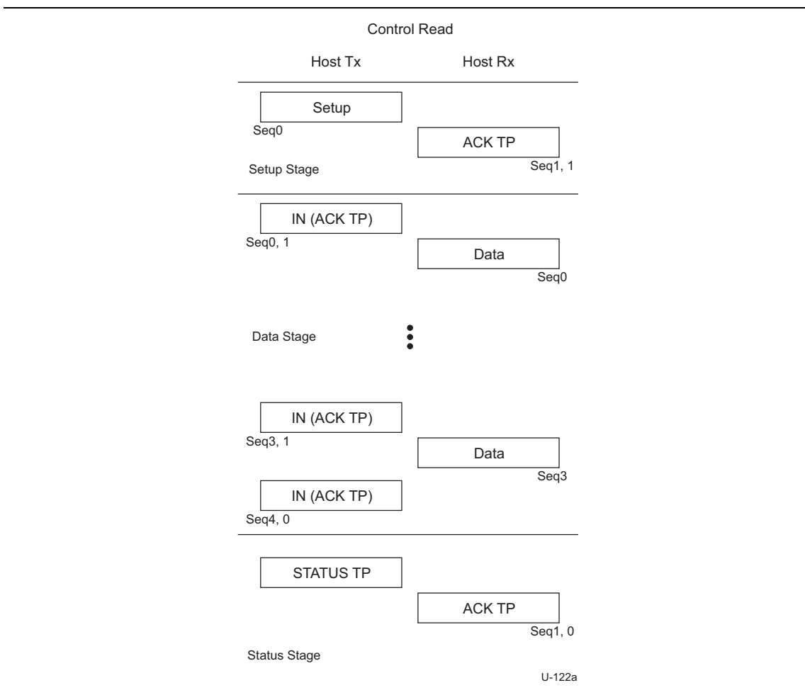
Figure 8-33. Control Read Sequence
