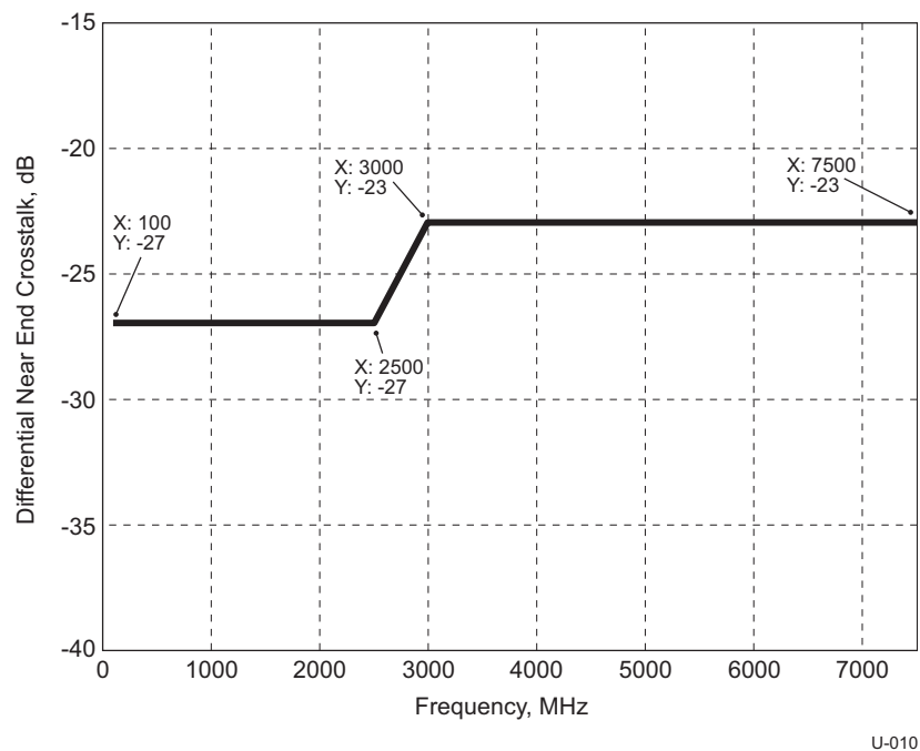
Figure 5-24. Differential Near-End Crosstalk Requirement Between SuperSpeed Pairs
