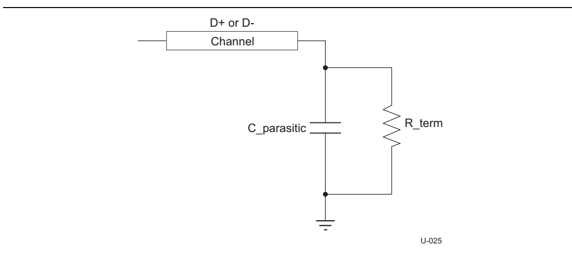
Figure 6-13. Device Termination Schematic
