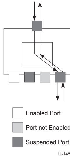
Figure 10-6. Resume Connectivity
