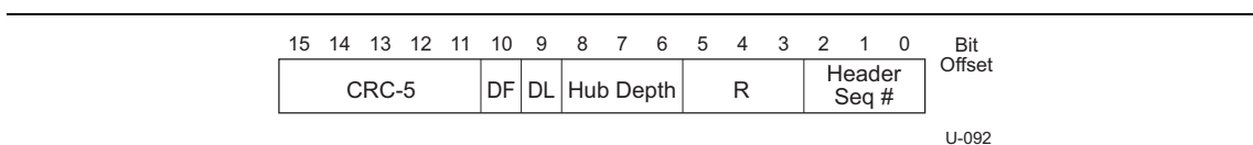
Figure 8-3. Link Control Word Detail
