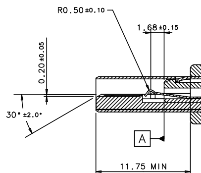
SECTION M-M
