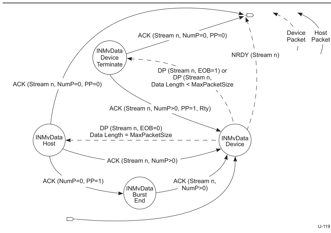
Figure 8-30. IN Move Data State Machine (IMDSM)
