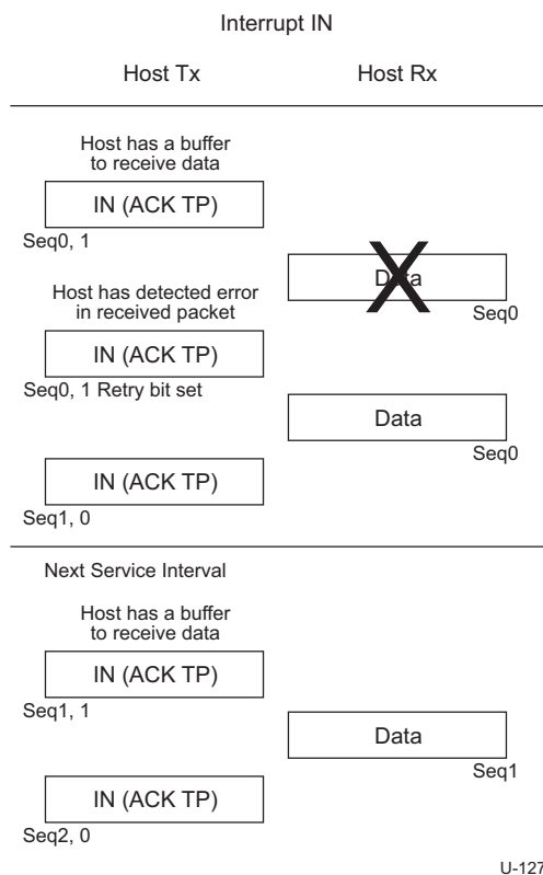
Figure 8-39. Host Detects Error in Data and Device Resends Data
