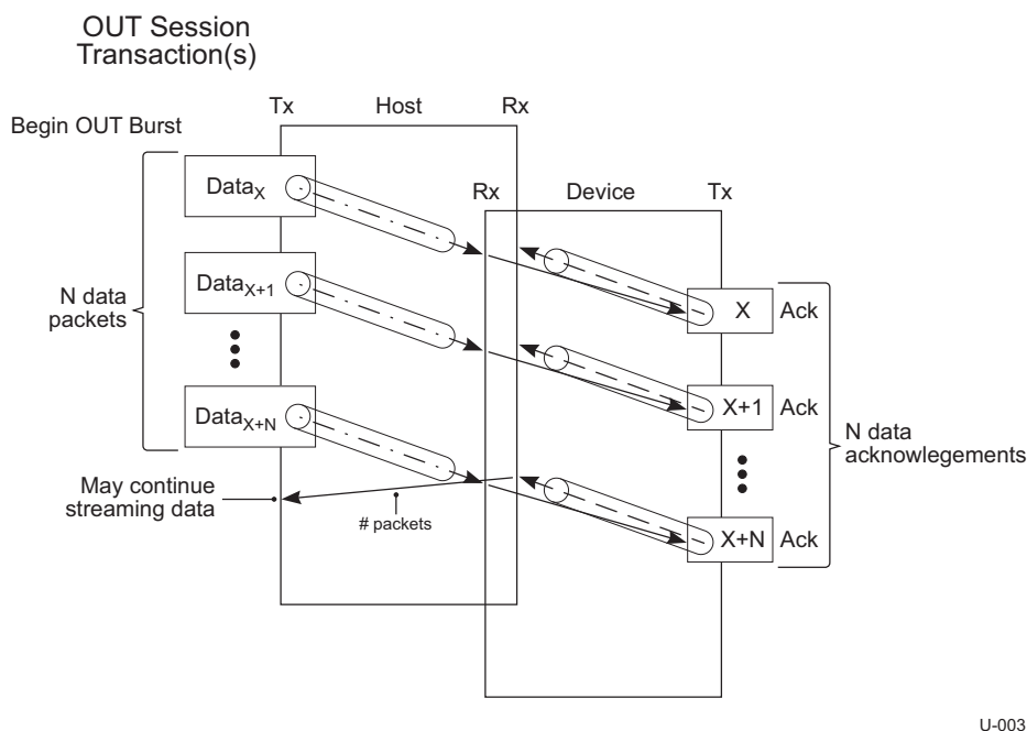
Figure 4-2. SuperSpeed OUT Transaction Protocol
