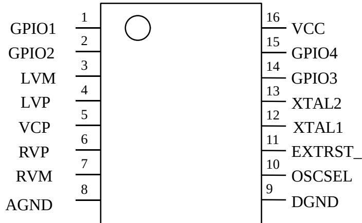
16-pin SOP
