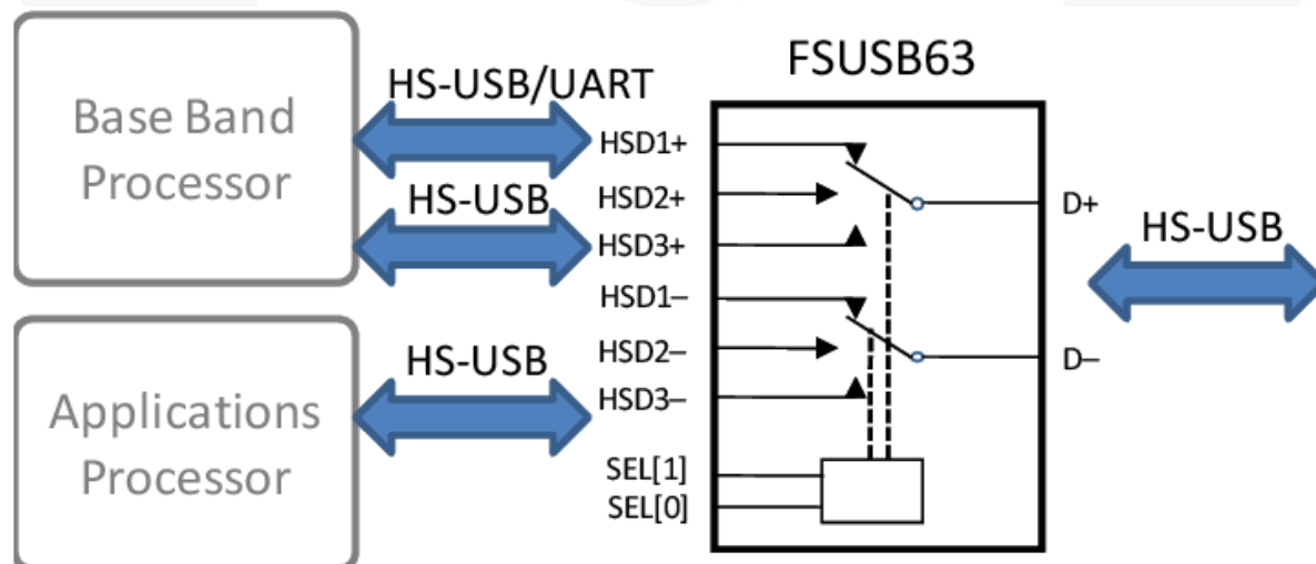
Figure 1. Analog Symbol
