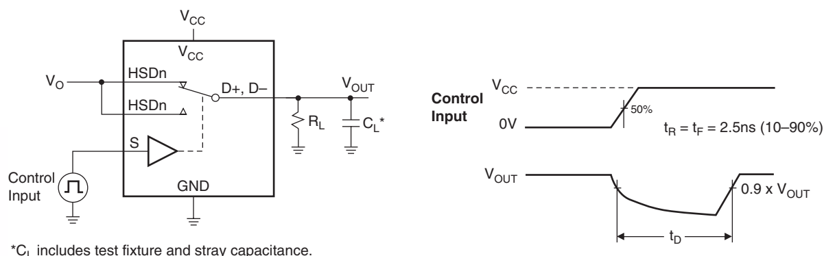
Figure 10. Break-Before-Make ( t_{BBM} )
