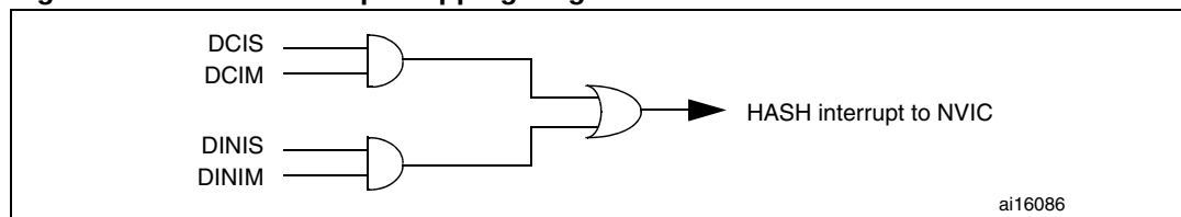
Figure 209. HASH interrupt mapping diagram
