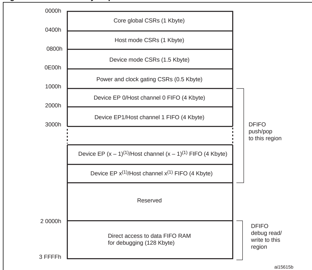
Figure 371. CSR memory map
