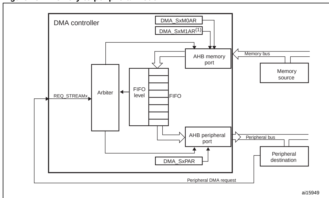
Figure 25. Memory-to-peripheral mode
