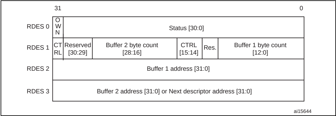
Figure 339. Normal Rx DMA descriptor structure
