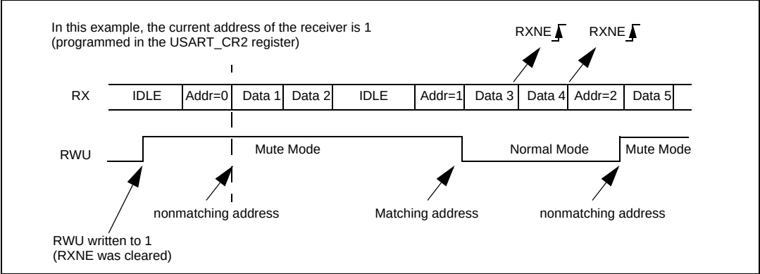
Figure 225. Mute mode using address mark detection
