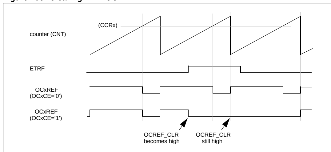
Figure 103. Clearing TIMx OCxREF
