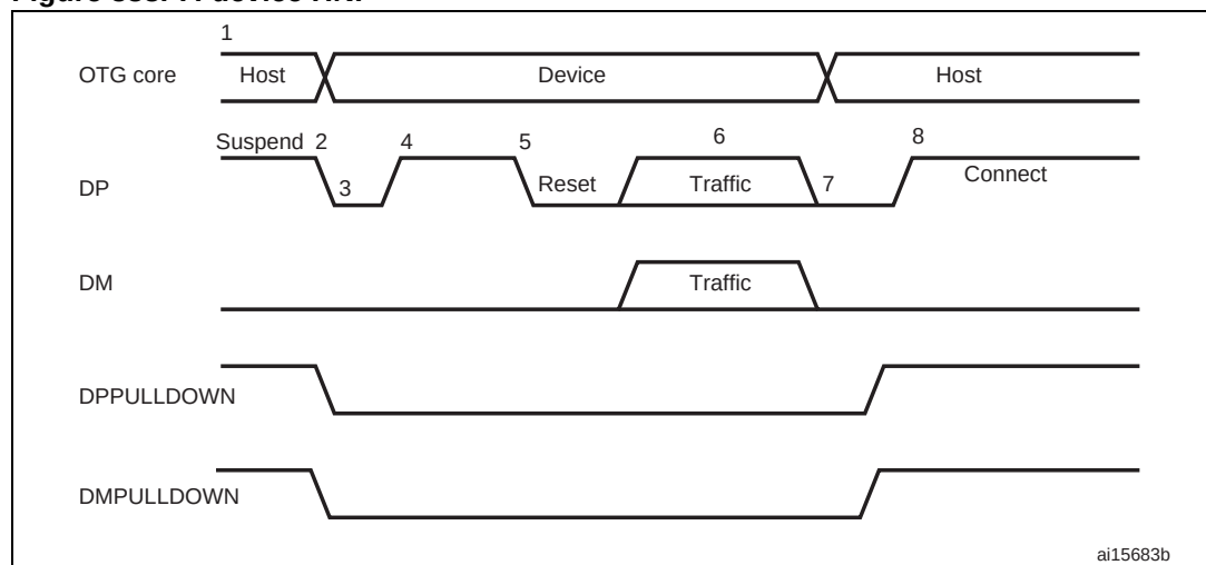
Figure 388. A-device HNP
