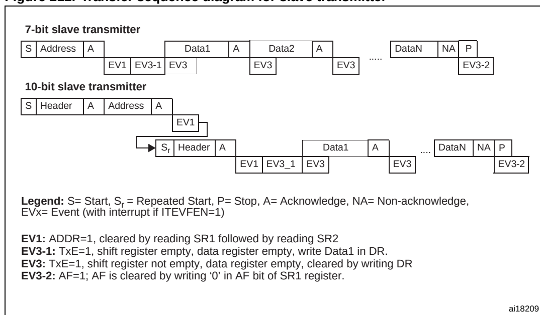
Figure 212. Transfer sequence diagram for slave transmitter
