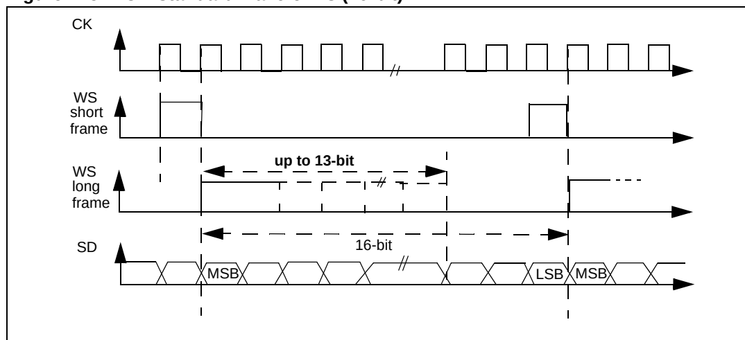
Figure 275. PCM standard waveforms (16-bit)
