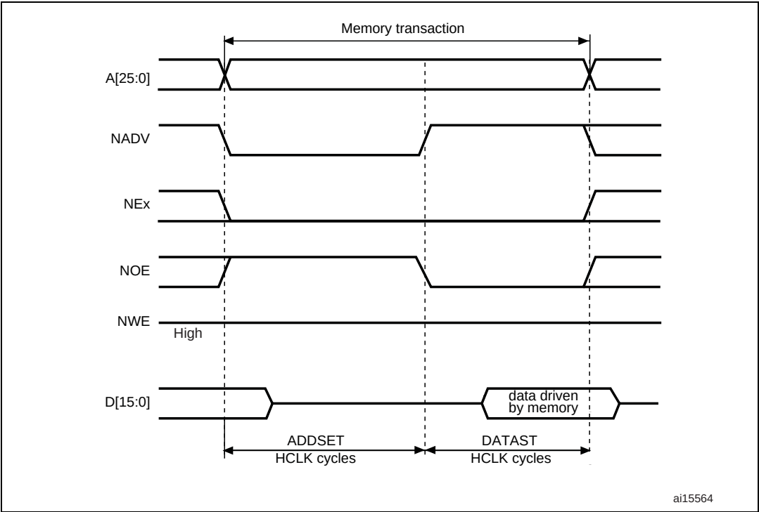
Figure 399. ModeC read accesses
