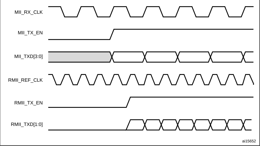
Figure 322. Frame transmission in MMI and RMII modes
