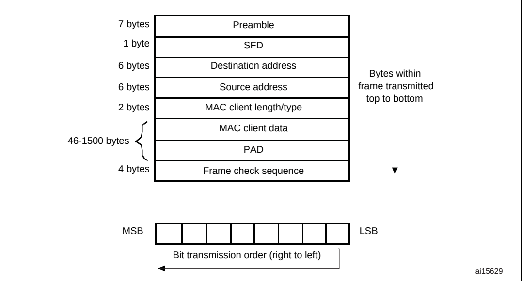
Figure 317. MAC frame format
