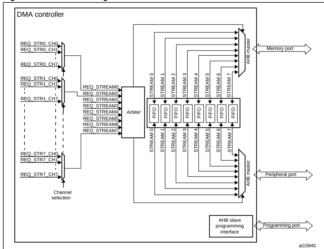
Figure 21. DMA block diagram
