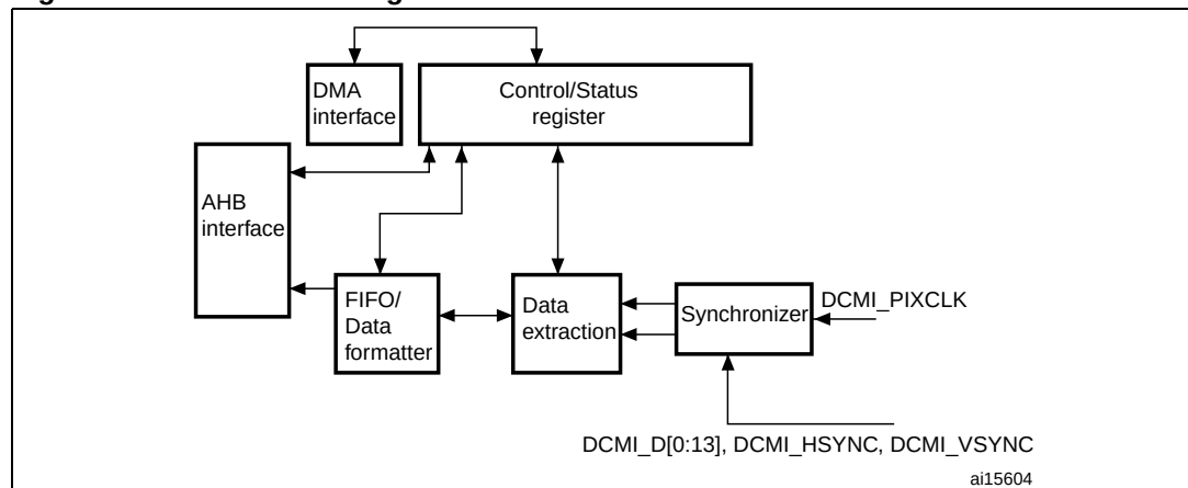
Figure 57. Top-level block diagram
