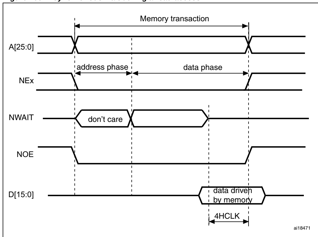
Figure 405. Asynchronous wait during a read access
