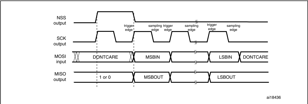
Figure 248. TI mode - master mode, single transfer
