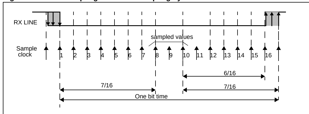
Figure 222. Data sampling when oversampling by 16
