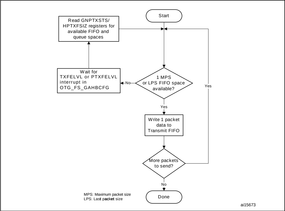
Figure 372. Transmit FIFO write task
