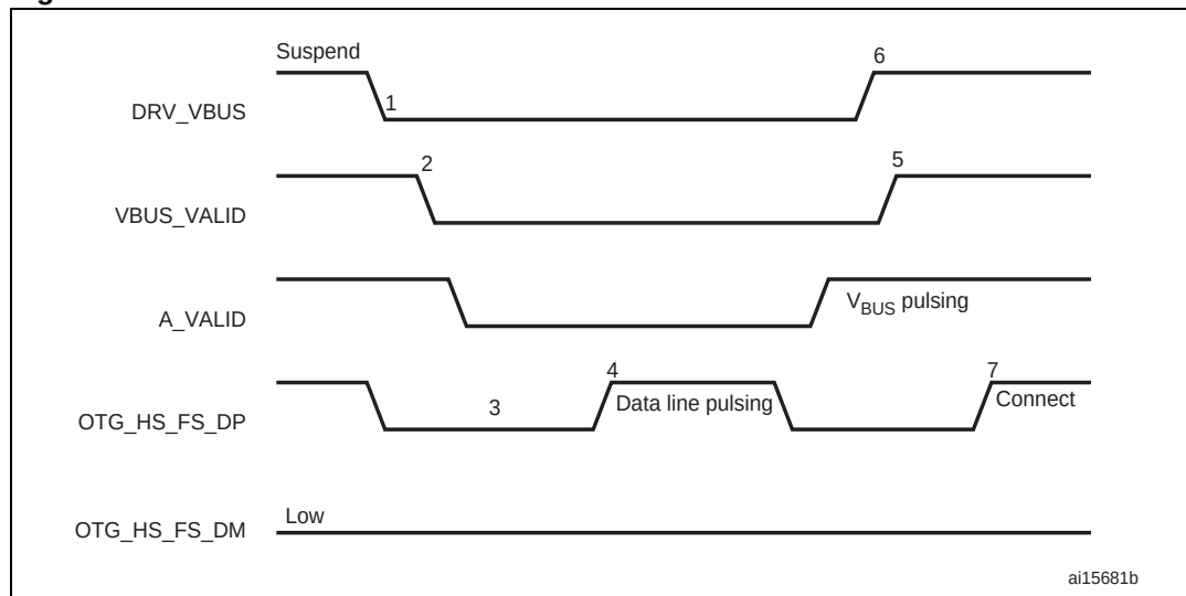
Figure 386. A-device SRP
