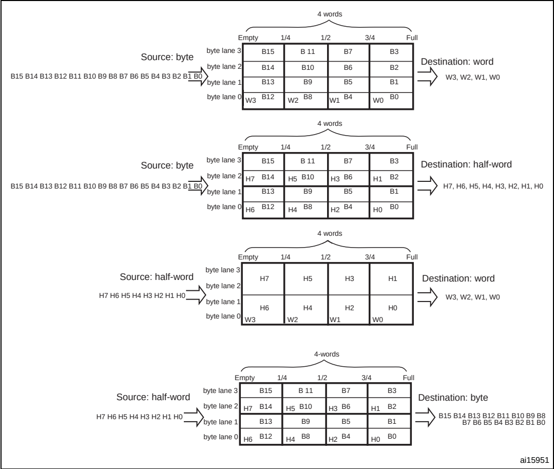
Figure 27. FIFO structure
