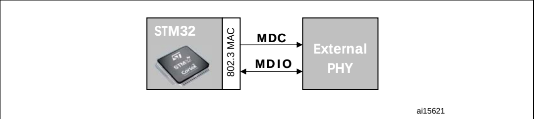
Figure 308. SMI interface signals
