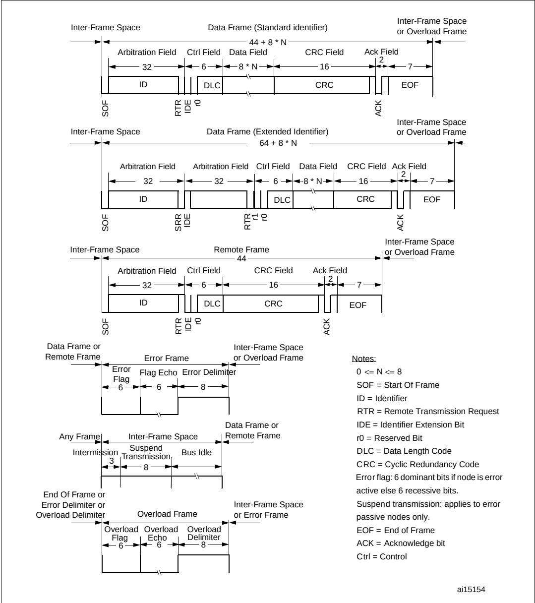
Figure 305. CAN frames
