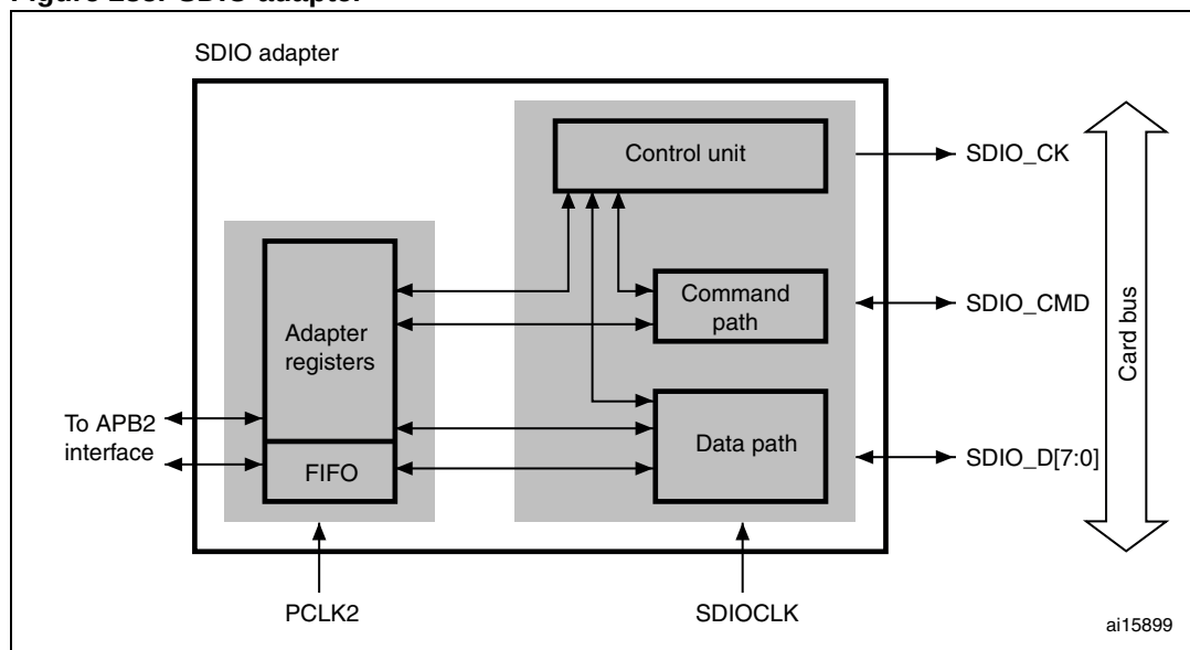
Figure 285. SDIO adapter
