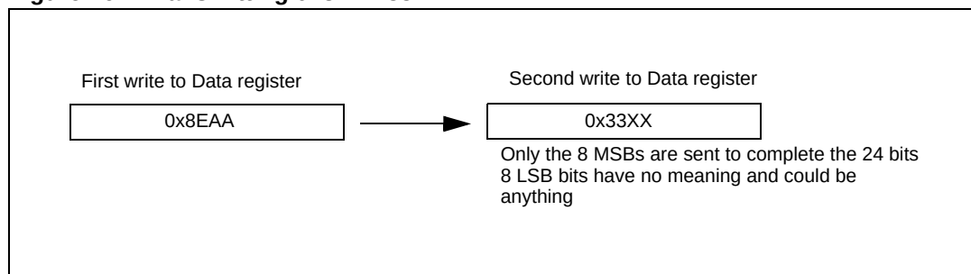
Figure 262. Transmitting 0x8EAA33
