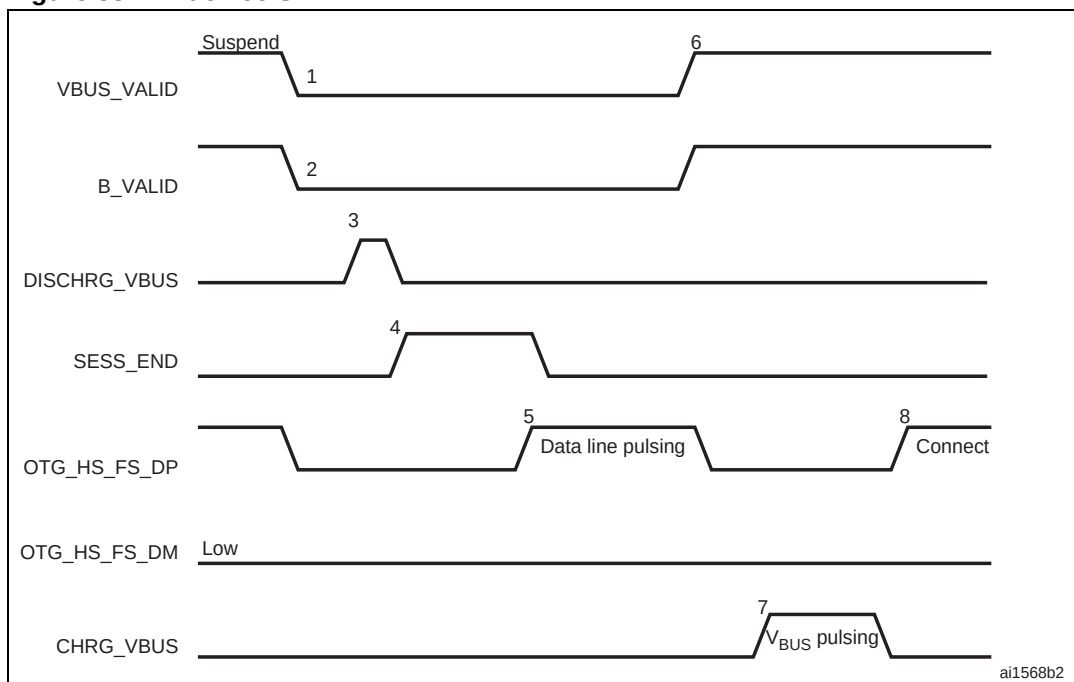
Figure 387. B-device SRP
