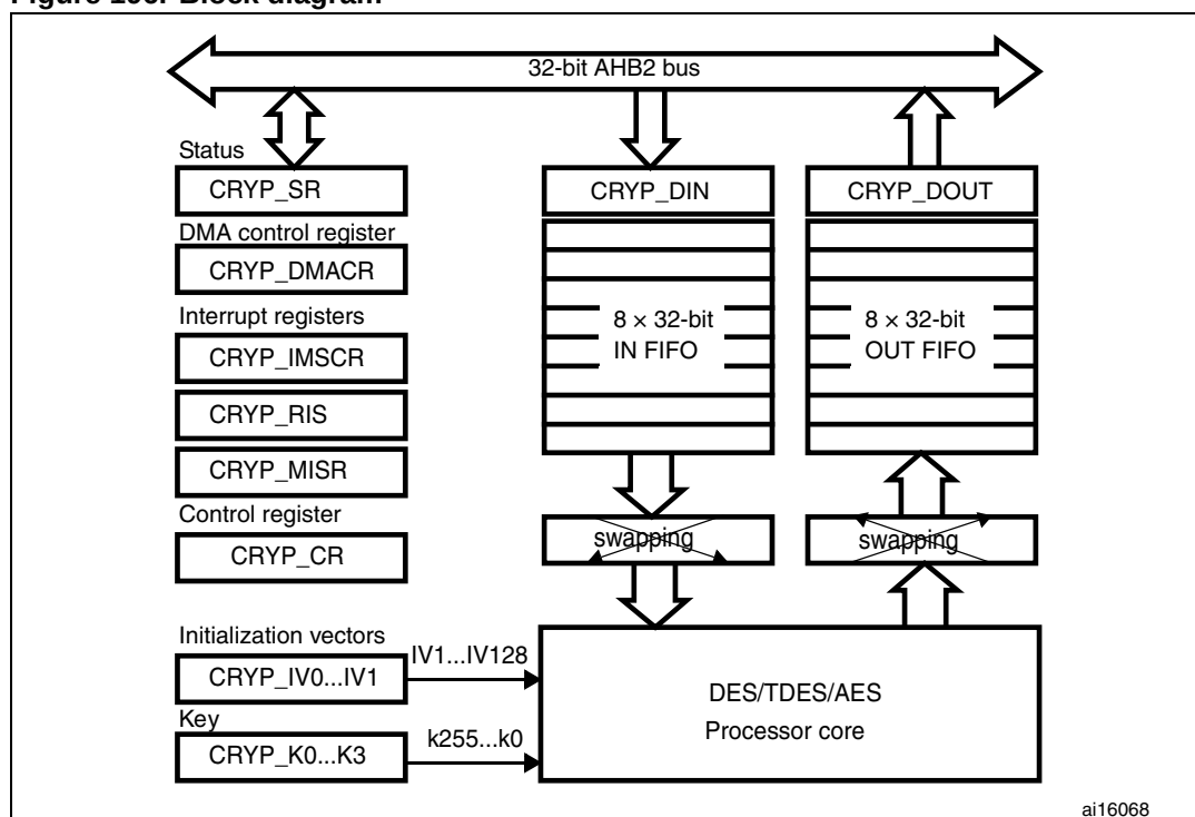
Figure 196. Block diagram
