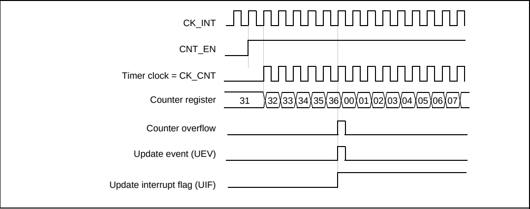
Figure 116. Counter timing diagram, internal clock divided by 1
