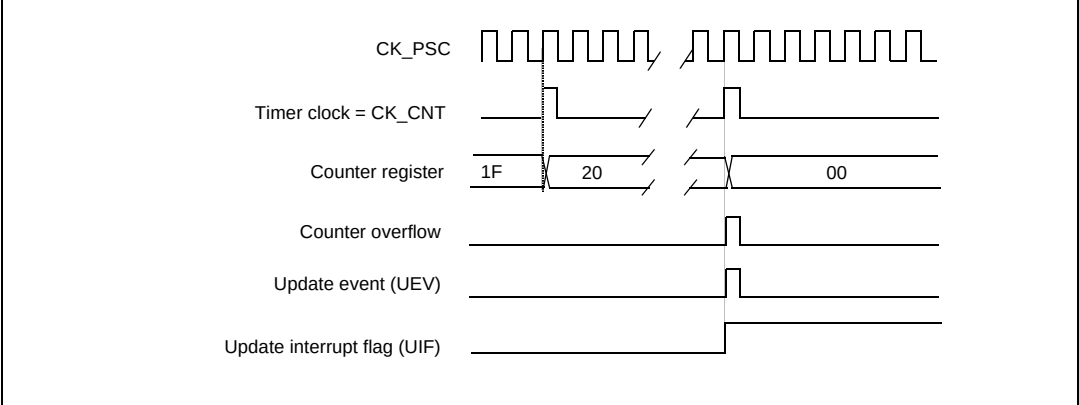
Figure 166. Counter timing diagram, internal clock divided by N
