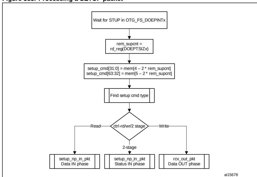
Figure 383. Processing a SETUP packet
