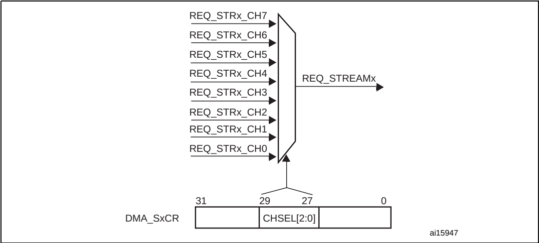
Figure 23. Channel selection
