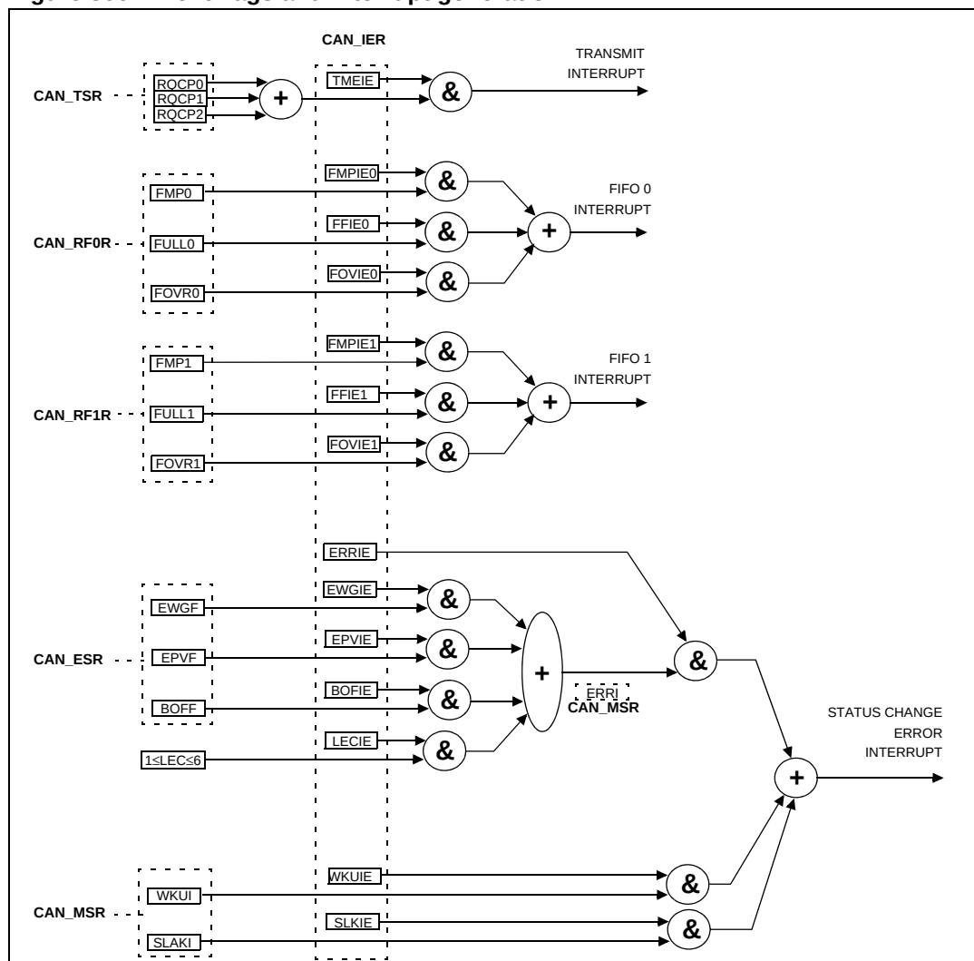
Figure 306. Event flags and interrupt generation
