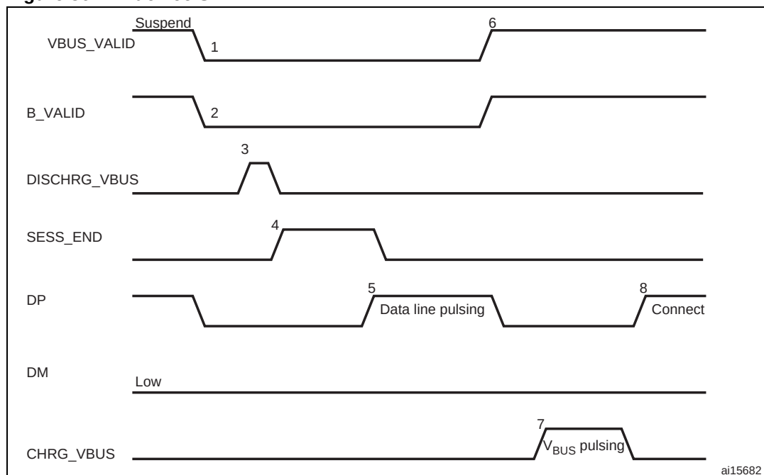
Figure 364. B-device SRP
