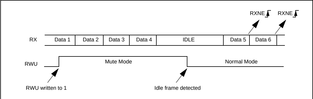
Figure 224. Mute mode using Idle line detection
