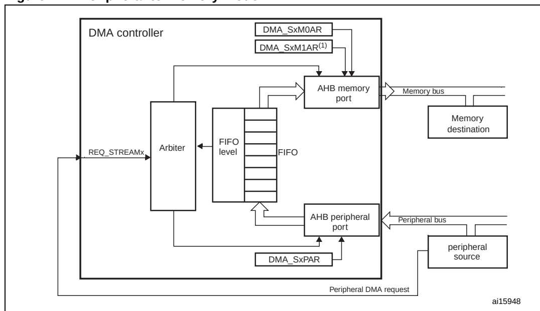
Figure 24. Peripheral-to-memory mode
