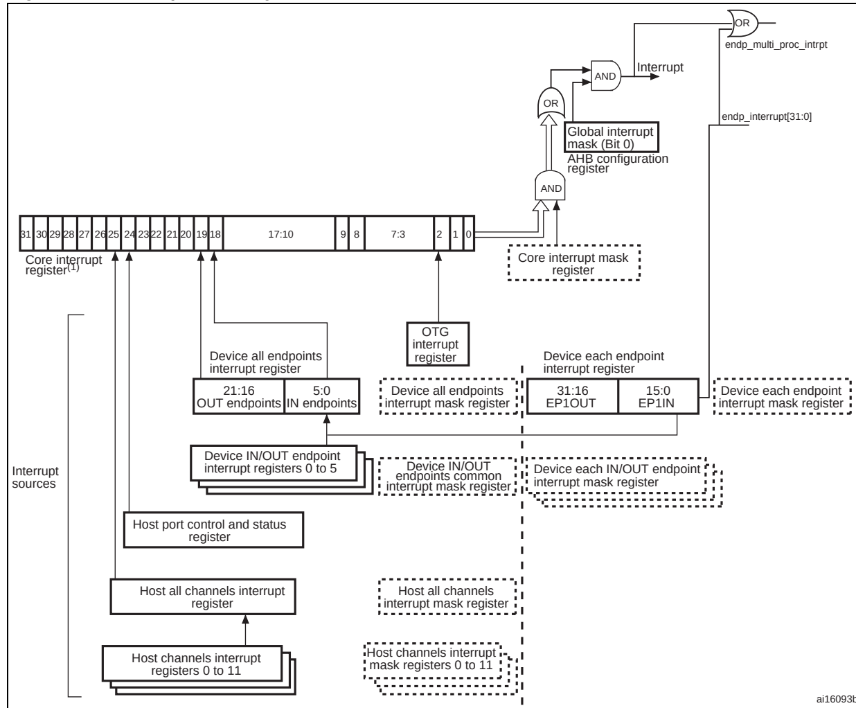
Figure 370. Interrupt hierarchy
