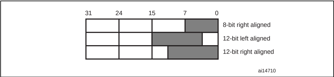
Figure 49. Data registers in single DAC channel mode
