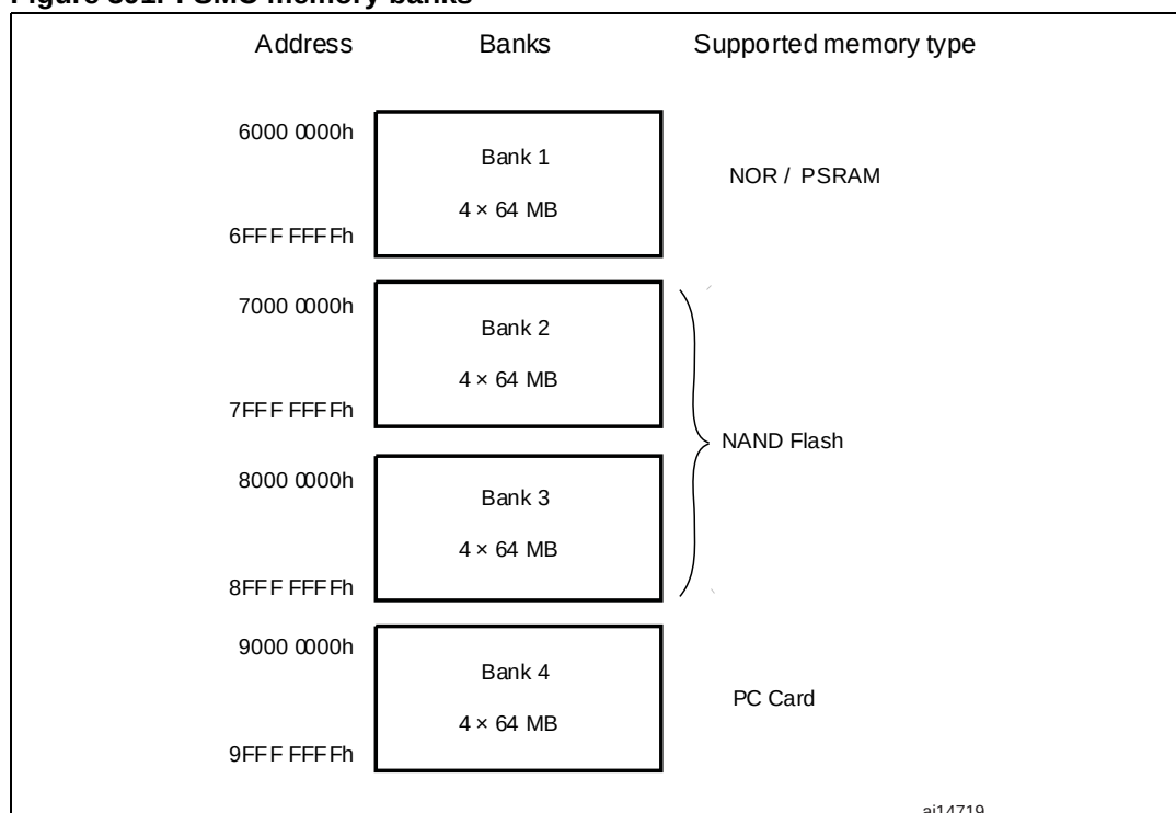
Figure 391. FSMC memory banks
