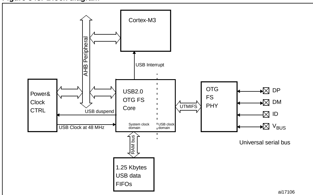
Figure 343. Block diagram
