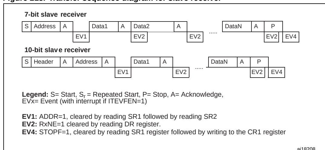
Figure 213. Transfer sequence diagram for slave receiver
