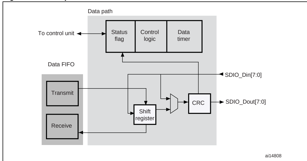
Figure 290. Data path
