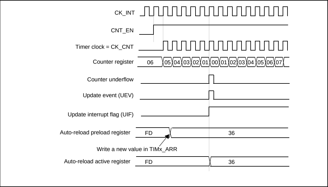
Figure 131. Counter timing diagram, Update event with ARPE=1 (counter underflow)
