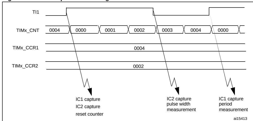
Figure 95. PWM input mode timing
