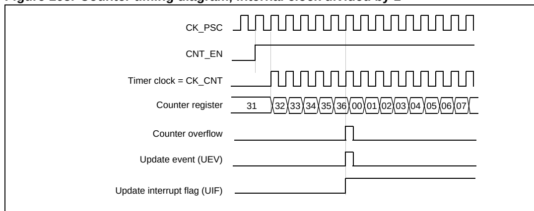
Figure 163. Counter timing diagram, internal clock divided by 1
