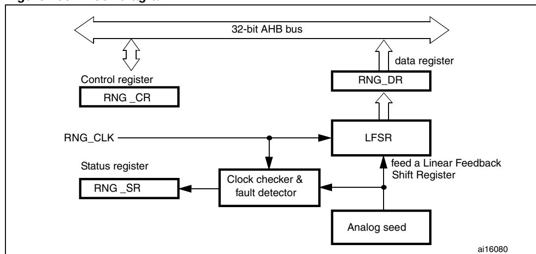
Figure 206. Block diagram
