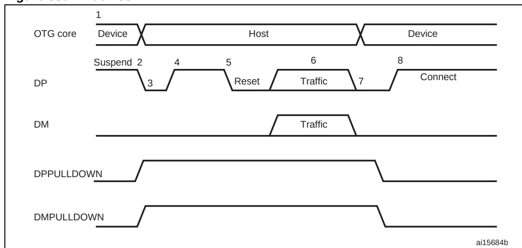
Figure 389. B-device HNP
