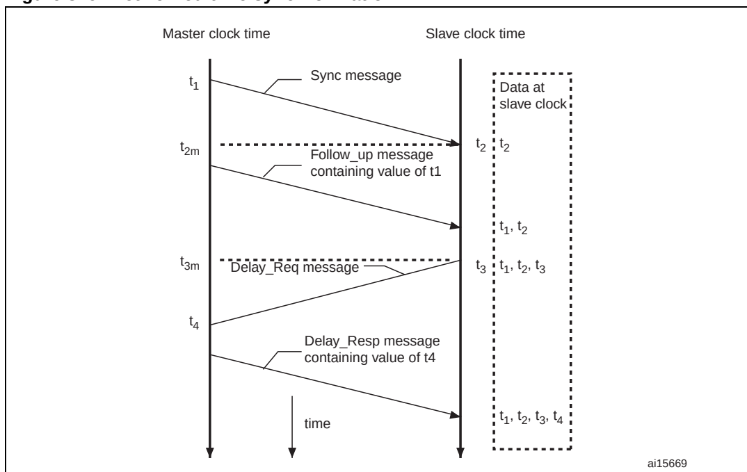
Figure 329. Networked time synchronization
