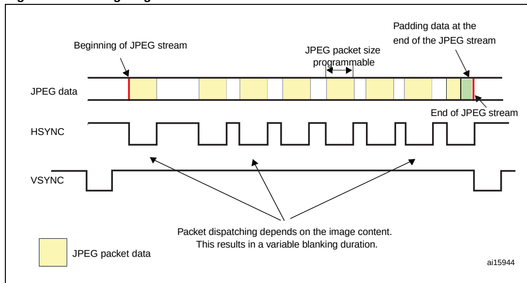
Figure 59. Timing diagram
