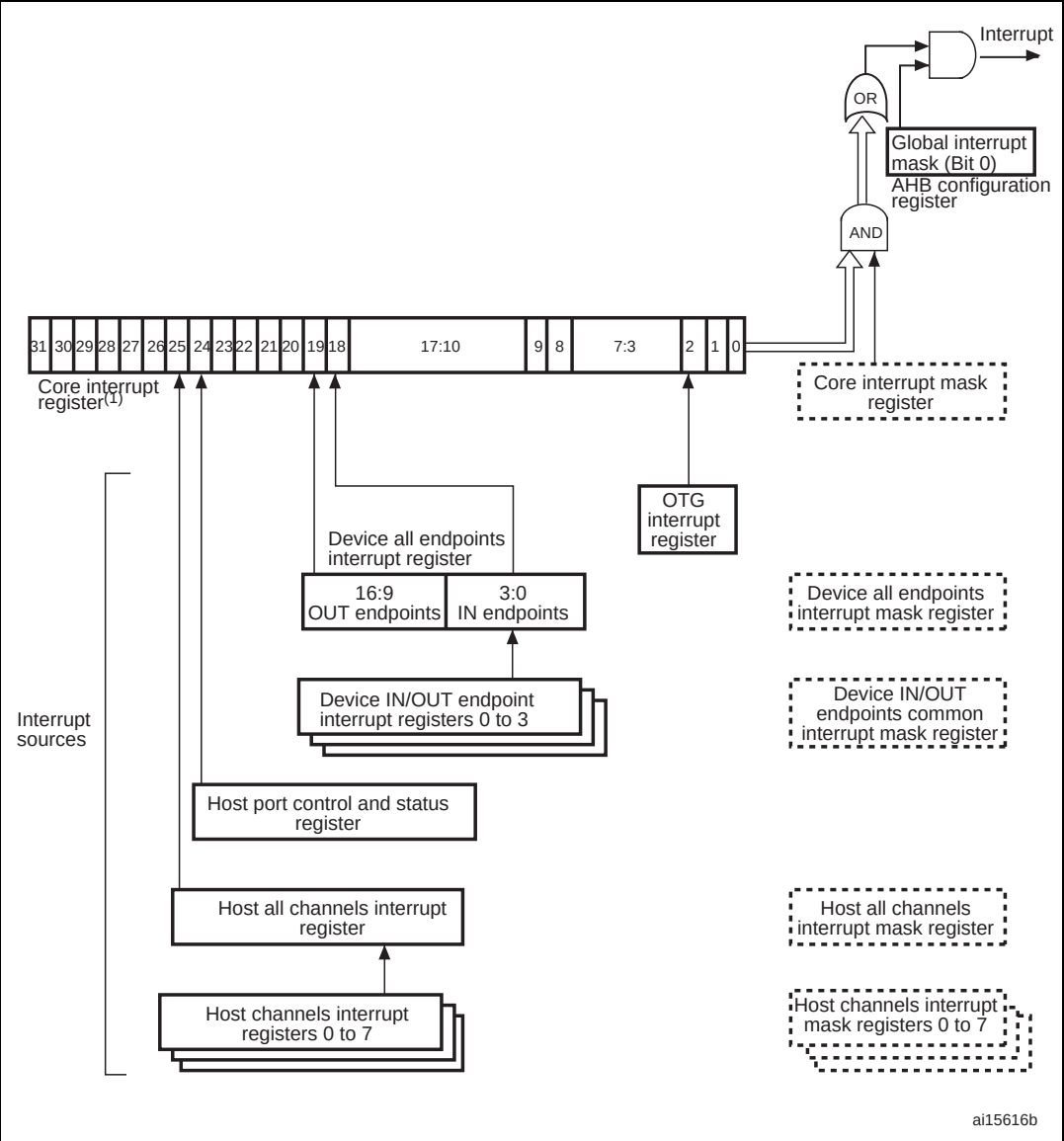
Figure 351. Interrupt hierarchy
