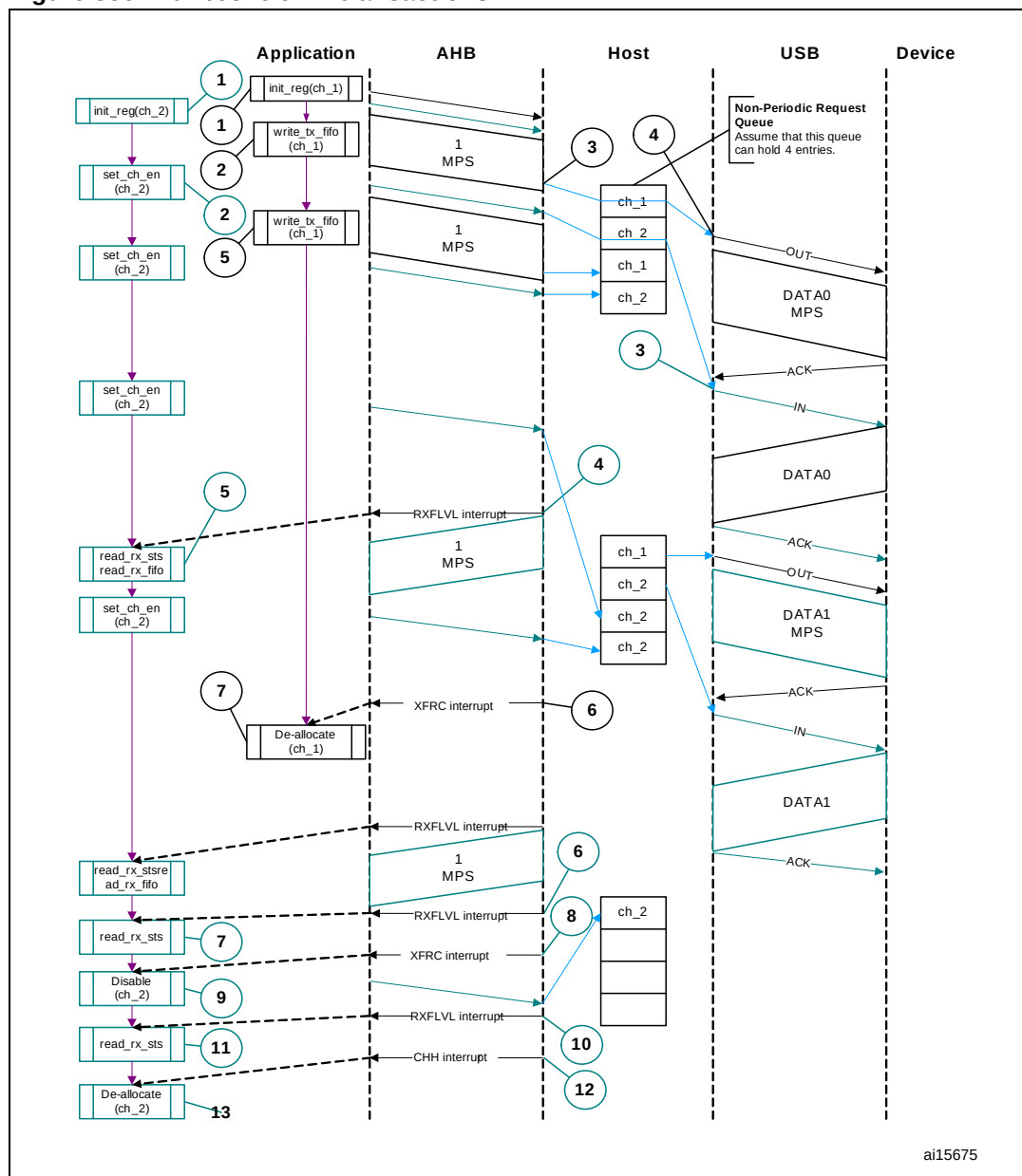
Figure 356. Bulk/control IN transactions
