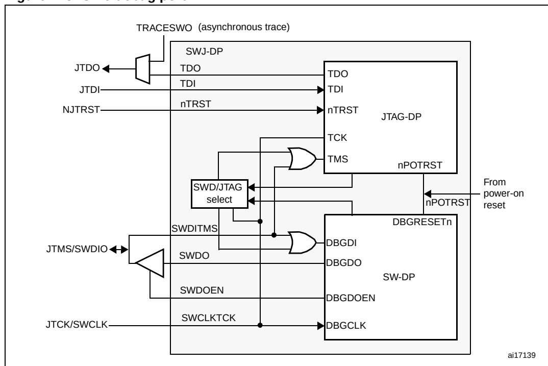
Figure 413. SWJ debug port
