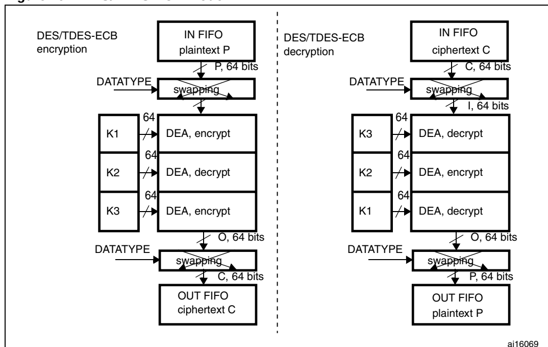
Figure 197. DES/TDES-ECB mode
