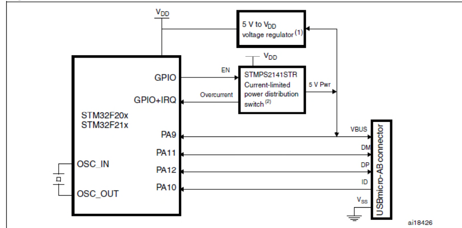
Figure 344. OTG A-B device connection
