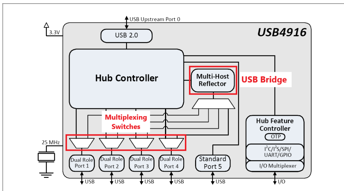
FIGURE 2-1: INTERNAL BLOCK DIAGRAM
