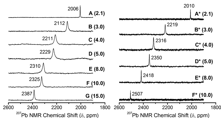
Figure 4. ^{207}\text{Pb} NMR spectra of the alkaline aqueous lead(II) cysteine solutions A–G enriched in ^{207}\text{Pb} ( C_{\text{Pb}^{\text{II}}} = 10 \text{ mM} ; \text{H}_2\text{Cys}/\text{Pb}^{2+} mole ratios 2.1–15.0) and A*–F* with 10% \text{D}_2\text{O} ( C_{\text{Pb}^{\text{II}}} = 100 \text{ mM} ; \text{H}_2\text{Cys}/\text{Pb}^{2+} mole ratios 2.1–10.0).
