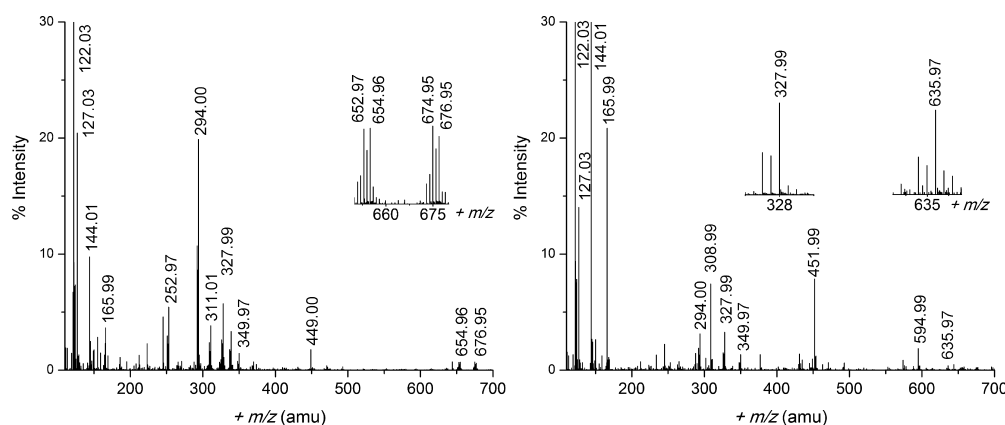
Figure 1. ESI-MS spectra measured in positive-ion mode for solutions A (left) and F (right) ( C_{\text{Pb}^{II}} = 10 mM) with \text{H}_2\text{Cys}/\text{Pb}^{II} mole ratios 2.1 and 10.0, respectively. The peak at 122.03 amu has 100% intensity. Selected peaks assigned to lead(II) species with distinct isotopic patterns for Pb are shown in the inset.
