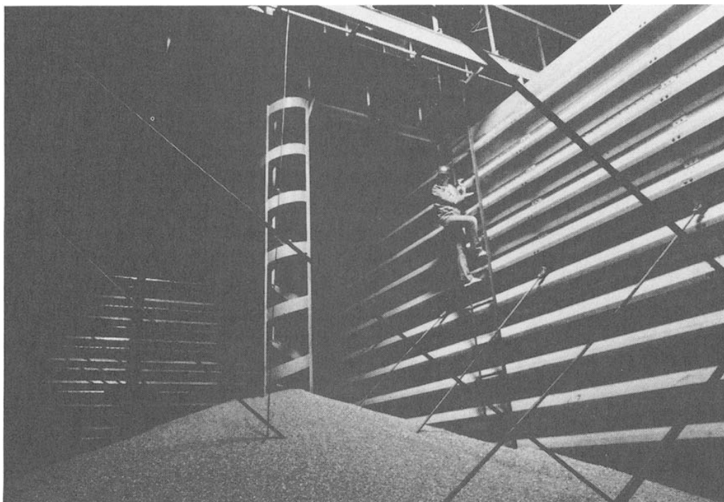
Fig. 9-11. Bulk seed in storage awaiting further conditioning and bagging. The spiral chute permits filling the bin while subjecting the seed to minimal mechanical injury.
