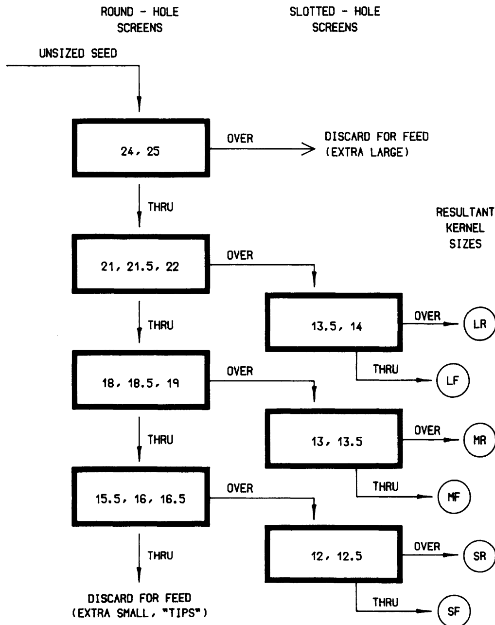
Fig. 9-12. A diagrammatic outline of typical screen sizes used for sizing seed corn, using round-hole screens first and then dividing each portion (large, medium, and small) into flat and round kernels with slotted-hole screens. Screen sizes are given in 64ths of an inch.
