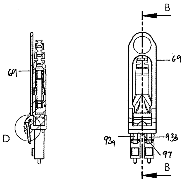
SECTION B-B - Latched
