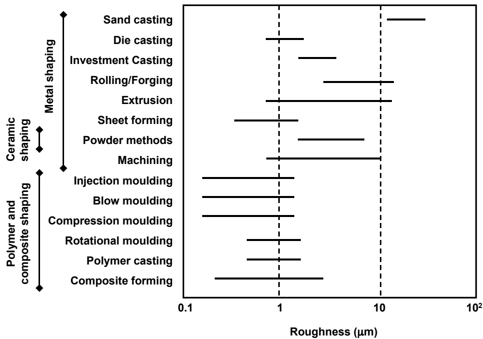
Figure 4.4: Process attribute chart for shaping processes: surface roughness ( \mu\text{m} )
