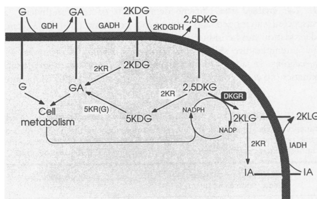
Fig. 1. Summary of the enzymes, intermediates, and by-products encountered in the synthesis of 2-keto-L-gulononic acid (2-KLG) from glucose in genetically engineered E. herbicola . The control of cloned (white printing on black) 2,5-DKG reductase activity, which requires the reduced form (NADPH) of nicotinamide adenine dinucleotide phosphate (NADP) supplied by the cell metabolism, directs metabolite flow to 2-KLG. Wide band with dots, cell membrane; straight bars, transport systems. Abbreviations are as follows: GDH, D-glucose dehydrogenase; GADH, D-gluconate dehydrogenase; 2KDGDH, 2-keto-D-gluconate dehydrogenase; 2KR, 2-keto-D-gluconate reductase; DKGR, 2,5-diketo-D-gluconate reductase; IADH, L-idonate dehydrogenase; 5KR(G), 5-keto-D-gluconate reductase (D-gluconate-producing); G, D-glucose; GA, D-gluconate; 2KDG, 2-keto-D-gluconate; 2,5DKG, 2,5-diketo-D-gluconate; IA, L-idonate; and 5KDG, 5-keto-D-gluconate. Reprinted by permission from (21).
