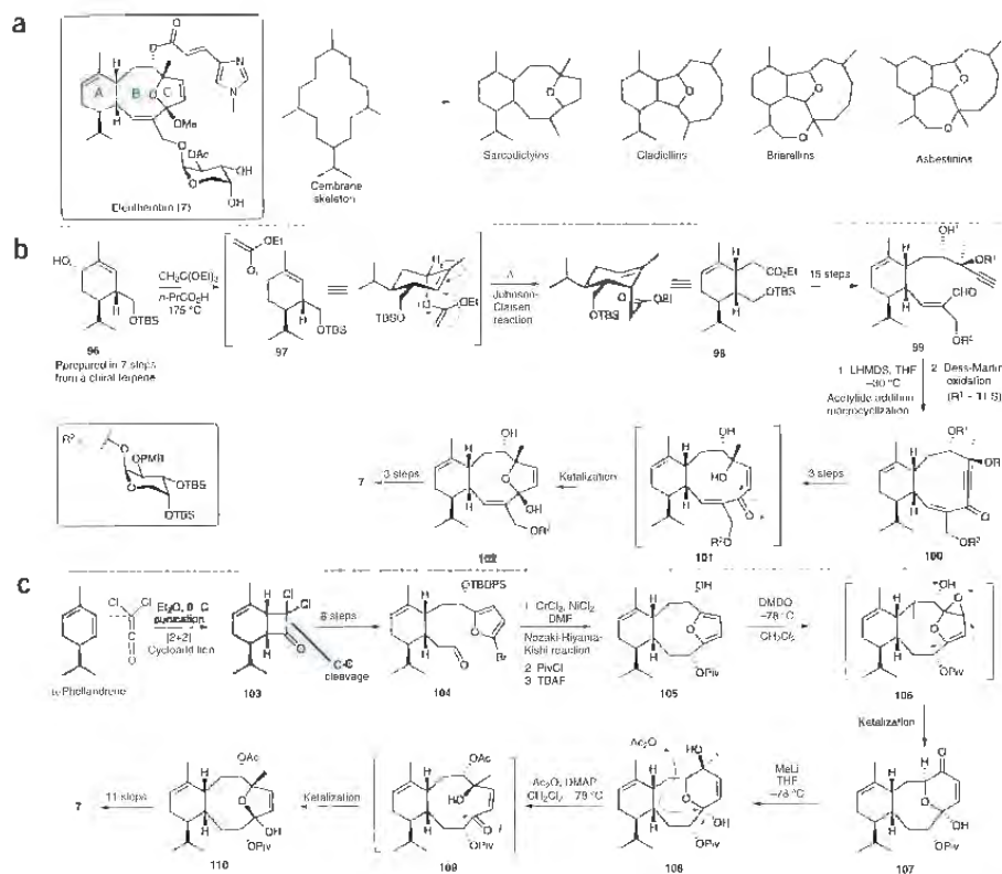
Scheme 7 Total synthesis of eleutherobin. (a) Eleutherobin's cerambrane-derived skeleton makes it a member of the sarcodictyin family, and it is presumably related to several other large classes of diterpenes. (b) Key steps in Nicolaou's synthetic route to eleutherobin. The A ring was derived from a commercially available terpene and the macrocycle was formed by an intramolecular acetylide addition. (c) Key steps in Danishefsky's total synthesis of eleutherobin. An intramolecular Nozaki-Hiyama-Kishi coupling was used to construct the B ring. Furan 106 underwent an Achmatowicz ring expansion and ketalization ring contraction to form the core structure ( 110 ). Ac, acetyl; DMAP, N,N -dimethylaminopyridine; DMDQ, 2,2-dimethyldioxirane; LHMDs, lithium hexamethyldisilazide; PMB, p -methoxybenzyl; Piv, pivaloyl; TBAF, tetrabutylammonium fluoride; TBDPS, t -butyldiphenylsilyl; TBS, t -butyldimethylsilyl; TES, triethylsilyl.
