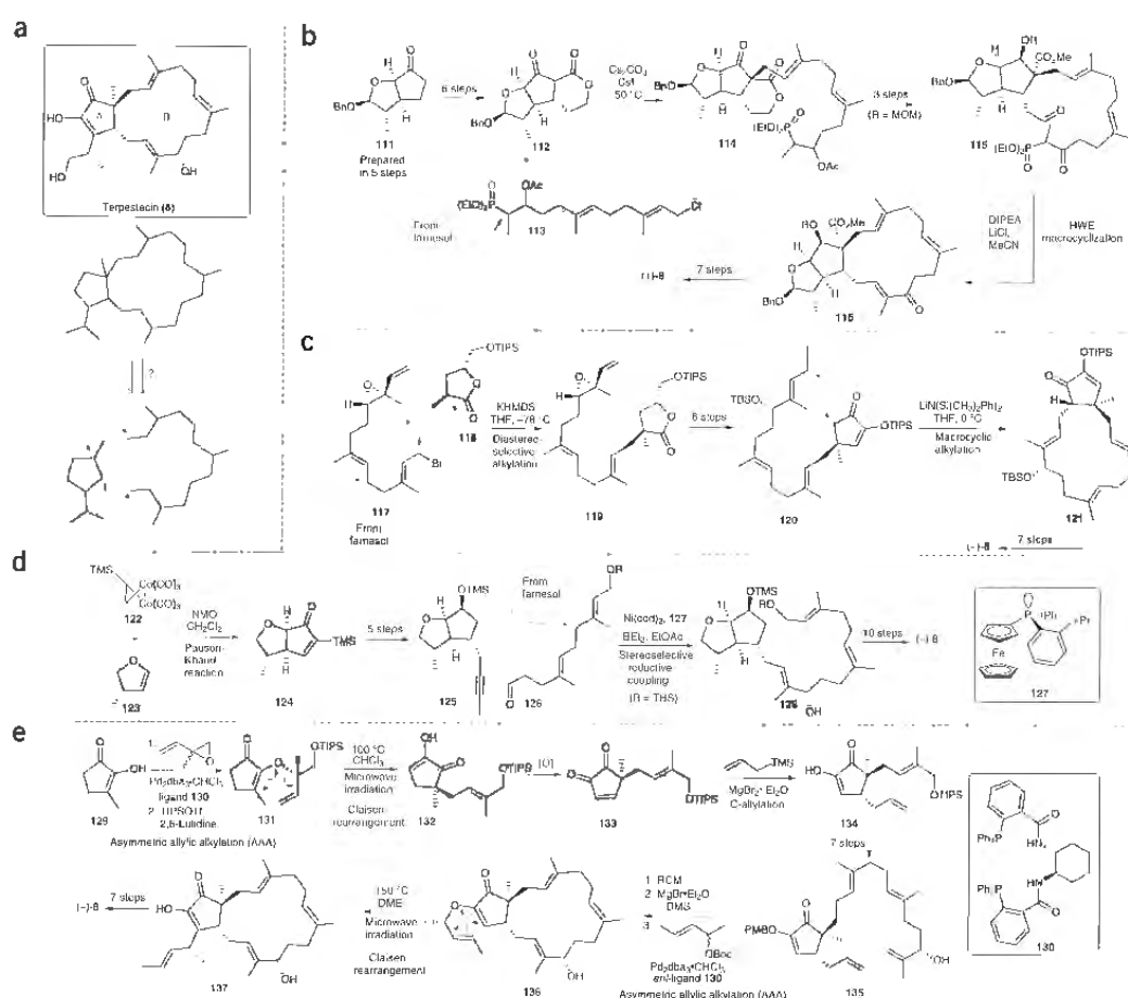
Scheme 8 Total syntheses of terpestacin. (a) Macrocyclization as a key synthetic challenge posed by the anti-HIV agent terpestacin. (b) A Horner-Wadsworth-Emmons (HWE) macrocyclic olefination en route to terpestacin (Tatsuta). (c) Use of an easily prepared chiral lactone to control the stereochemistry of the critical quaternary center en route to (–)-terpestacin (Myers). (d) Use of a stereoselective, regioselective nickel-catalyzed reductive coupling between an aldehyde and alkyne en route to terpestacin (Jamison). (e) Trost's synthesis of terpestacin. Two of the four stereocenters were constructed using an asymmetric allylic alkylation (AAA) and Claisen rearrangement protocol. Ac, acetyl; Bn, benzyl; Boc, t -butoxycarbonyl; cod, cyclooctadiene; dba, dibenzylideneacetone; DIPEA, diisopropylethylamine; DME, 1,2-dimethoxyethane; DMS, dimethyl sulfide; KHMDS, potassium hexamethyldisilazide; LDA, lithium diisopropylamide; MOM, methoxymethylene; NMO, N -methylmorpholine N -oxide; [O], oxidation; PMB, p -methoxybenzyl; RCM, ring-closing metathesis; TBS, t -butyldimethylsilyl; TIPS, triisopropylsilyl; TMS, trimethylsilyl.
