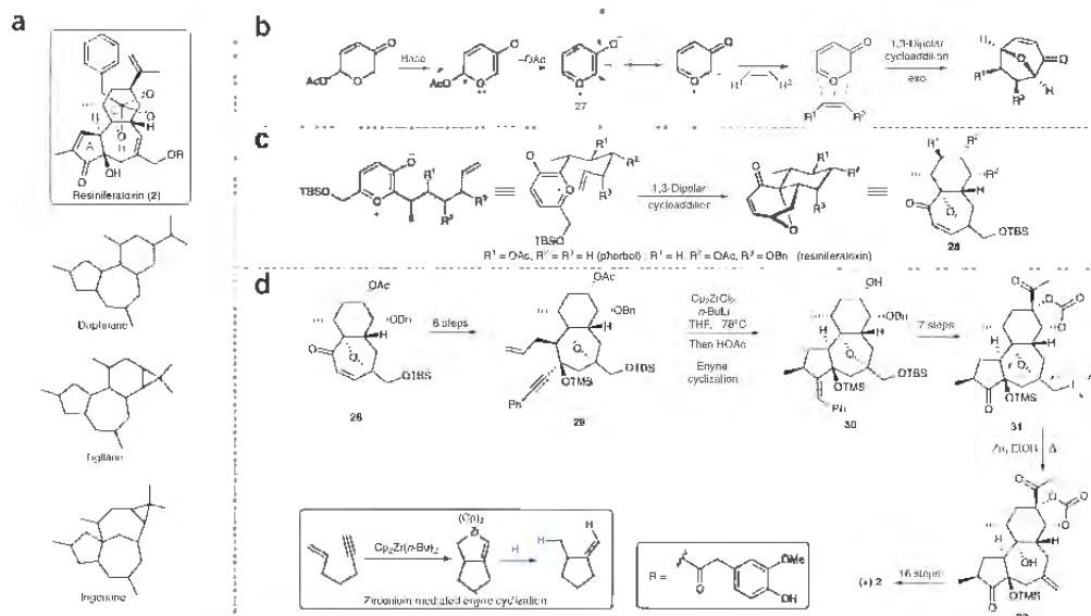
Scheme 2 Synthetic methods used in the construction of resiniferatoxin. (a) Resiniferatoxin's daphnane skeleton and its close chemical relatives, also from the plant family Euphorbiaceae. (b) General method for the generation of a reactive oxidopyrylium ( 27 ) and its subsequent participation in an exo-selective 1,3-dipolar cycloaddition. (c) Use of an intramolecular oxidopyrylium cycloaddition as an efficient synthetic entry into the tigliane and daphnane skeletons (Wender and colleagues). (d) Key transformations in Wender's pioneering total synthesis of resiniferatoxin. Ac, acetyl; Bn, benzyl; Cp, cyclopentadienyl; TBS, t-butyldimethylsilyl; THF, tetrahydrofuran; TMS, trimethylsilyl.
