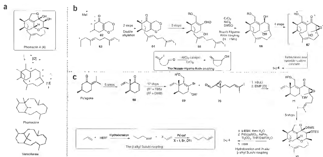
Scheme 4 Total syntheses of phomactin A. (a) Phomactin's unusual diterpene skeleton coupled with its high oxidation render it a formidable synthetic challenge. Also shown for comparison is the verticillane skeleton. (b) Pattenden's total synthesis featuring a Nozaki-Hiyama-Kishi macrocyclization. (c) β-alkyl Suzuki macrocyclization strategy used by Halcomb and co-workers. 9-BBN, 9-borabicyclo[3.3.1]nonane; DMB, 3,4-dimethoxybenzyl; DMSO, dimethylsulfoxide; DMP, Dess-Martin periodinane; PMB, p -methoxybenzyl; dppf, 1,1'-bis(diphenylphosphino)ferrocene; TBAF, tetrabutylammonium fluoride; TBS, t -butyldimethylsilyl; TES, triethylsilyl; Tf, trifluoromethane sulfonate; THF, tetrahydrofuran; TMS, trimethylsilyl.
