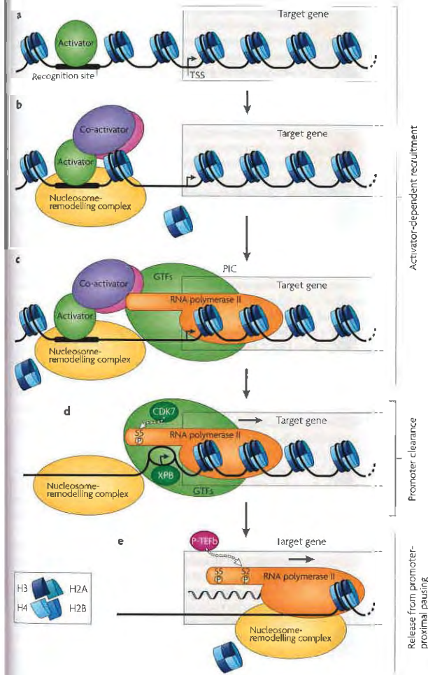
Figure 1 | Early steps in the transcription cycle.
