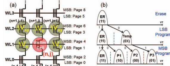
Fig. 1. (a) All-bit-line NAND flash architecture with victim cell circled in red and aggressor cells circled in grey; (b) Two-bit MLC flash programming scheme. Cell states are encoded in format (LSB, MSB)
