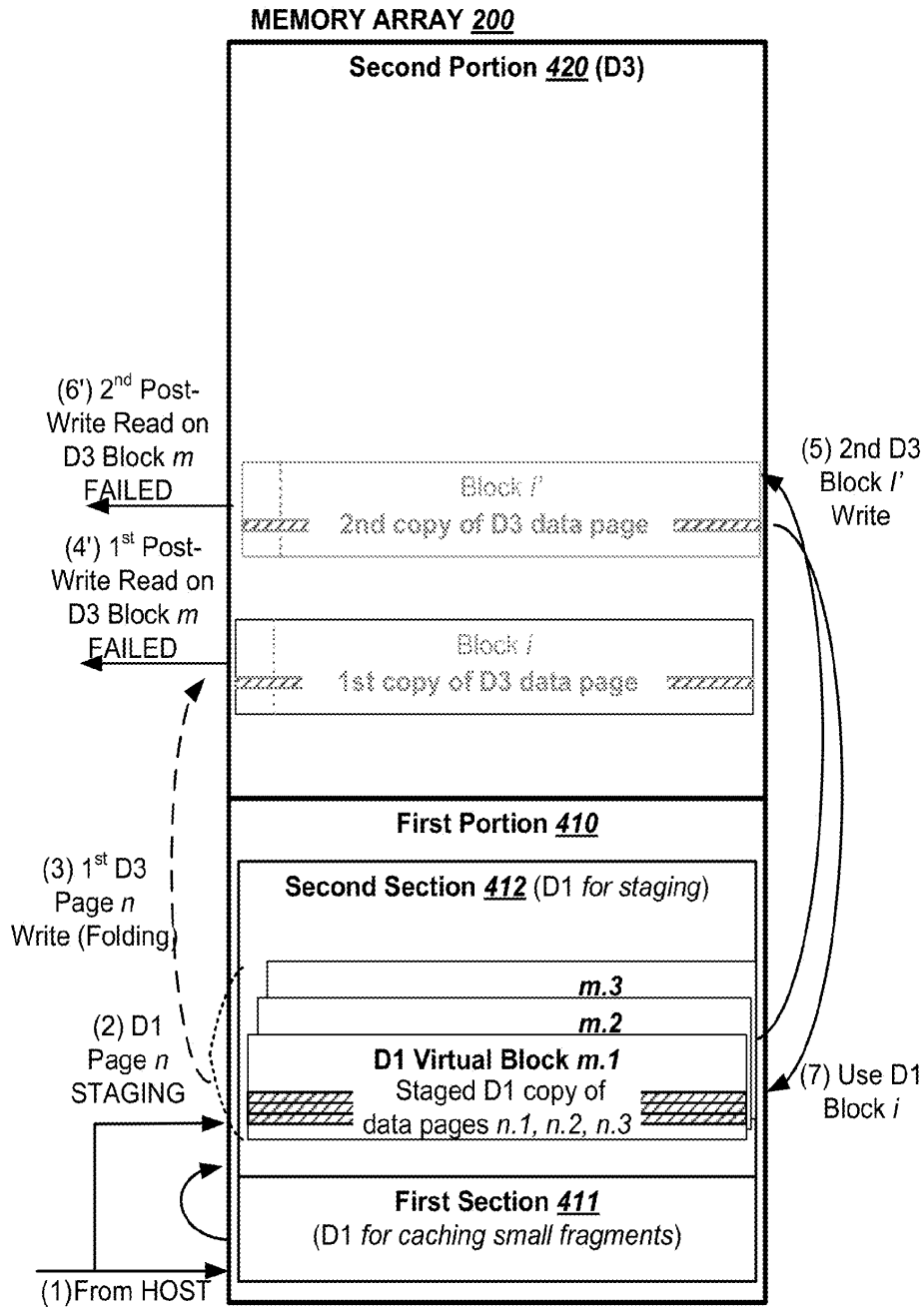
Example of Read Error after 2nd D1 to D3 Folding
