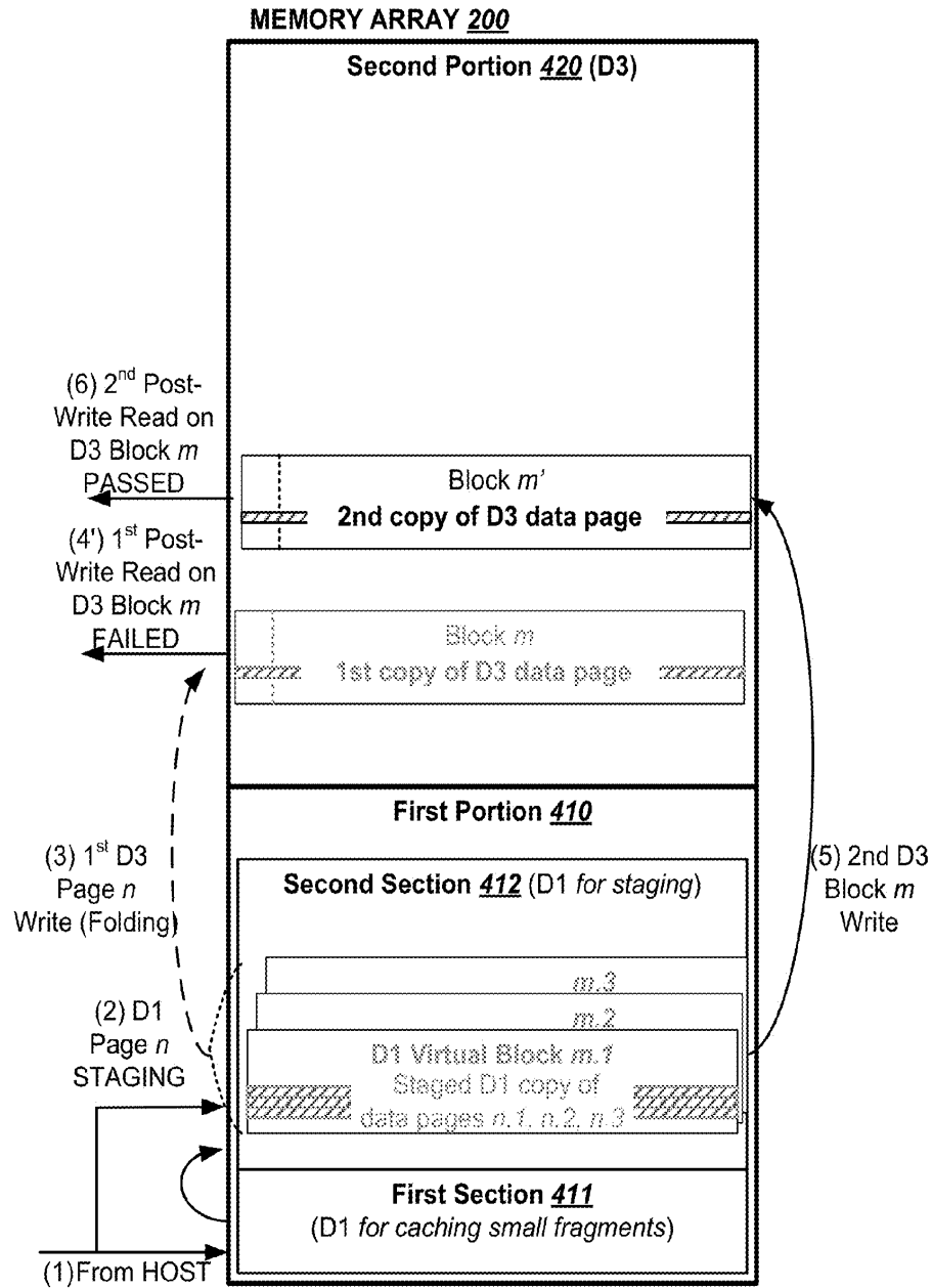
Example of Read Error after 1 st D1 to D3 Folding
