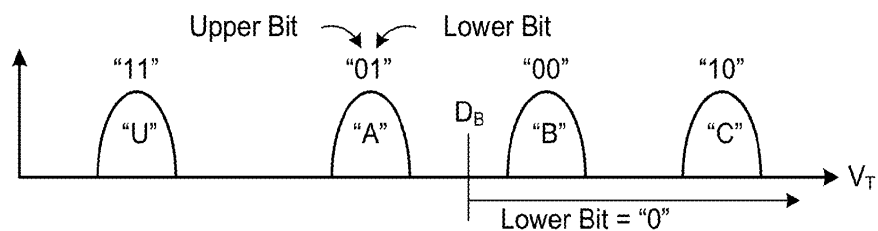
Lower Page Read (LM Gray Code)
