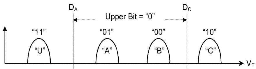
Upper Page Read (LM Gray Code)
