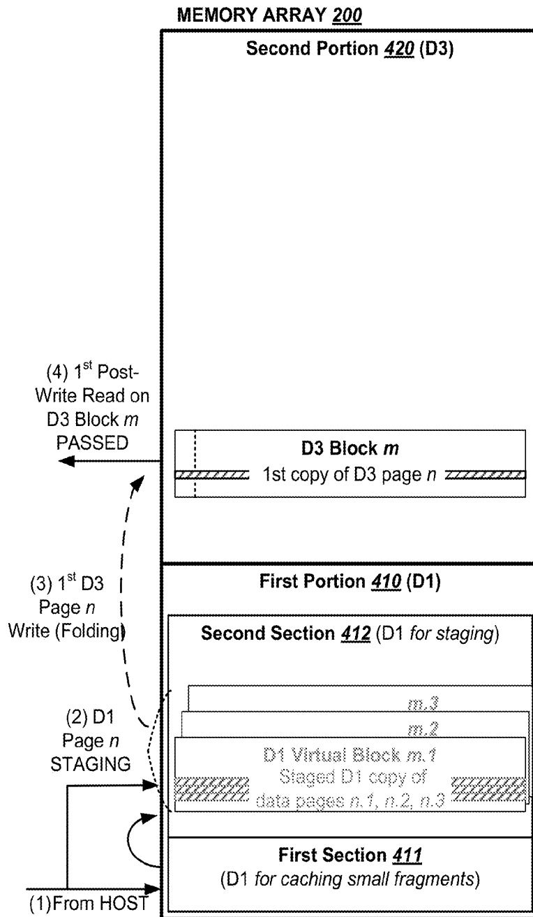
Example of successful D1 to D3 Folding
