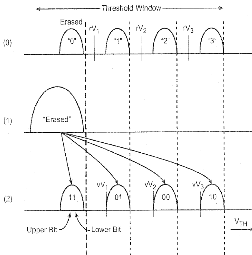
Programming into Four States Represented by a 2-bit Code
