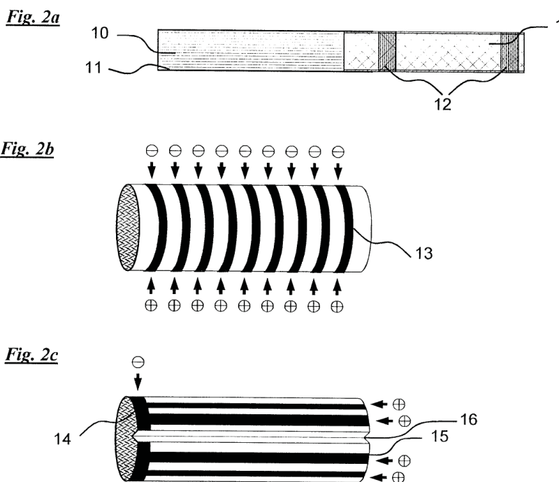
FIGS. 2a-2c.
