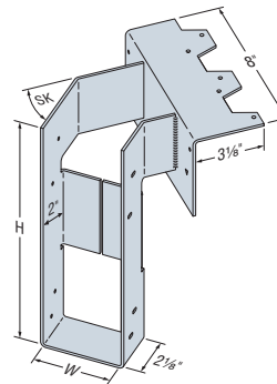
DGH3.62/11.88 Skewed Right Shown; All Others Similar
