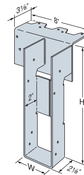
Top Flange Offset; Right Similar
