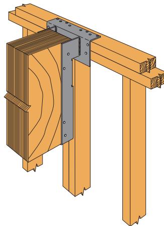
DGB Hanger Installed with Double Studs
