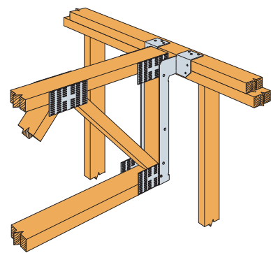
DG Hanger on Stud Wall with Trusses
