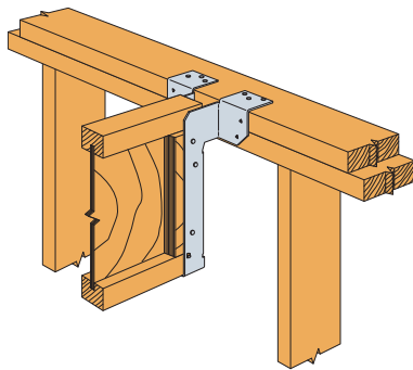
DG Hanger on Stud Wall with I-Joists
