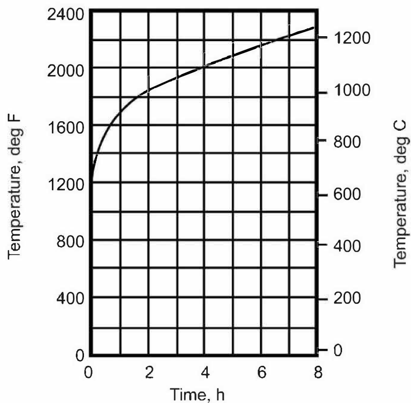
Figure 6 ASTM E 119 Time temperature curve
