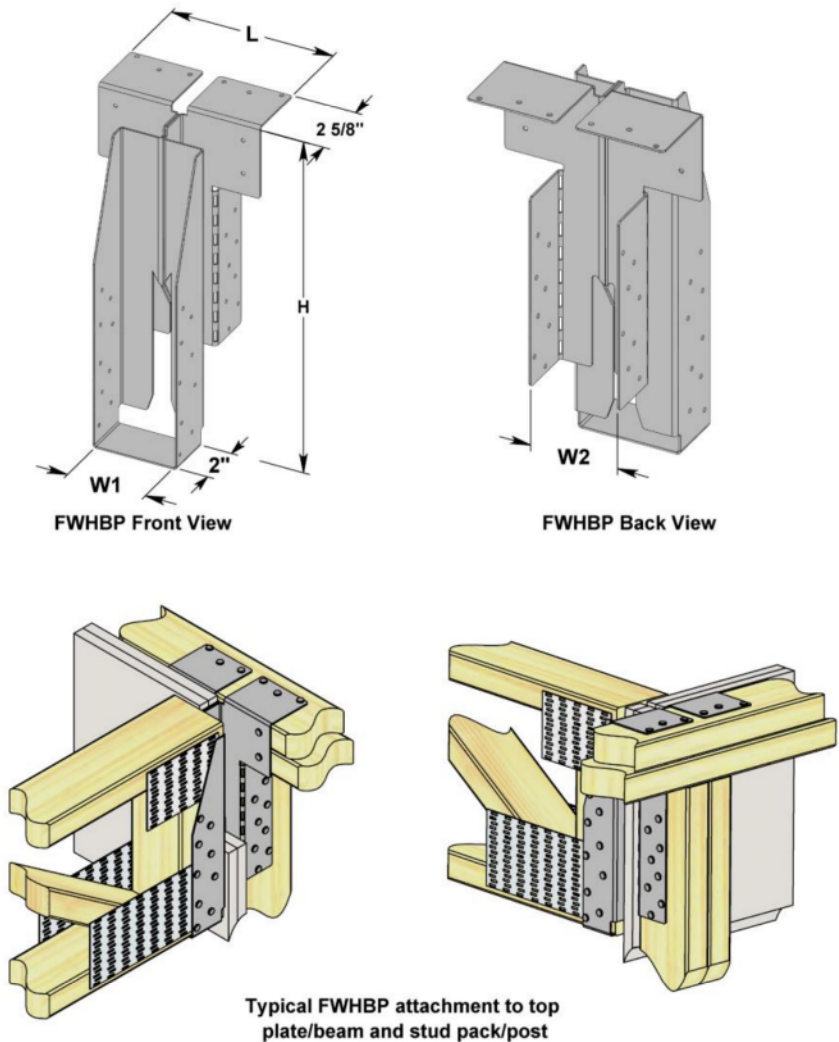
FIGURE 2—FWHBP FIRE WALL HANGER AND TYPICAL INSTALLATION
