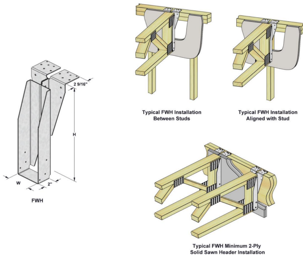
FIGURE 1—FWH TOP MOUNT FIRE WALL HANGER AND TYPICAL INSTALLATIONS ON STUD WALL AND SOLID SAWN HEADER
