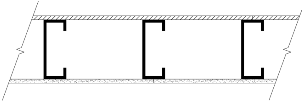
FIG. X7.4 Cold Formed Steel Floor Specimen
