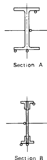
FIG. 4 Typical Location of Thermocouple
