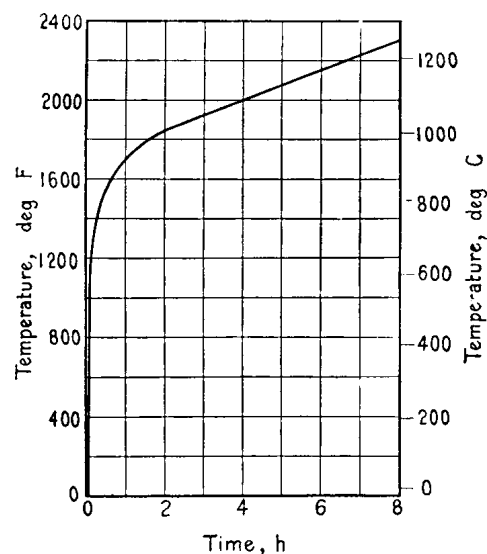
FIG. 1 Time-Temperature Curve
