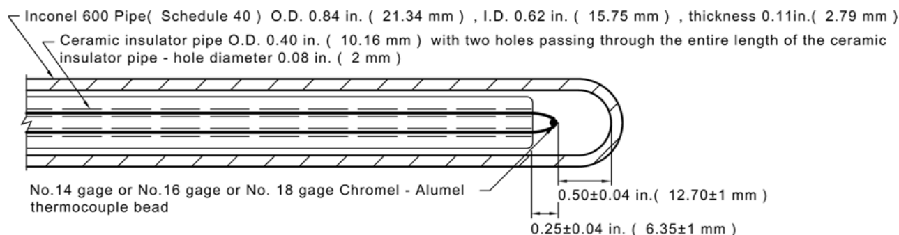
FIG. 2 Thermocouple Assembly
