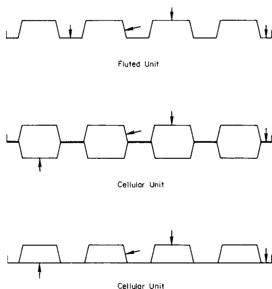
FIG. 3 Typical Location of Thermocouples
