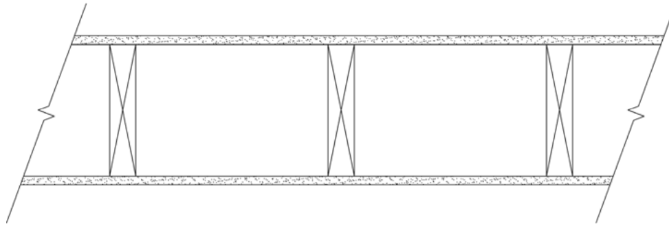
FIG. X7.3 Wood Wall and Floor Specimen
