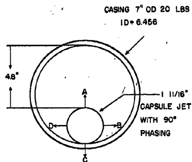
Fig. 2 - Capsule Jet Laying Against Side of Casing
