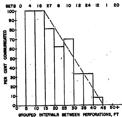
Fig. 5 - Communication Between Sets of Perforations At Various Spacings
