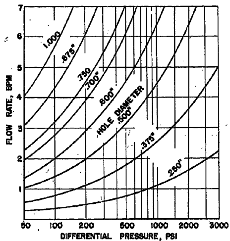
Fig. 1 - Pressure Drop Through Perforations
