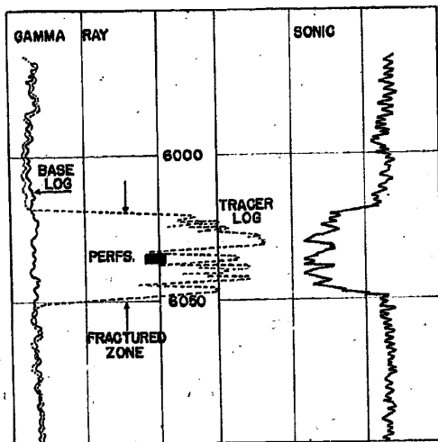
Fig. 7 - Gamma Ray - Sonic Log With Tracer Log Obtained After Fracturing With Radioactive Sand
