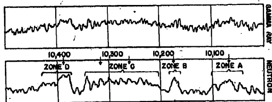
Fig. 6 - Selection of Entry Points From A Gamma Ray-Neutron Log
