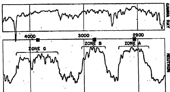
Fig. 9 - Gamma Ray-Neutron Log For Example Problem
