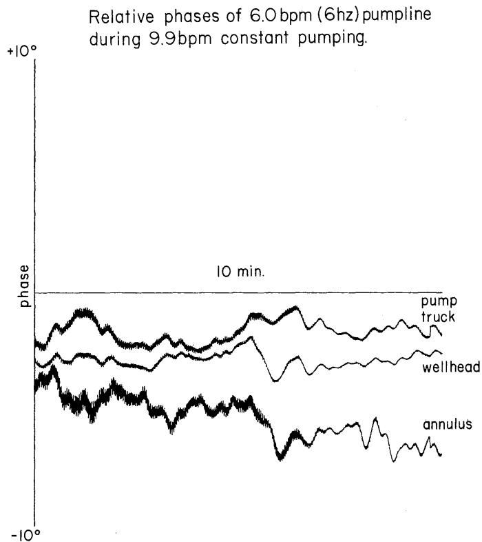
Fig. 7—Phase changes of 6-Hz pumpline during 10 minutes of proppant injection, Mounds well.
