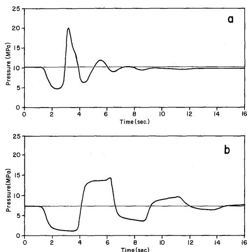
Fig. 1—Free oscillations in 1,589-m deep perforated well: (a) pre-fracture and post-fracture.
