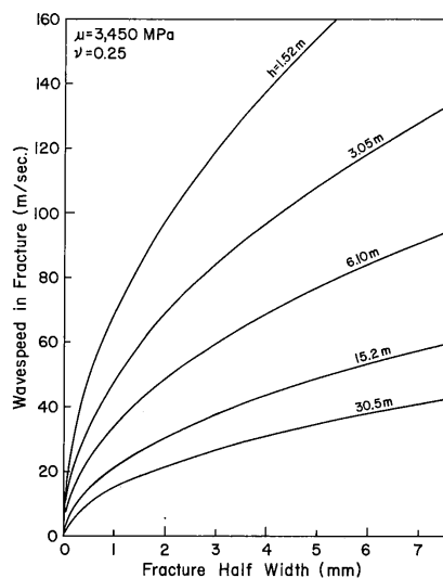
Fig. 12—Wavespeed in fracture for different radii h .
