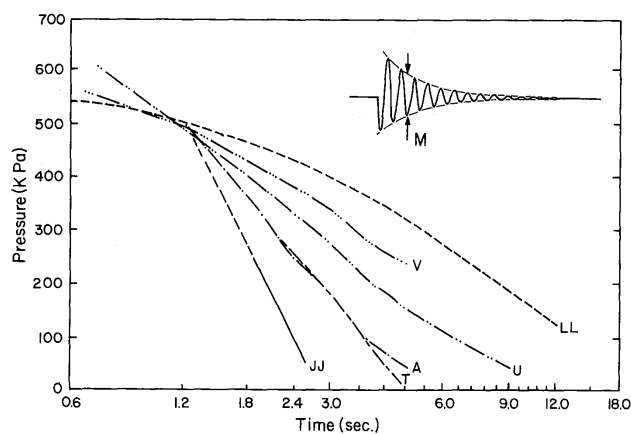
Fig. 4—Decay envelopes for free oscillations in Mounds well following different volumes of water injection in liters: JJ = less than 800, A = 800, T = 1,600, U = 2,400, V = 3,350, and LL = 47,700.
