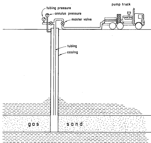
Fig. 5—Well completion and pressure measurement schematic for second Mounds test.
