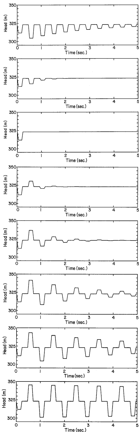
Fig. 10—Theoretical decay of free oscillations in frictionless well for which Z_c = 11,250 \text{ sec/m}^2 . From top to bottom, R_1 = 112,500, 22,500, 11,250, 5,725, 2,812, 1,125, 562 and 56 \text{ sec/m}^2 .
