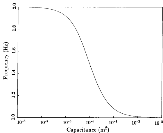
Fig. 11—Frequency of free oscillations vs. fracture capacitance for T_d = 0.5 \text{ sec} .
