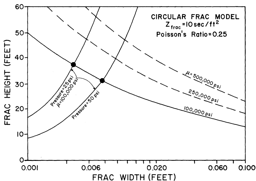
Fig. 14—Fracture height vs. width predicted by impedance method (lines with negative slope) and by static inflation (lines with positive slope). Characteristic impedance of fracture is 108 \text{ sec/m}^2 ( 10 \text{ sec/ft}^2 ).
