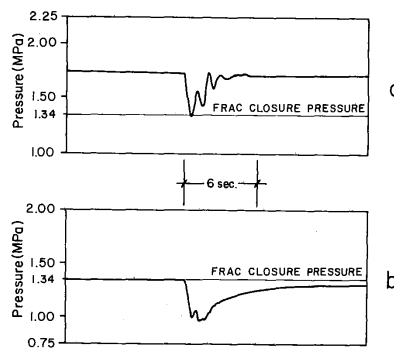
Fig. 2—Free oscillations in Mounds well: (a) above fracture closure pressure and (b) at fracture closure pressure.
