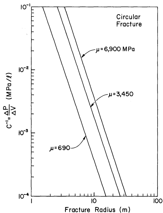
Fig. 9—Inverse of fracture capacitance (in units of pressure change per volume change) vs. radius for different rock shear moduli.
