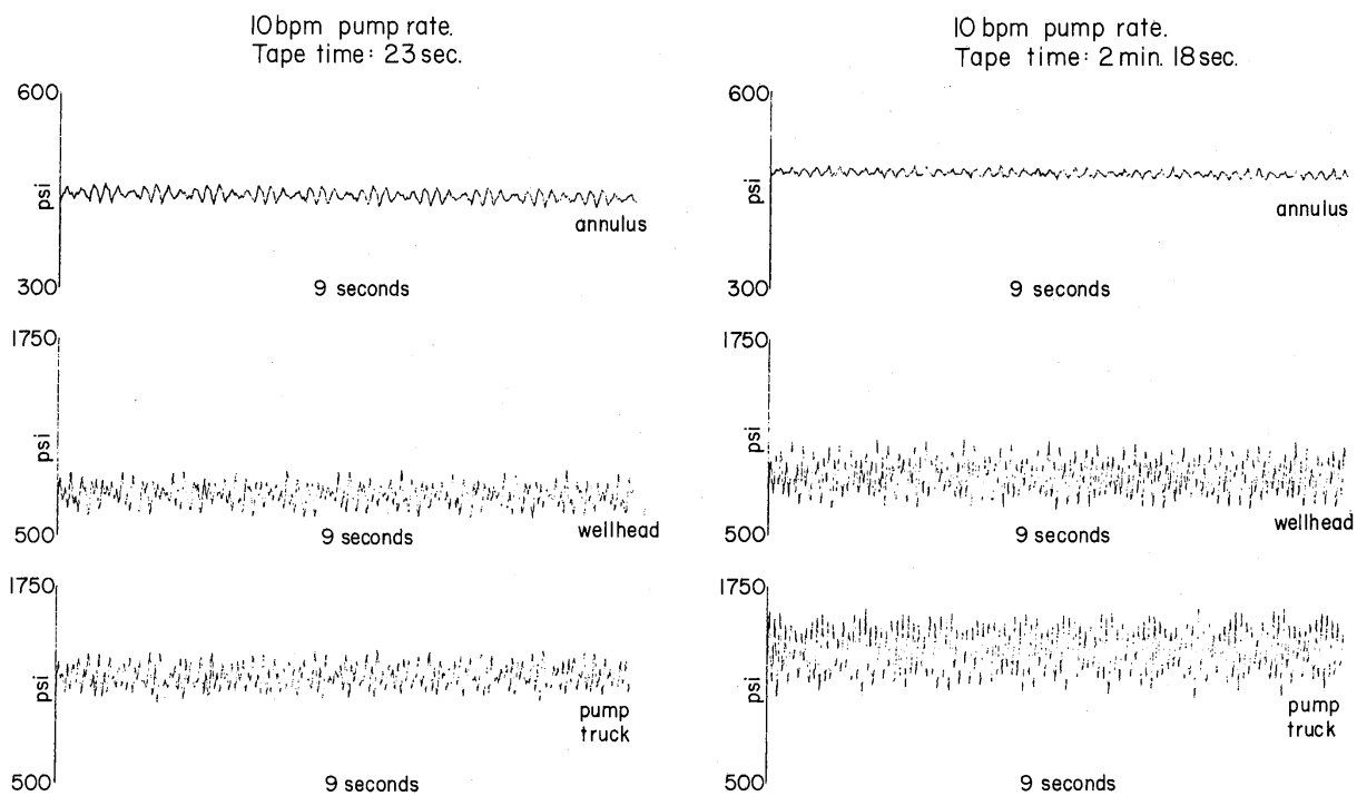
Fig. 6—Forced oscillations of pressure at constant pump rate: (a) at beginning of proppant injection and (b) 2 minutes later.
