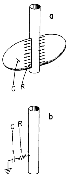
Fig. 8—(a) Hydraulic model of well and fracture and (b) electrical analog.
