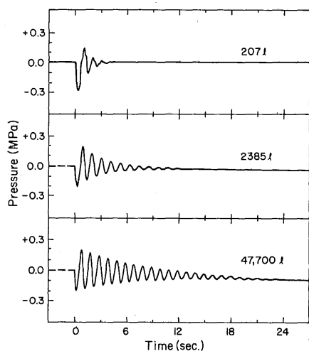
Fig. 3—Free oscillations in Mounds well after injection of 207, 2,385, and 47,700 liters of water.
