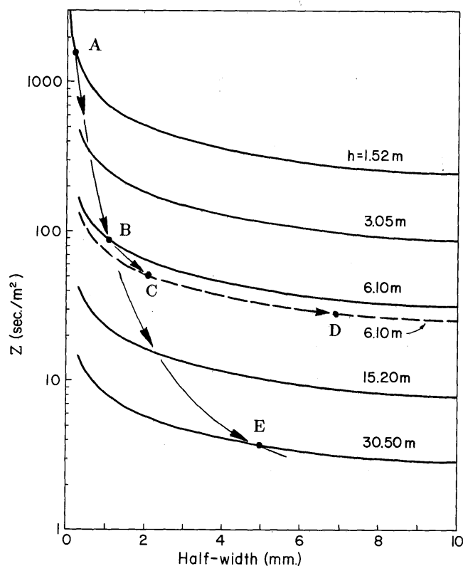
Fig. 13—Characteristic impedances of penny-shaped (solid lines) and plane strain (dashed line) fractures of different radii or height h .
