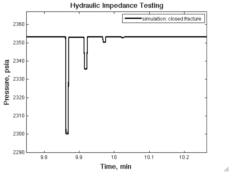
Figure 3.2: Simulated HIT for well with closed fracture.
