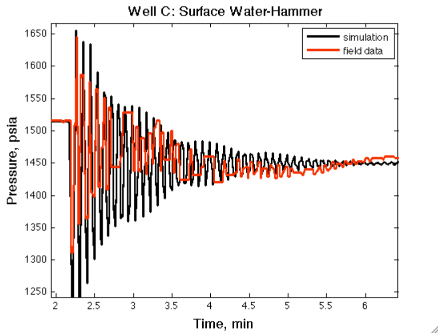
Figure 3.8: Detailed waveform comparison of water hammer in Well C.
