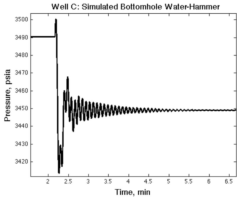
Figure 3.16: Simulated bottomhole water hammer for well C.
