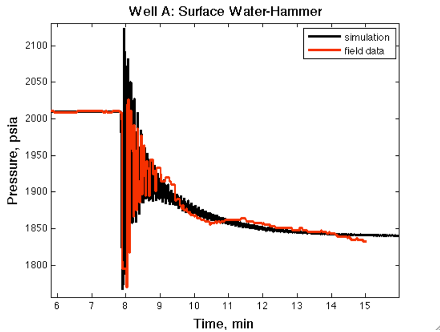
Figure 3.3: History matching overall surface water hammer in Well A.
