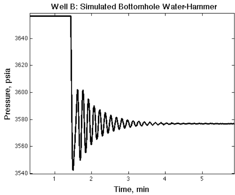
Figure 3.15: Simulated bottomhole water hammer for well B.
