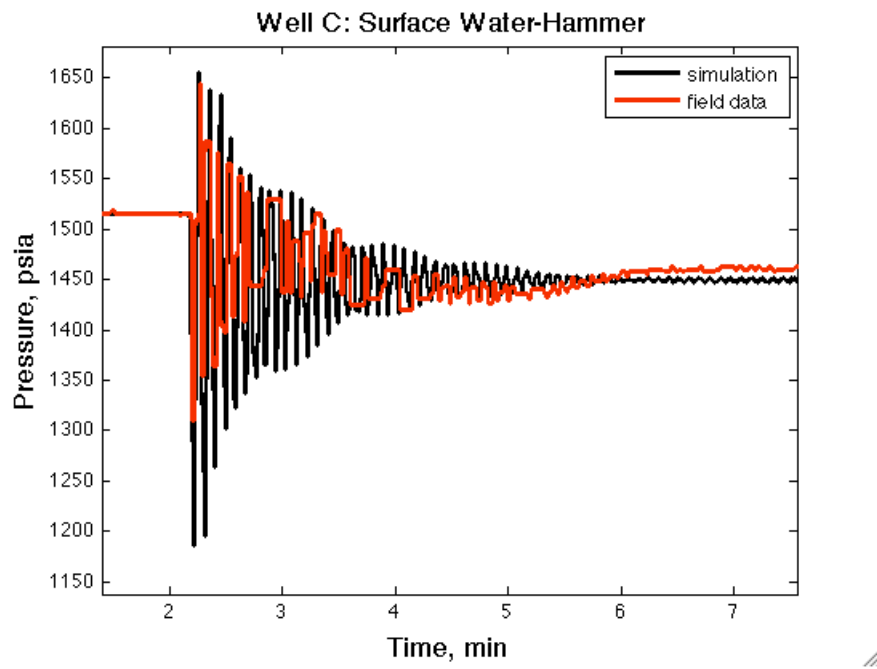
Figure 3.7: History matching overall surface water hammer in Well C.
