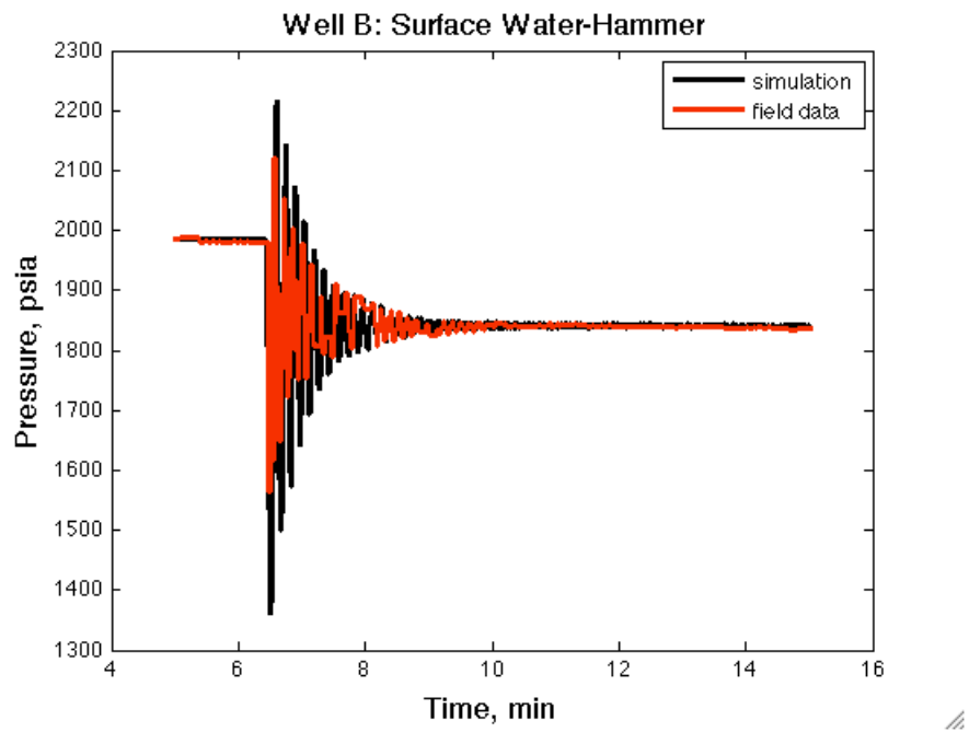
Figure 3.5: History matching overall surface water hammer in Well B.
