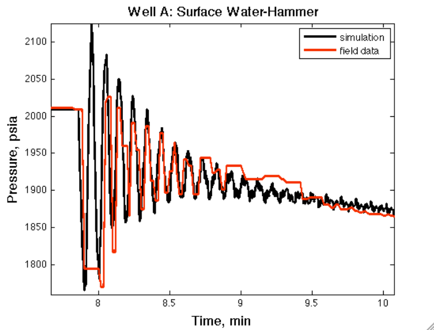
Figure 3.4: Detailed waveform comparison of water hammer in Well A.
