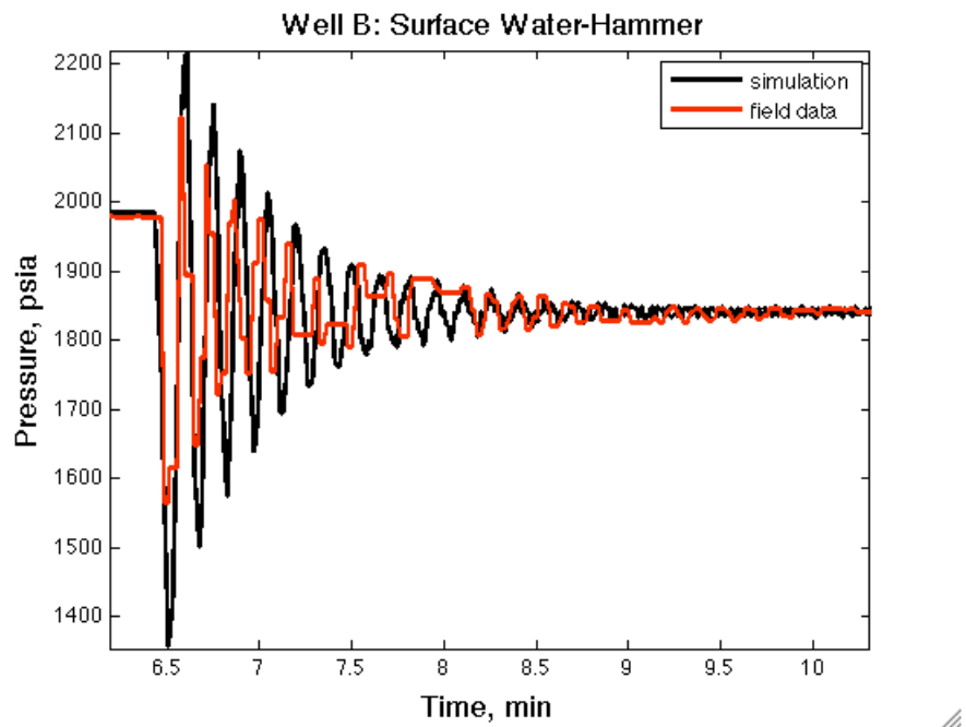
Figure 3.6: Detailed waveform comparison of water hammer in Well B.
