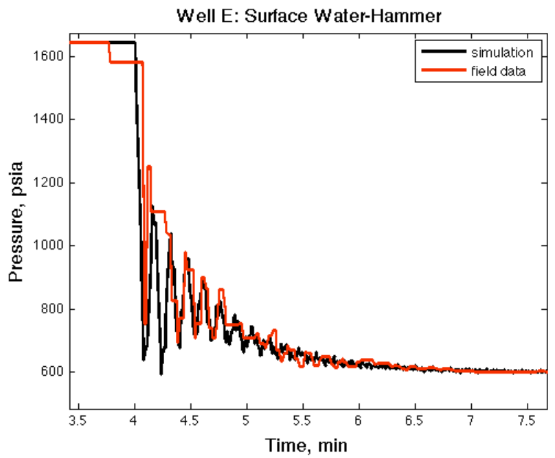
Figure 3.12: Detailed waveform comparison of water hammer in Well E.
