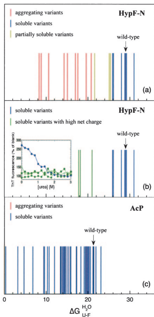
FIG. 4. a , conformational stabilities of wild-type HypF-N and 18 variants, each with a single mutation (reported in Table I). Blue, gold, and red bars indicate mutants that were found to be completely soluble, partially aggregated, or fully aggregated after expression in vivo , respectively. b , conformational stabilities for wild-type and all soluble single variants (blue bars) and three multiple mutants that were soluble despite their relatively low stability (green bars). The latter are a quadruple mutant containing the E55K/V59R/E77R/E87K substitutions ( \Delta G_{U-F}^{H_2O} = 21 \pm 3 \text{ kJ mol}^{-1} ) and two quintuple mutants with the additional T5R or Q32K mutations, respectively (both of which have \Delta G_{U-F}^{H_2O} = 18 \pm 3 \text{ kJ mol}^{-1} ). The inset shows the ThT fluorescence present after incubation for 30 min under denaturing conditions (30% trifluoroethanol) as a function of the urea concentration for the wild-type protein (blue circles) and for the quadruple mutant (green circles) and quintuple mutants (green triangles and squares) HypF-N. c , conformational stabilities for wild-type AcP and 42 variants, each with a single mutation. The mutants illustrated in the figure and their conformational stabilities have been described previously (23, 41). Blue bars indicate soluble mutants that could be purified. In all three panels \Delta G_{U-F}^{H_2O} errors (corresponding to the standard deviation) are 3.0 and 3.4 \text{kJ mol}^{-1} for soluble and aggregated variants, respectively.
