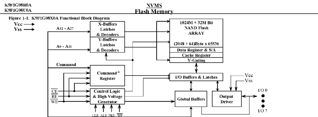
Figure 2-1. K9F1G08X0A (X8) Organization
