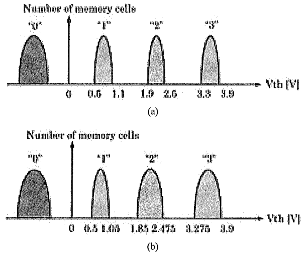
Fig. 7. Threshold voltage distribution of a four-level NAND cell. (a) Conventional. (b) Proposed.
