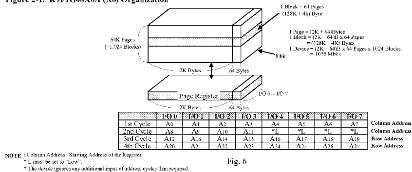
Figure 2-1. K9F1G08X0A (X8) Organization
