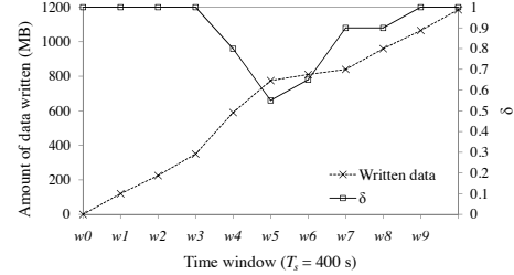
Figure 14: The changes in the size of written data and the \delta value
