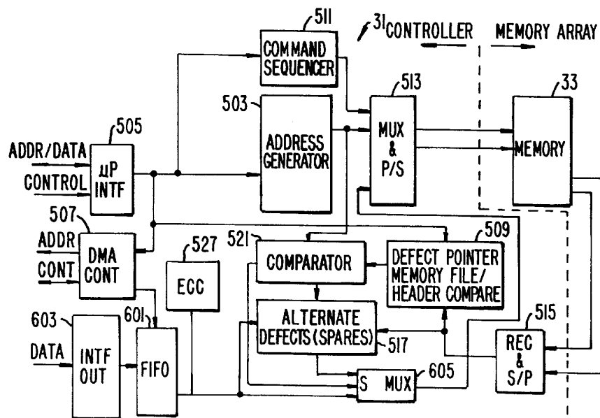
WRITE DATA PATH CONTROL
