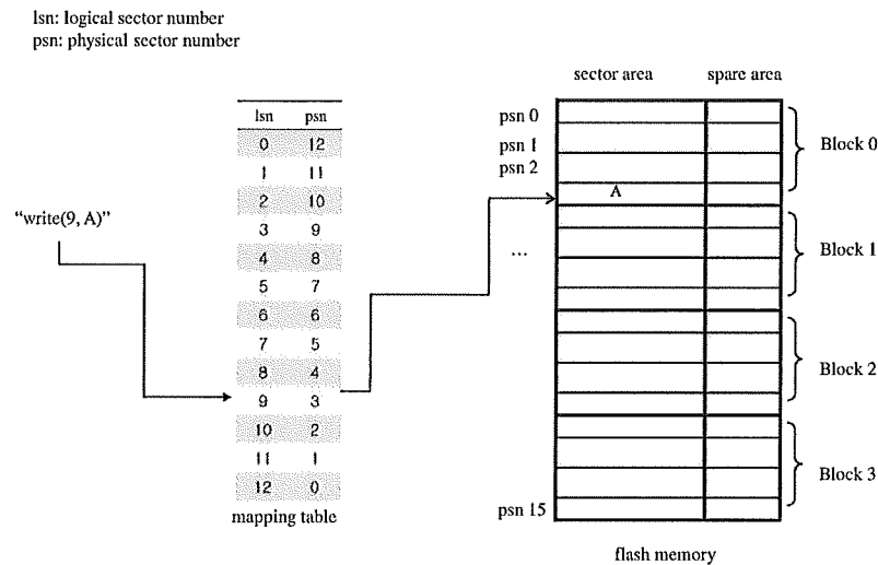
Fig. 2. Sector mapping.
