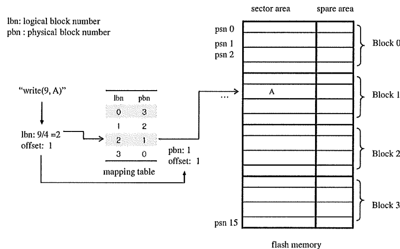
Fig. 3. Block mapping.
