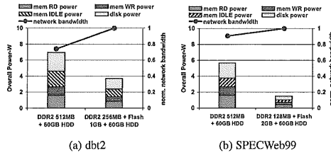
Figure 9. Breakdown in system memory and disk power and network bandwidth for architecture with/without a Flash based disk cache.
