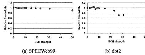
Figure 10. Average throughput as a function of ECC strength. The system used 256MB of DRAM and 1GB of Flash.
