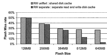
Figure 4. A miss rate comparison executing a dbt2 (OLTP) disk trace for a unified Flash based disk cache and a split read and write Flash based disk cache.
